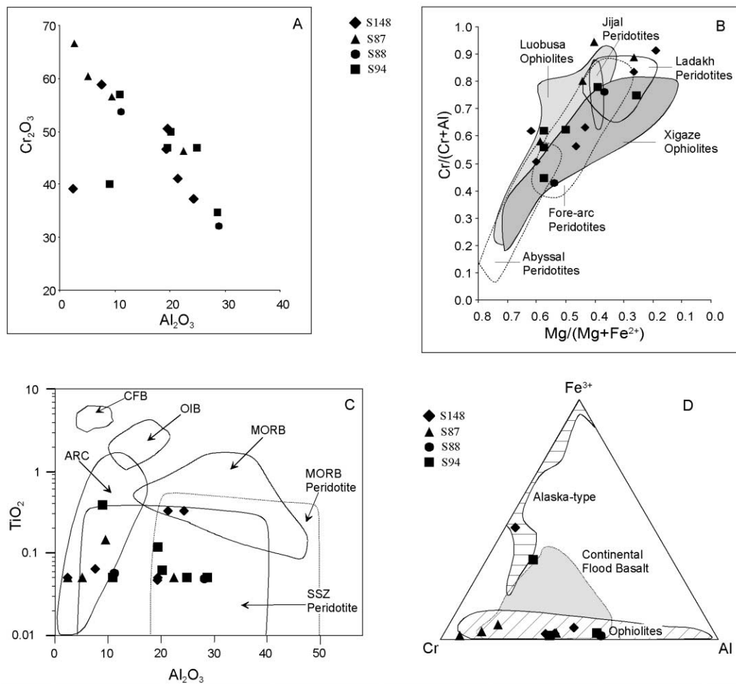
Figure 9. Geochemical plots of Cr-rich spinels from the Youxia and Shenkeza sandstones. A, \text{Cr}_2\text{O}_3 versus \text{Al}_2\text{O}_3 . B, Cr number ( \text{Cr}/(\text{Cr} + \text{Al}) ) versus Mg number ( \text{Mg}/(\text{Mg} + \text{Fe}^{2+}) ). Fields displayed are abyssal peridotites from Bryndzia and Wood (1990), fore-arc peridotites from Parkinson and Pearce (1998), Jijal peridotites and Ladakh peridotites from Rolland et al. (2002), Luobusa ophiolites from Zhou et al. (1996), and Xigaze ophiolites from Wang et al. (2000). C, \text{TiO}_2 versus \text{Al}_2\text{O}_3 . Fields displayed are from Kamenetsky et al. (2001): CFB = continental flood basalt, OIB = oceanic island basalt, MORB = mid-ocean ridge basalt, ARC = volcanic island arc, SSZ = suprasubduction zone. D, Cr-Al- \text{Fe}^{3+} ternary plot (12 points with valid \text{Fe}^{3+} shown). Fields displayed are from Cookenboo et al. (1997).
