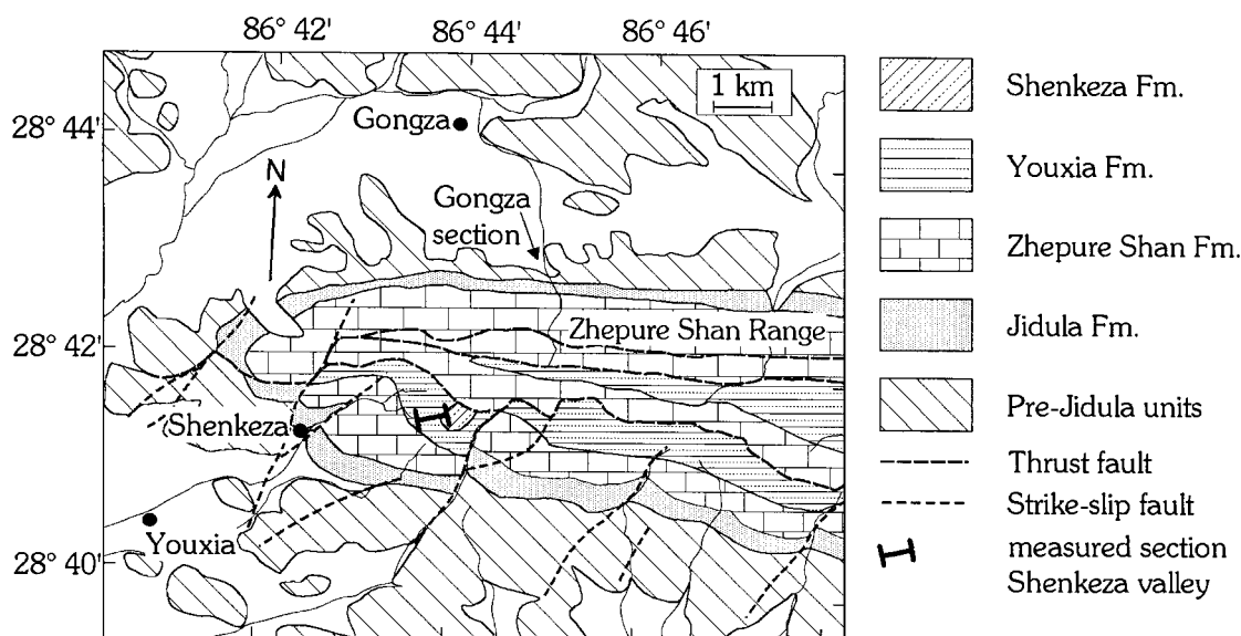
Figure 2. Simplified geologic map showing the location of the studied sections on the western end of the Zhepure Shan range. Interpretation extended from outcrop observations using Landsat TM image.
