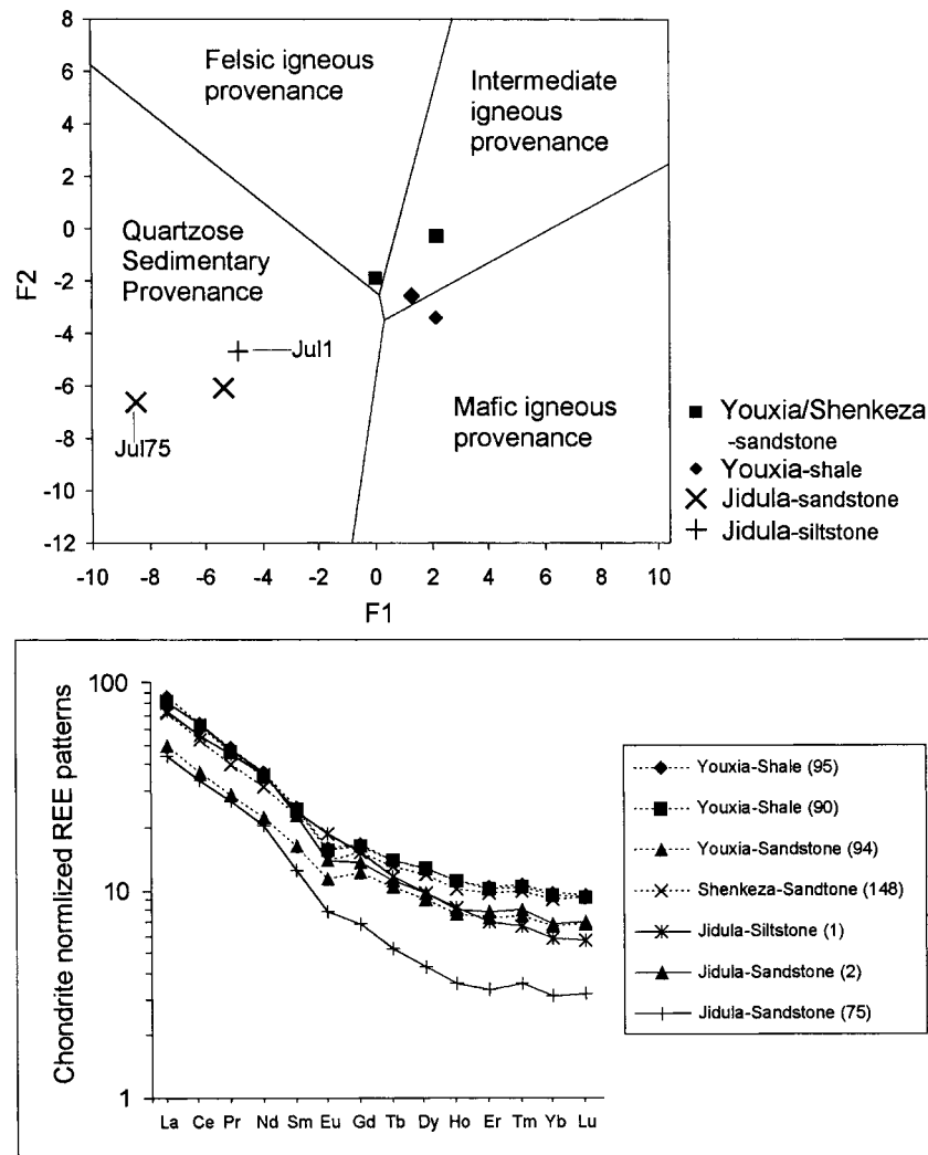
Figure 7. Geochemical plots of the lower Tertiary clastics in the Tingri region. Top , Provenience discrimination diagram. Tectonic setting fields are from Roser and Korsch (1988). Jul 1 and Jul 75 are recalculated to 100% CaO and are volatile free because of significantly high calcite contents. Bottom , Chondrite-normalized rare earth element patterns; chondritic values are those of Taylor and McLennan (1985).
