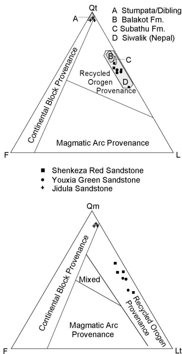
Figure 4. Detrital mode plot of lower Tertiary sandstones in the Tingri region. Tectonic fields are from Dickinson (1985). Fields shown of other related Himalayan sandstones are from Garzanti et al. (1996).
