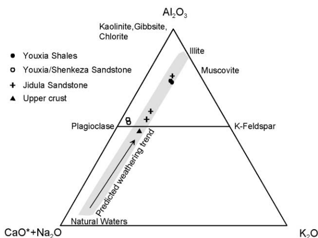
Figure 5. Chemical index of alteration ternary plot of lower Tertiary clastics in the Tingri region. Modified after Bock et al. (1998). The enrichment in \text{Al}_2\text{O}_3 and depletion of \text{CaO}^* + \text{Na}_2\text{O} + \text{K}_2\text{O} on this plot reflects the degree of chemical weathering to which the materials have been subjected. Three analyses of the Jidula Formation define a linear trend encompassed in the predicted weathering trend for the average upper crustal composition, while those of the Youxia Formation do not follow the predicted weathering trend, indicating processes in addition to the weathering have affected the Youxia sediments.
