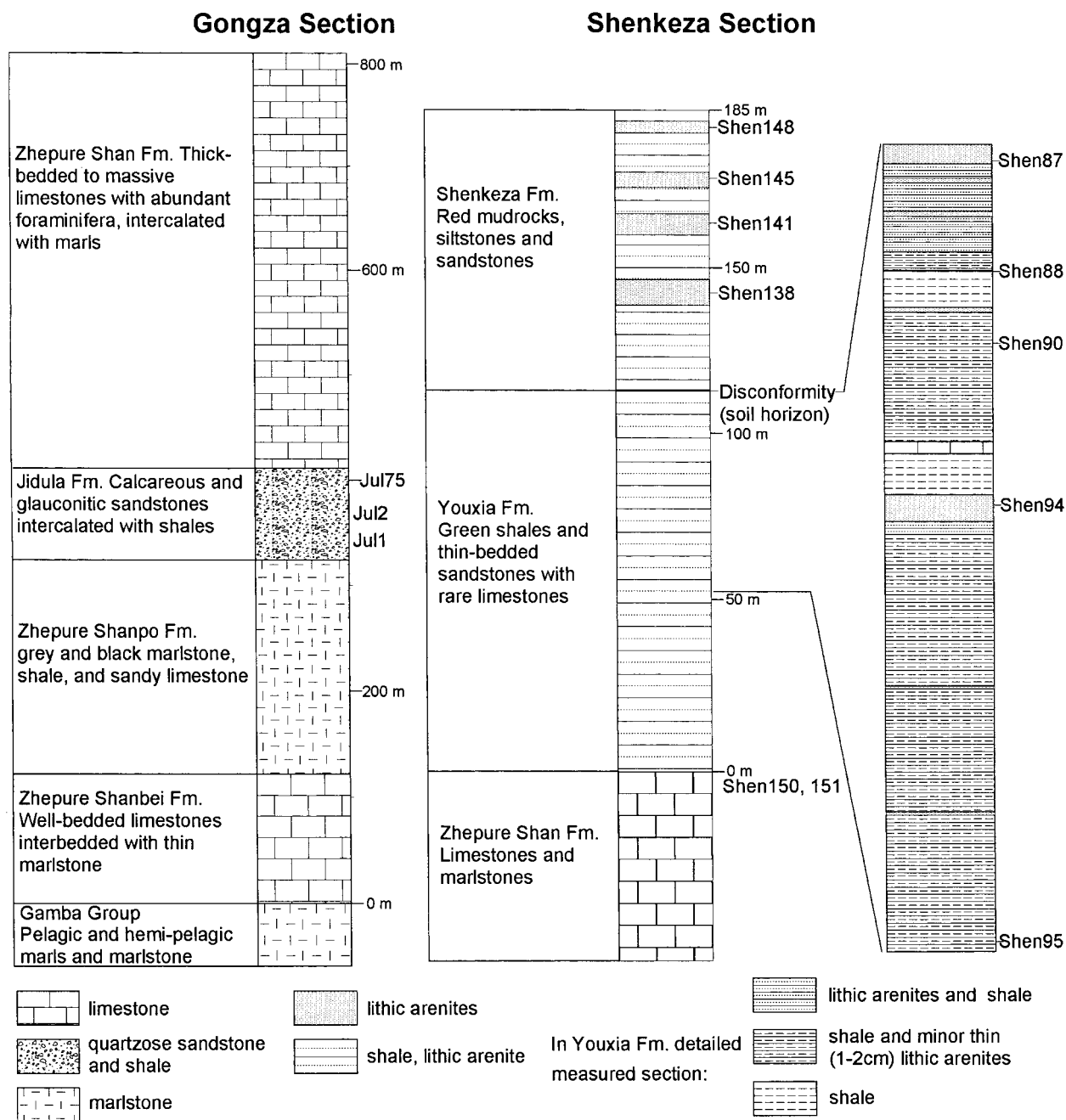
Figure 3. Stratigraphic columns of lower Tertiary sequence in the Tingri region. The Shenkeza section was measured by us in 2000; the Gongza section is from Willems et al. (1996). Section locations are shown in figure 2. Sample positions are indicated by “Shen” plus a number in the Shenkeza section and “Jul” plus a number in the Gongza section.
