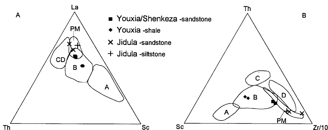
Figure 8. Tectonic discrimination plots from Bhatia and Crook (1986). A , La-Th-Sc ternary. B , Th-Sc-Zr/10 ternary. Fields: A = oceanic island arc, B = continental island arc, C = active continental margin, D = passive margin, PM = passive margin field from McLennan et al. (1990).
