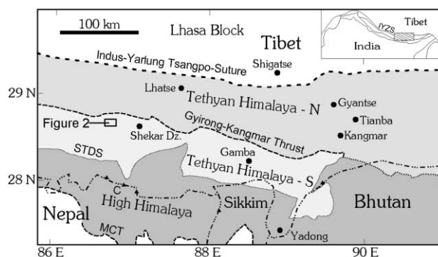
Figure 1. Simplified tectonic map of the east-central Tethyan Himalaya (modified after Willems et al. 1996). The inset map shows the position of this area in the Himalayan system. MCT = Main Central Thrust; STDS = Southern Tibet Detachment system; C = Cholmolungma.
