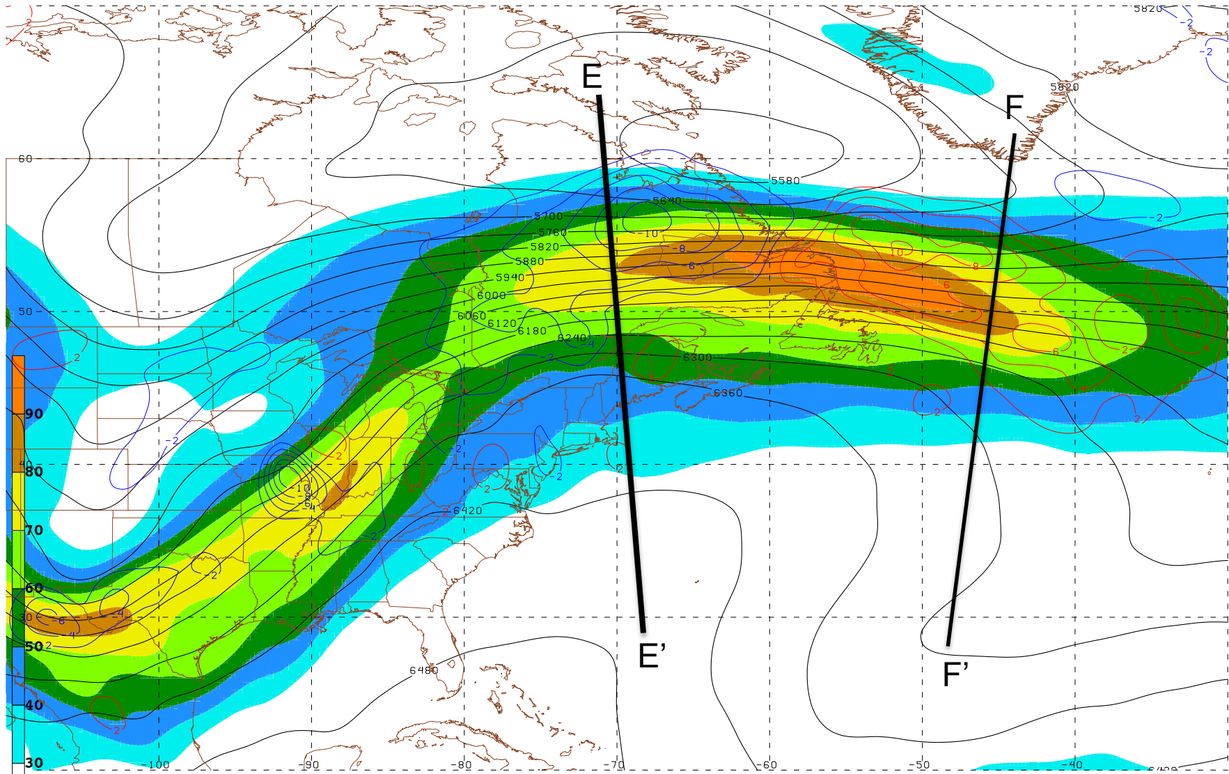
250mb geo. jet, 300-700mb thck, 400mb geo. temp. adv. 131222/1200V012
