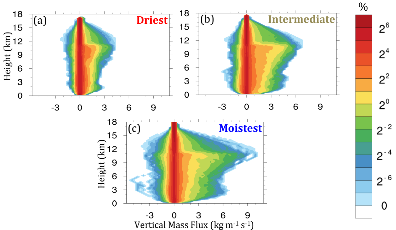
Figure 1: Contoured frequency by altitude diagrams of vertical mass flux averaged 24 hours before the spinup time for a moist entropy deficit of (a) 100 \text{ J kg}^{-1} \text{ K}^{-1} , (b) 30 \text{ J kg}^{-1} \text{ K}^{-1} , and (c) 0 \text{ J kg}^{-1} \text{ K}^{-1} .
