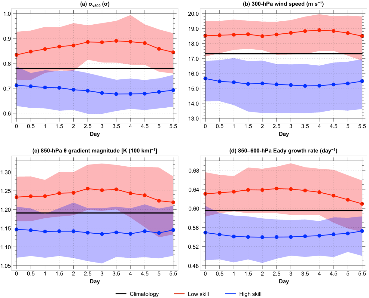
Fig. 2.3. Distributions of (a) area-averaged \sigma_{v500} ( \sigma ), (b) area-averaged 300-hPa wind speed ( m s^{-1} ), (c) area-averaged 850-hPa \theta gradient magnitude [ K (100 km)^{-1} ], and (d) area-averaged 850–600-hPa Eady growth rate ( day^{-1} ) over the Arctic at days 0–5.5, every 0.5 days, for low-skill forecasts (red) and high-skill forecasts (blue), with solid lines indicating the mean values and shading indicating the IQR. Black lines indicate the mean values of the quantities across all times during the 2007–2017 climatology. Dots indicate statistical significance at the 95% confidence level of the mean values of the quantities for low-skill forecasts (red) and high-skill forecasts (blue) with respect to climatology.
