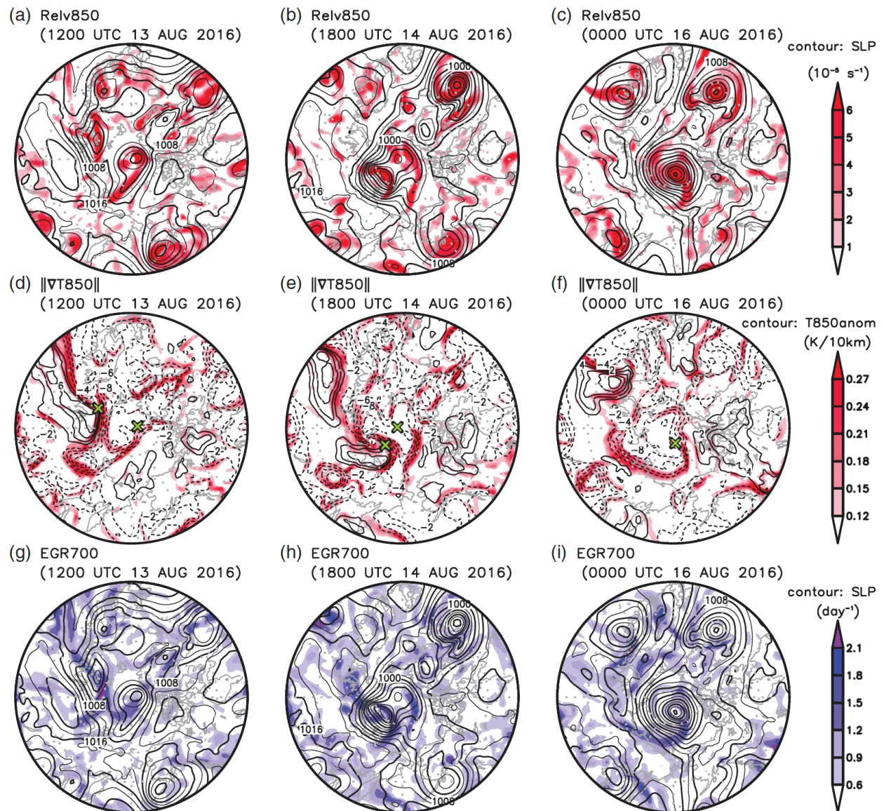
Fig. 1.4. (a)–(c) Relative vorticity at 850 hPa ( 10^{-5} \text{ s}^{-1} , shading) and SLP (contours, every 3 hPa), (d)–(f) magnitude of the horizontal temperature gradient at 850 hPa [ \text{K} (10 \text{ km})^{-1} , shading] and temperature anomaly at 850 hPa (contours, every 2 K), and (g)–(i) Eady growth rate at 700 hPa ( \text{day}^{-1} , shading) and SLP (contours, every 3 hPa), at (a),(d),(g) 1200 UTC 13 August 2016, (b),(e),(h) 1800 UTC 14 August 2016, and (c),(f),(i) 0000 UTC 16 August 2016. Green crosses mark the locations of minimum central pressure of two cyclones (d),(e) that merge into one cyclone (f). [Figure 3 and adapted caption from Yamagami et al. (2017).]
