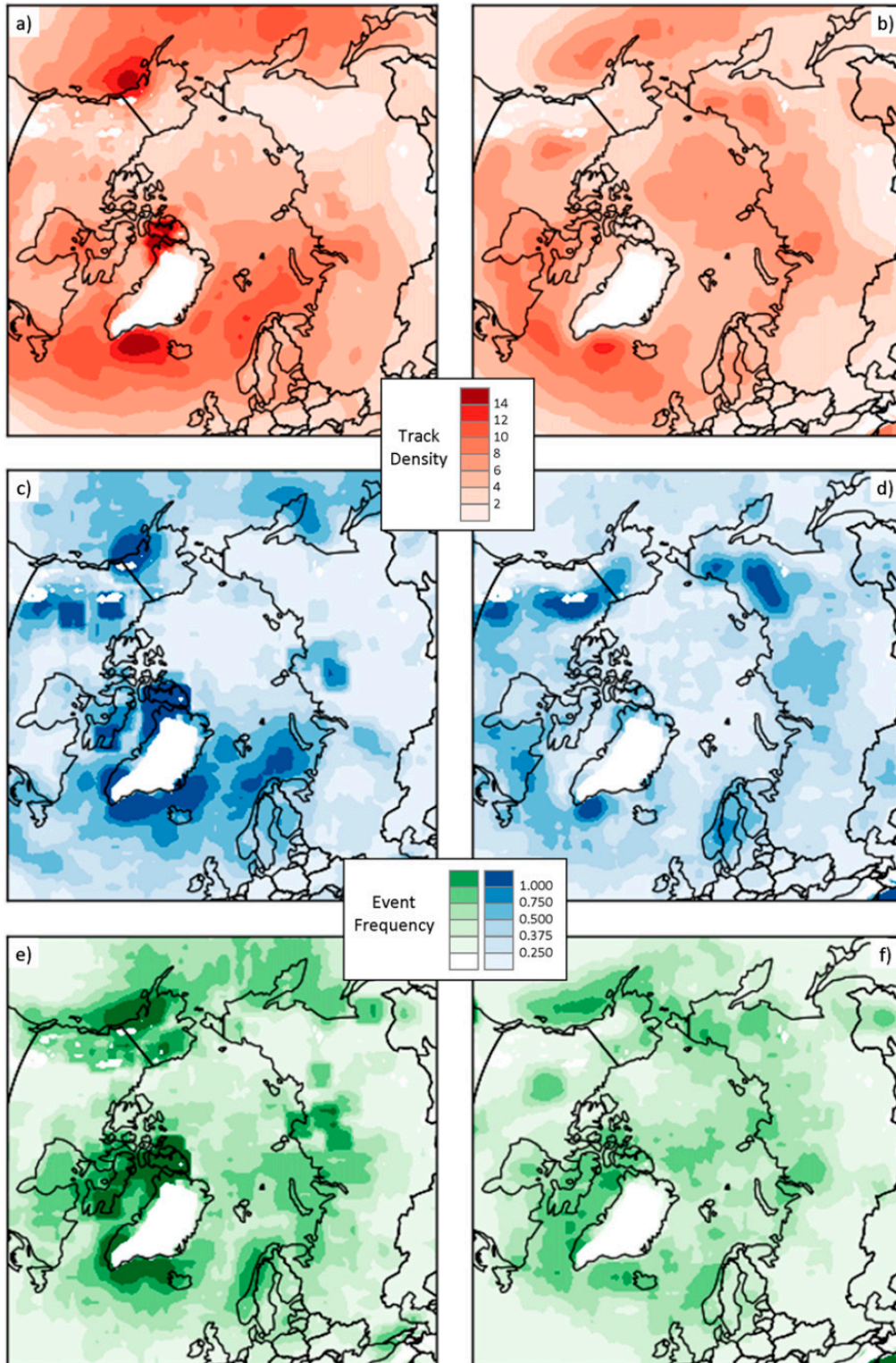
Fig. 1.3. Frequency of (a),(b) cyclone tracks, (c),(d) cyclogenesis events, and (e),(f) cyclolysis events for (a),(c),(e) winter (DJF) and (b),(d),(f) summer (JJA), averaged for the period 1979–2014. Units are the number of tracks or events per 500 km 2 area per month. [Figure 3 and caption from Crawford and Serreze (2016).]
