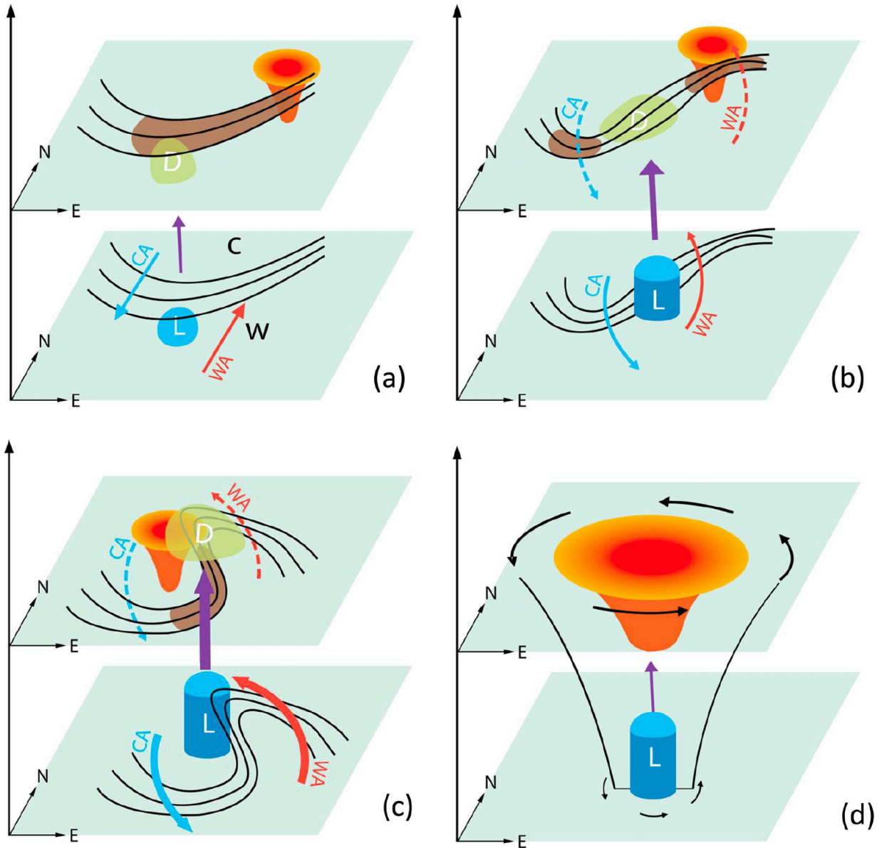
Fig. 1.5. Sketch of the development of AC12 for the (a) “incipient stage,” (b) “early development stage,” (c) “drastic intensification period,” and (d) “lingering stage.” Isotherms are indicated by black contours, jet streaks are indicated by brown shading, upper-tropospheric divergence (“D”) is indicated by green shading, a TPV and associated stratospheric warm temperature anomaly is indicated by orange-red inverted cone, storm center (“L”) is indicated by blue column, cold and warm temperature advections (“CA” and “WA”, respectively) and associated directions in which cold and warm air are advected are indicated by blue and red arrows (arrows are dashed for upper troposphere and are solid for surface), respectively, upward motion is indicated by purple arrow, and cyclonic circulations around the storm center are indicated by black arrows. Labels “C” and “W” represent cold and warm air masses, respectively. Relative thickness of arrows corresponds to relative strength of quantities indicated by arrows. [Figure 4 and adapted caption from Tao et al. (2017b).]
