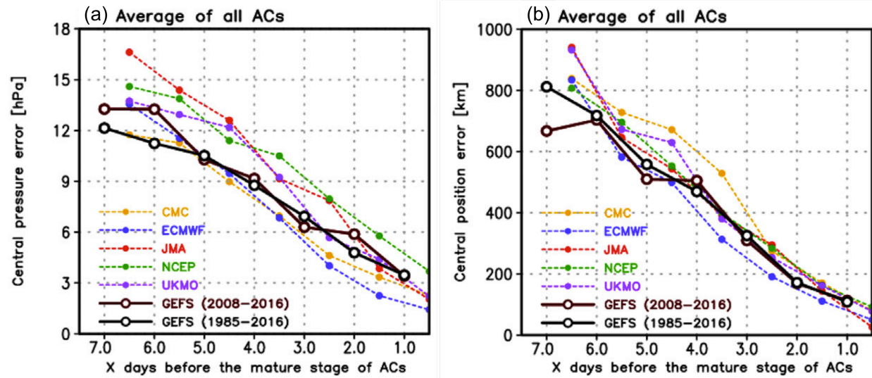
Fig. 1.6. (a) Average central pressure error (hPa) during the mature stage (i.e., time of peak intensity of AC) of 26 extraordinary ACs in summer during 1985–2016 (black) and 10 extraordinary ACs in summer during 2008–2016 (brown) from the GEFS reforecast dataset version 2, as a function of forecast lead time. Colored broken lines are the average central pressure errors for the 10 extraordinary ACs, predicted by CMC (yellow), ECMWF (blue), JMA (red), NCEP (green), and UKMO (purple). (b) As in (a), but for average central position error (km). [Figures 4a and 5a and captions adapted from Yamagami et al. (2019).]
