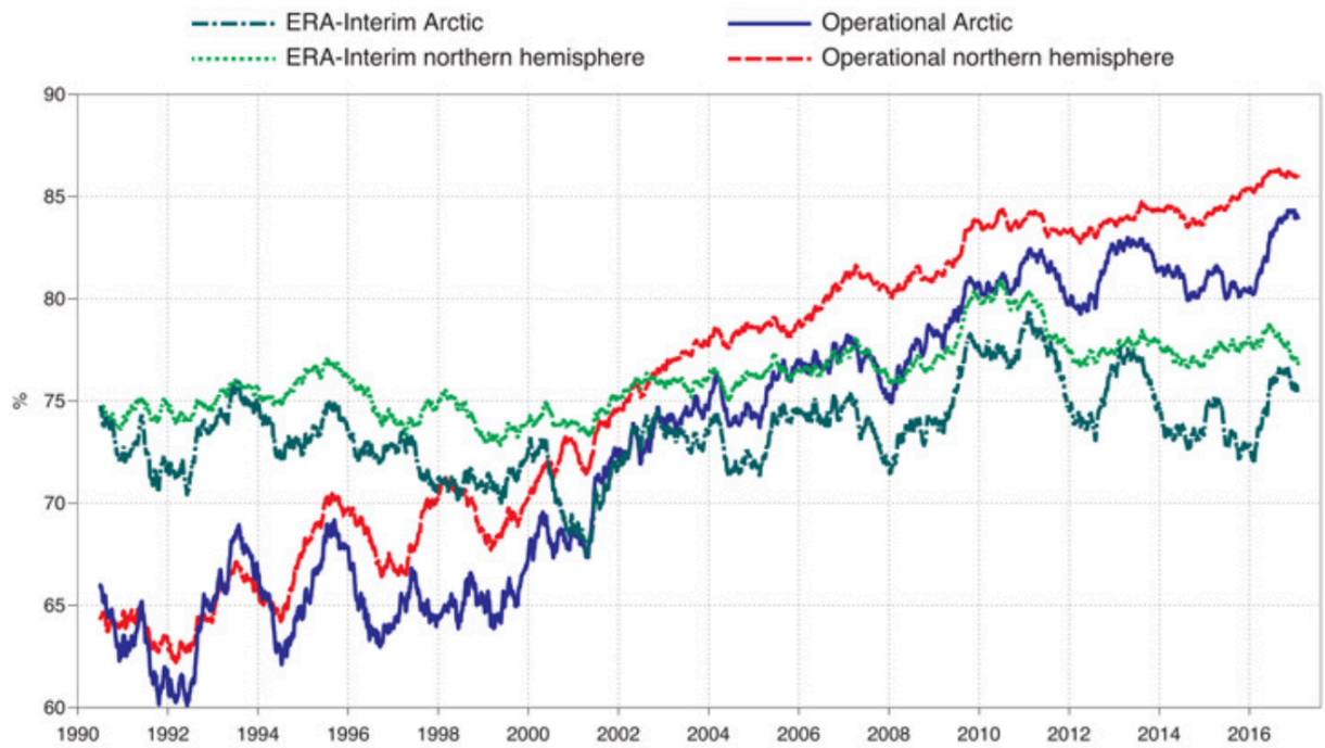
Fig. 1.1. Evolution of the anomaly correlation of 500-hPa geopotential height at forecast day 6 for the Northern Hemisphere and for the Arctic (60–90°N) in the ECMWF operational system and ERA-Interim reanalysis. [Figure 2 and adapted caption from Sandu and Bauer (2018).]
