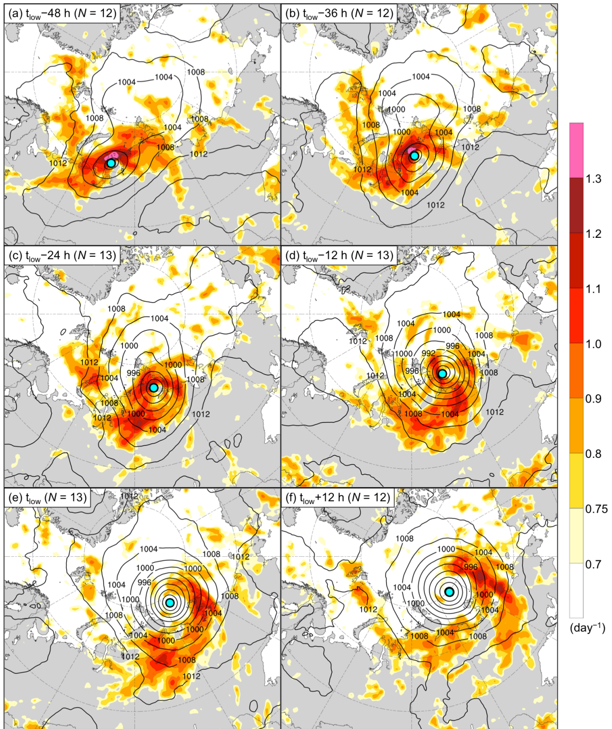
Fig. 3.3. AC-centered composites for the strong low-skill ACs of 850–600-hPa Eady growth rate ( \text{day}^{-1} ; shading) and SLP (hPa; black contours) at (a) t_{low} - 48 h, (b) t_{low} - 36 h, (c) t_{low} - 24 h, (d) t_{low} - 12 h, (e) t_{low} , and (f) t_{low} + 12 h. The cyan dot shows the location of the composite AC.
