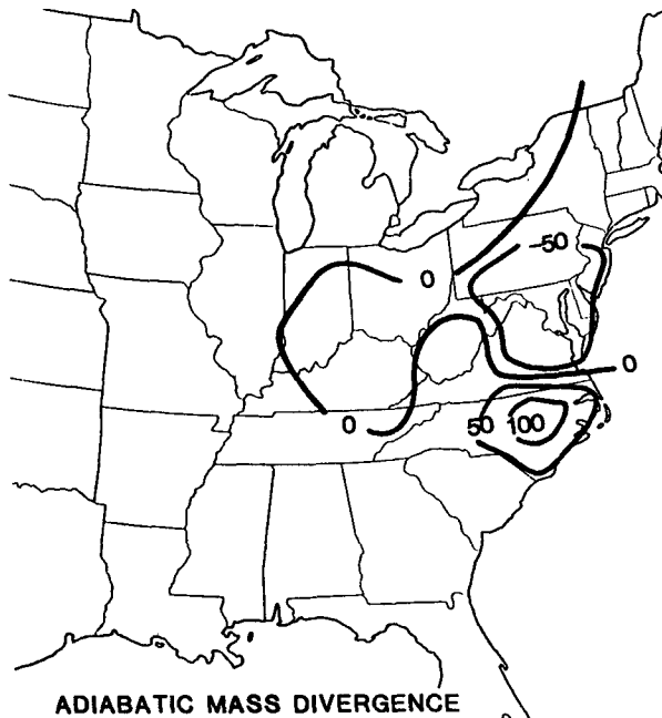
FIG. 16. Adiabatic mass divergence for the 292 K surface at 1200 GMT 19 February 1979 ( 50 = 50 \times 10^{-6} \text{ mb K}^{-1} \text{ s}^{-1} ).
