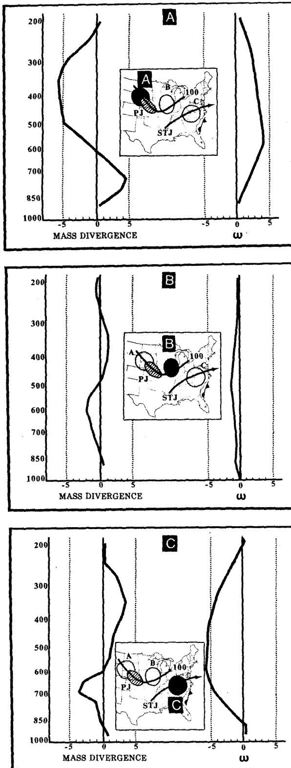
FIG. 6. Areal-averaged profiles of the adiabatic mass divergence ( S = 5 \times 10^{-5} \text{ mb K}^{-1} \text{ s}^{-1} ) and vertical motion ( \mu\text{b s}^{-1} ) for 1200 GMT 18 February 1979 (the vertical coordinate is \ln p ). The profiles are computed for the lettered areas shaded in the map inserts for each set in (a), (b) and (c). The map inserts contain the position of
