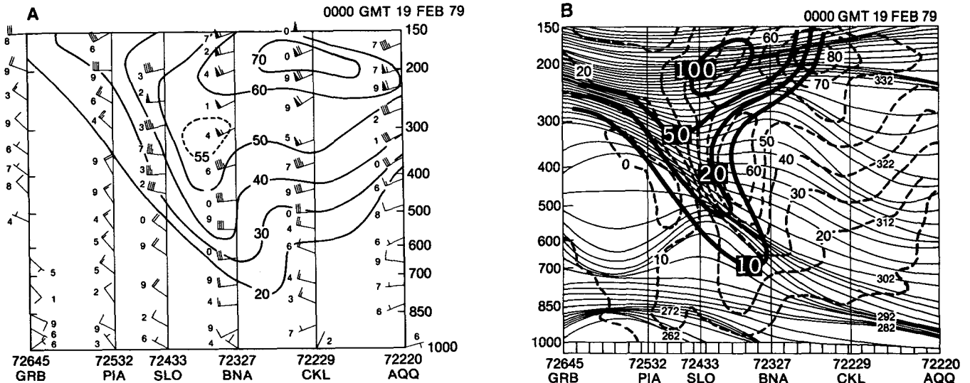
FIG. 10. As in Fig. 9 except from Green Bay, Wisconsin (GRB) to Apalachicola, Florida (AQQ) for 0000 GMT 19 February 1979.
