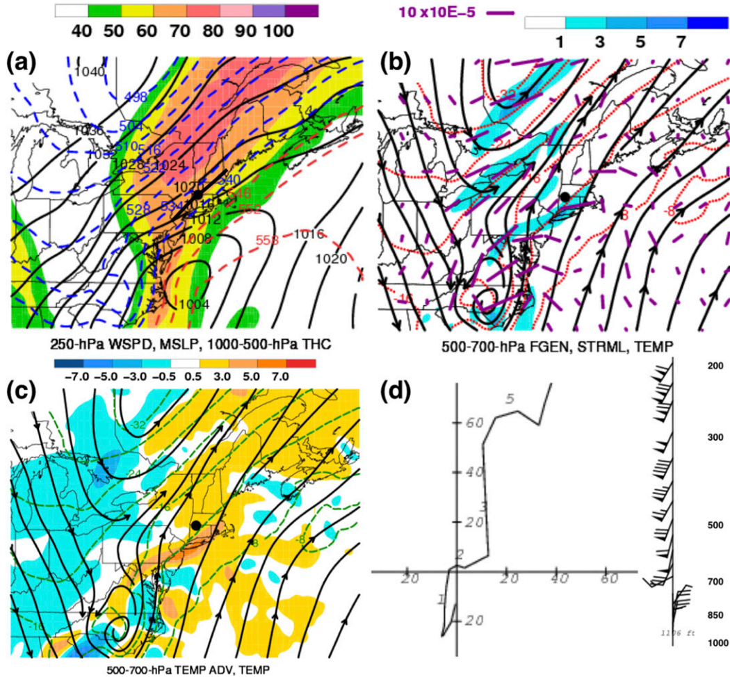
FIG. 13. As in Fig. 11, except for the laterally quasi-stationary snowband at 0600 UTC 2 Mar 2009. In (a), the black line segment represents the position of the band axis and corresponds to the dash-dot pattern in Fig. 3c.
