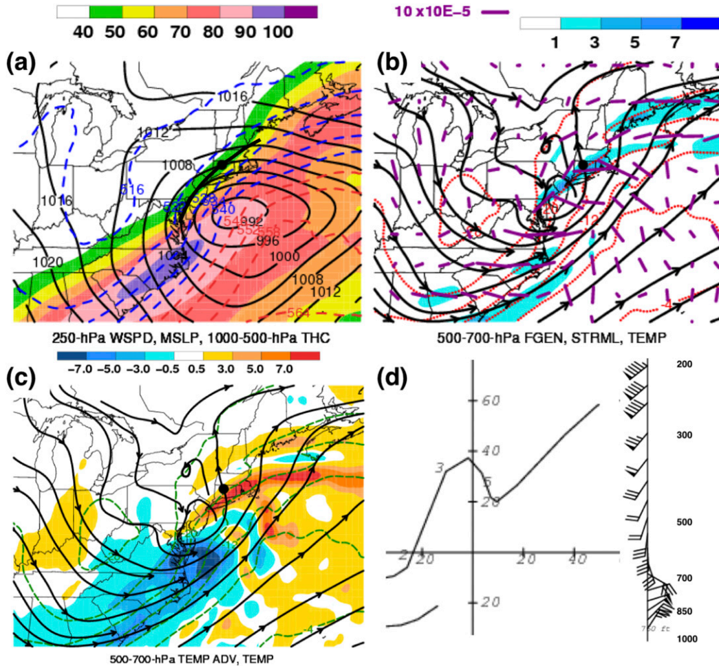
FIG. 15. As in Fig. 11, except for the pivoting snowband at 1200 UTC 12 Feb 2006. In (a), the black line segment represents the position of the band axis and corresponds to the dash-dot pattern in Fig. 3d. In (a)–(c), the heavy black dot marks the PZ location.
