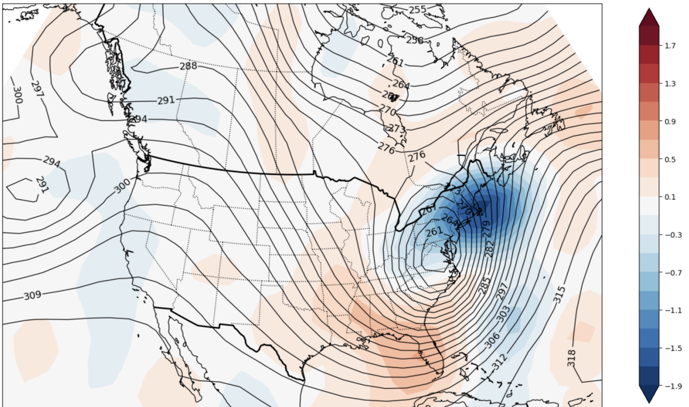
NCEP-NCAR 700-hPa height and omega Valid at: 1993-03-14-0000 UTC
