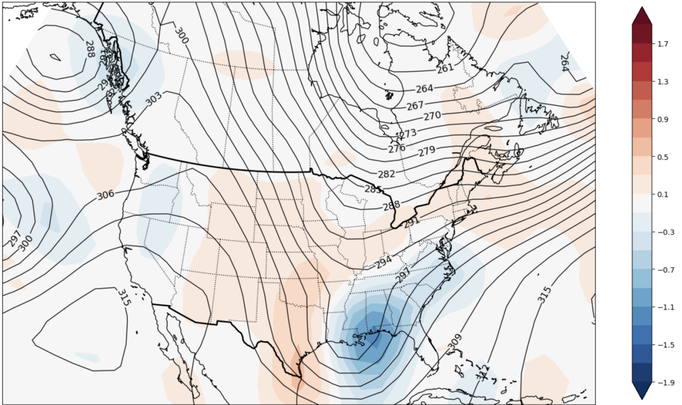
NCEP-NCAR 700-hPa height and omega Valid at: 1993-03-13-0000 UTC
