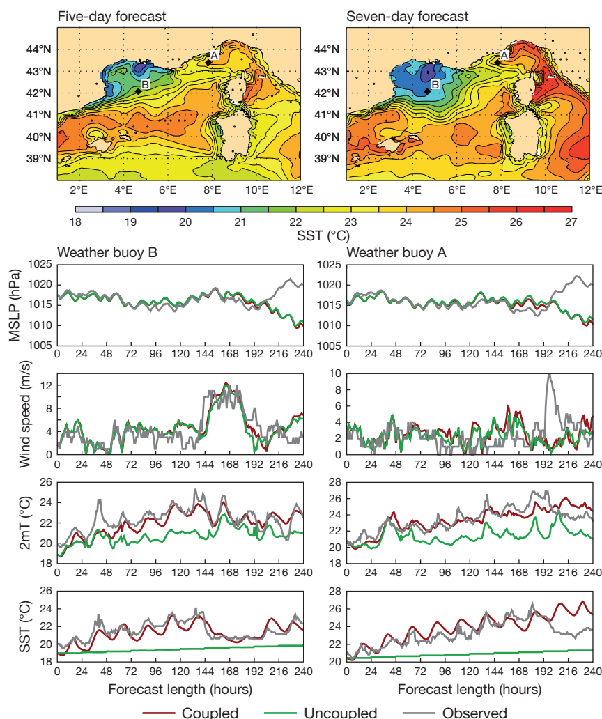
Mistral case. Predicted SST from experimental runs with ECMWF's coupled model starting from 00 UTC on 10 June 2017 valid at 00 UTC on 15 June (top left) and at 00 UTC on 17 June 2017 (top right). The other panels show the observed and predicted mean sea level pressure, wind speed, 2-metre temperature (2mT) and SST at the location of two buoys marked A and B in the top panels.
