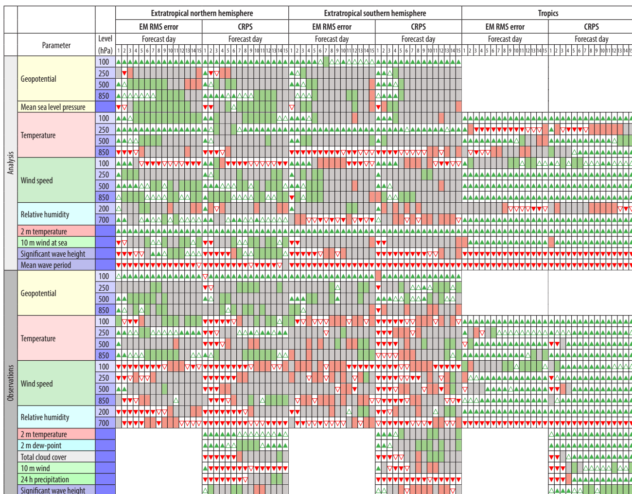
Figure 2 ENS scorecard of IFS Cycle 45r1 versus IFS Cycle 43r3 for medium-range/monthly forecasts up to forecast day 15, verified by the respective analyses and observations at 00 and 12 UTC, based on 408 ENS forecast runs in the period December 2016 to June 2018. See Box A for a discussion of how scores computed against analyses have been affected by changes to the analysis in IFS Cycle 45r1.
