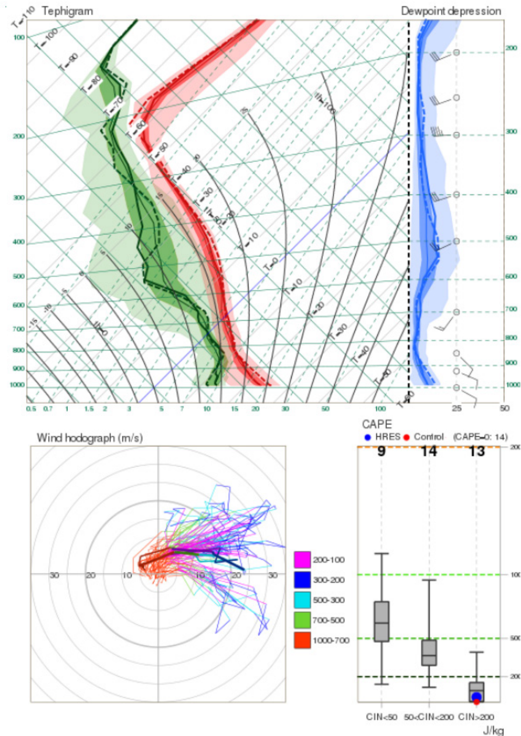
Figure 4 Vertical profile chart for the city of Plevin in northern Bulgaria affected by the severe thunderstorm on 15 May 2018. The forecast lead time is 108 hours, the valid time is 12 UTC on 15 May.
