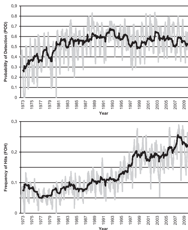
FIG. 3. (top) POD and (bottom) FOH calculated using 91- (gray line) and 365-day (black line) running means.
