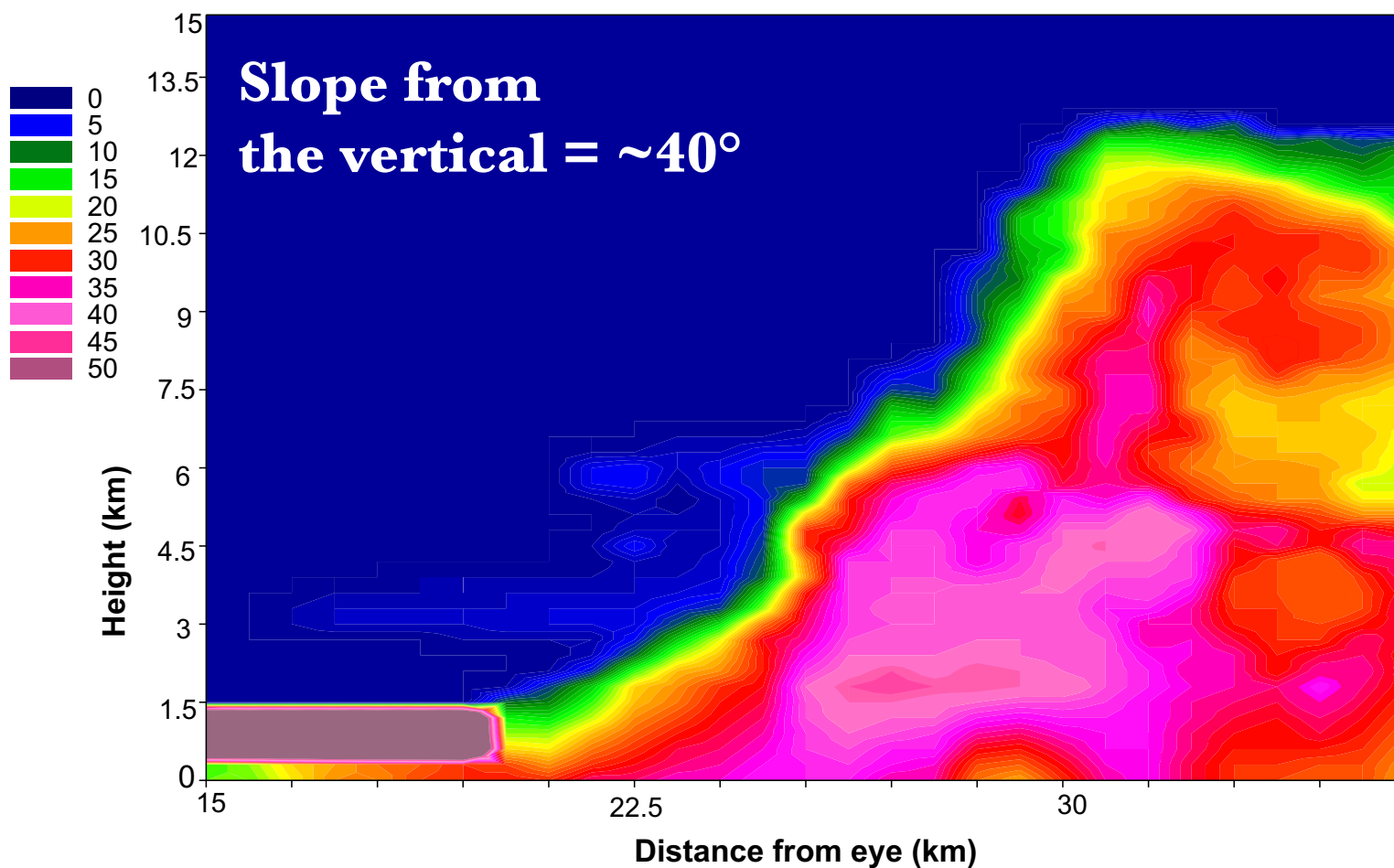
Radar Reflectivity Cross Section Hurricane Elena 1985
