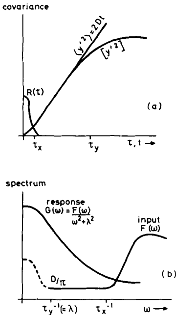
Fig. 2. Input and response of stochastically forced (single component) climate model with linear feedback; (a) covariances, (b) spectra. In the ranges \tau_x \leq \tau < \tau_y and \tau_y^{-1} \leq \omega < \tau_x^{-1} the models with and without feedback are identical. In the range \omega \leq \tau_y^{-1} the spectrum F(\omega) cannot be regarded as part of the "weather input", but is coupled to the climate response.
