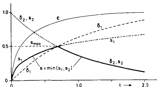
Fig. 3. Predicted climate changes \delta_1 relative to initial state and \delta_2 relative to asymptotic state, statistical error \epsilon , and skill parameters s_1 , s_2 and s = \min(s_1, s_2) , for a linear (single component) climate system. The initial value is chosen as y_0 = (R_\infty)^{1/2} = 1 (in this case s_2 and \delta_2 happen to coincide).
