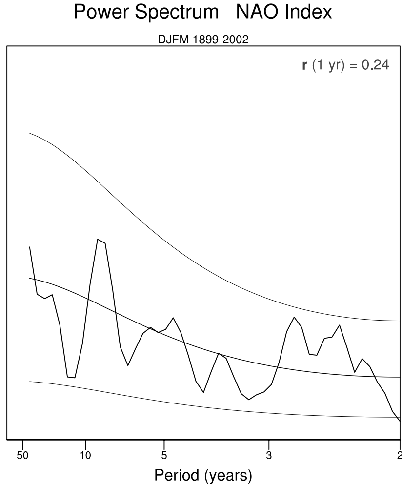
Figure 12. Power spectrum of the mean winter (December-March) NAO index over 1899-2002, defined as in the middle panel of Figure 10. Also shown is the corresponding red noise spectrum with the same lag one autocorrelation coefficient (0.24) and the 5 and 95% confidence limits.
