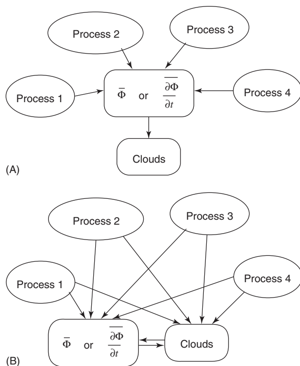
Figure 3 Schematic of the different approaches to cloud parameterization: (A) the principles of 'integrating' cloud schemes; (B) the process-oriented approach. Note that arrows indicating the obvious direct interactions between individual processes other than cloud processes have been omitted for clarity.
