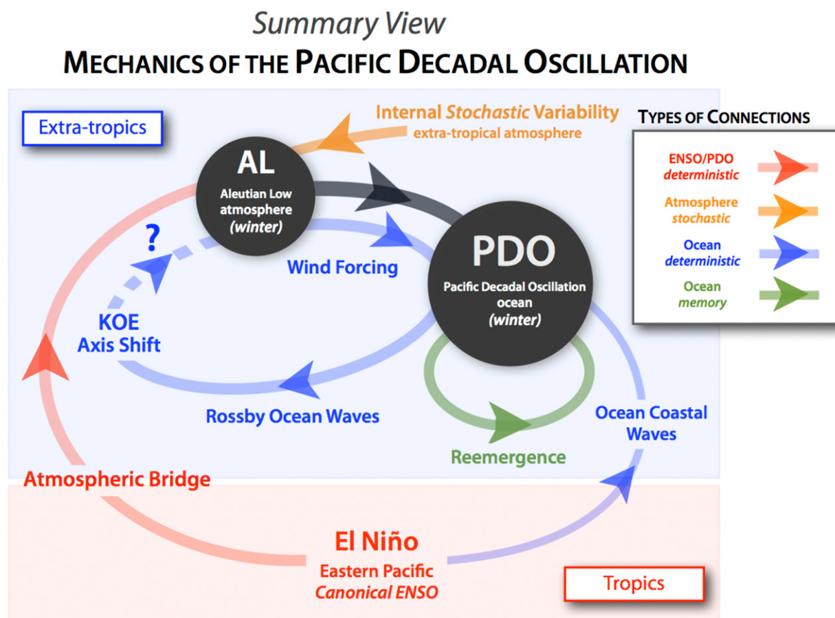
FIG. 14. Summary figure of the basic processes involved in the PDO.
