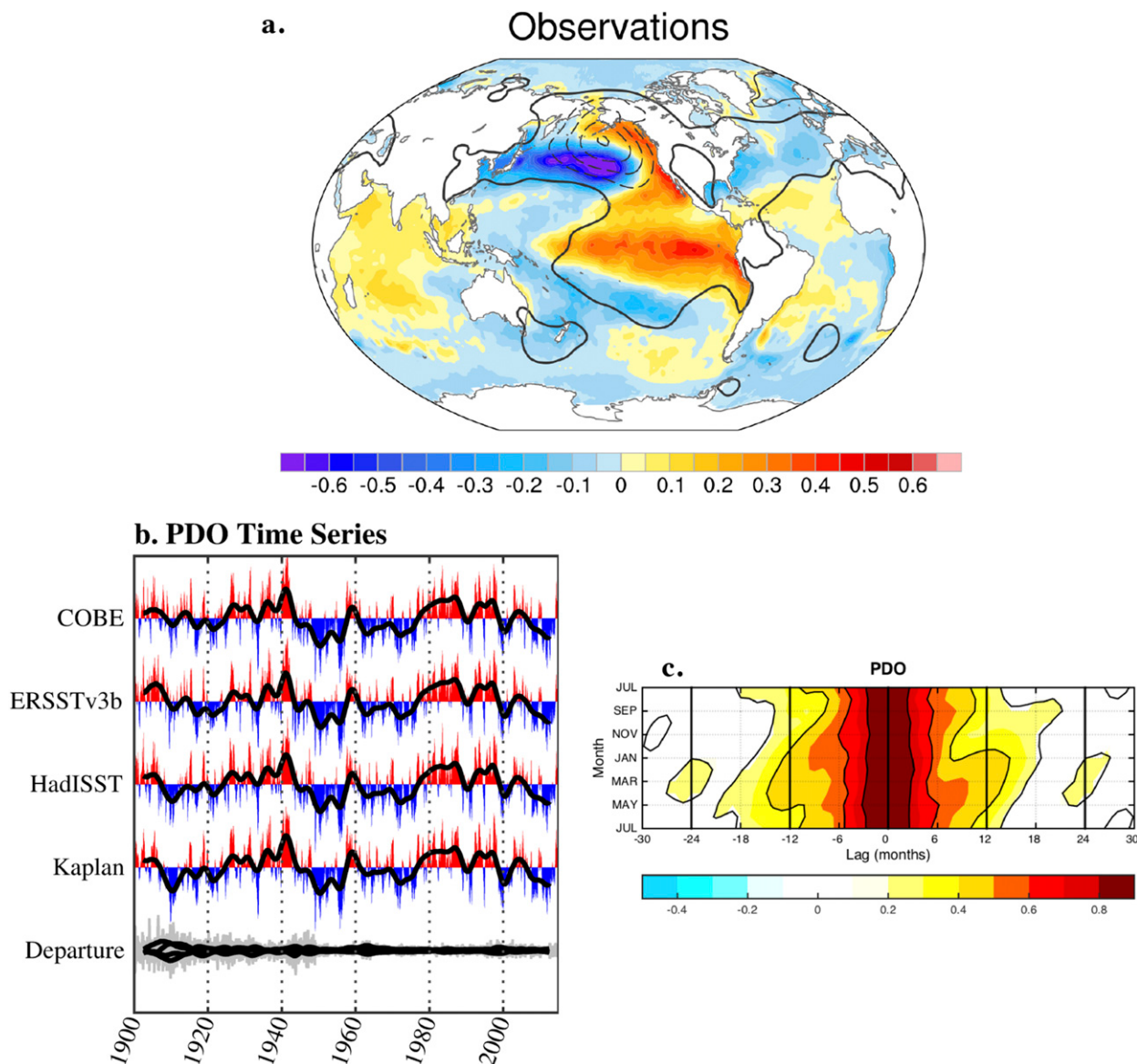
FIG. 1. The PDO over the historical record (1901–2014). (a) Regression of global monthly SST (shading; interval is 0.05^{\circ}\text{C} ) and DJF SLP (contours; interval is 1 hPa) anomalies onto the PDO time series from the HadISST dataset. Note that a positive PDO is associated with negative central North Pacific SSTA. (b) PDO index time series determined from the SST datasets, Centennial Observation-Based Estimates (COBE; Ishii et al. 2005), ERSST.v3b (Smith et al. 2008), HadISST (Rayner et al. 2003), and Kaplan (Kaplan et al. 1998). Positive (negative) values are drawn in red (blue). The thick black line in each panel shows the smoothed (6-yr lowpass; Zhang et al. 1997) time series. The last series in (b) shows the departure of each time series from the mean of all four time series. (c) Seasonal cycle of (3-month running mean) PDO index autocorrelation. Contour (shading) interval is 0.2 (0.1). Only values that are 95% significant are shaded. The month ordinate indicates the time of the PDO base month, and the lag indicates how far ahead or behind the PDO is; for example, the value plotted at (5, MAY) represents the correlation between the May value of the PDO and the subsequent October value of the PDO.
