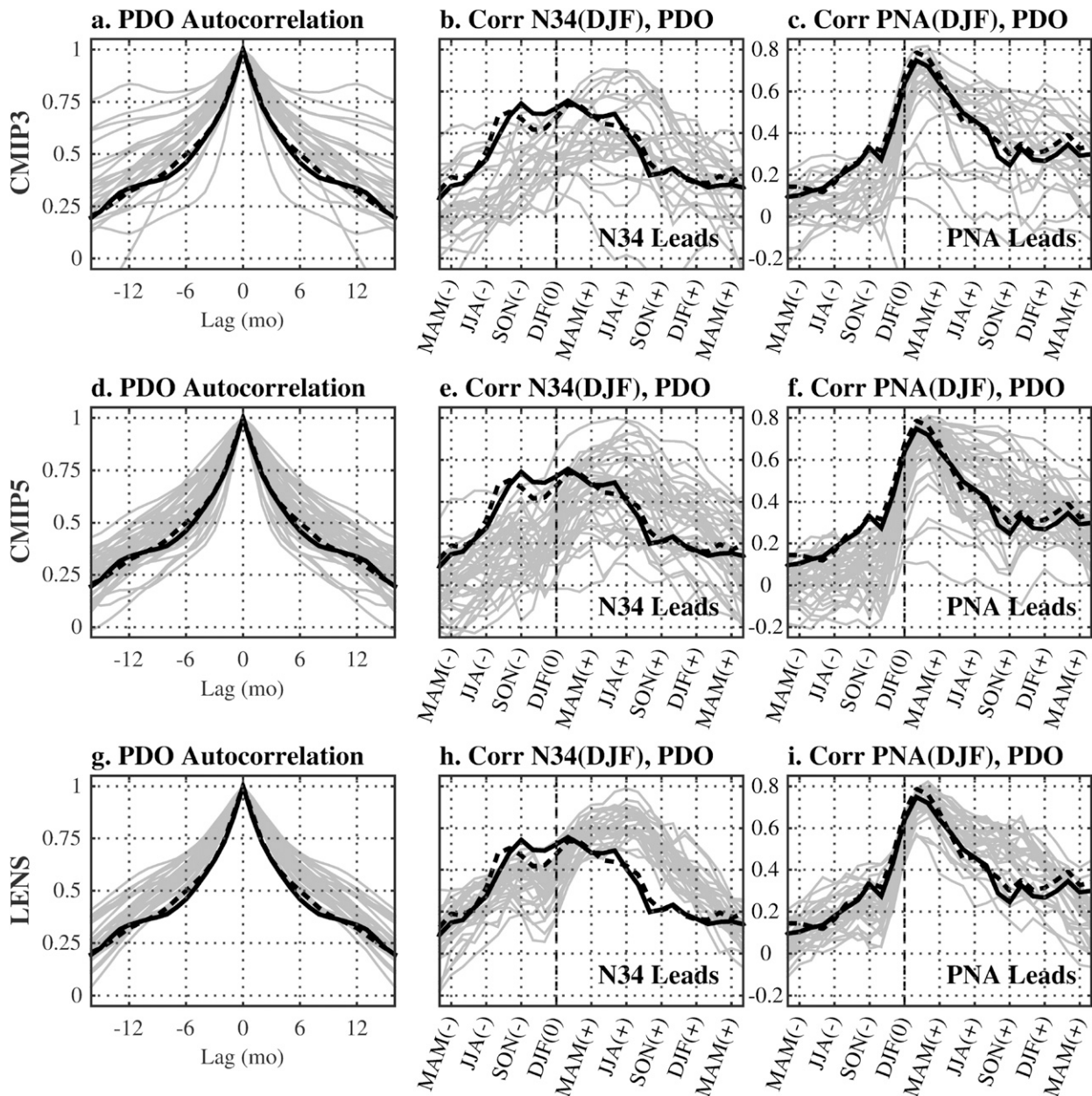
FIG. 9. Temporal relationships relevant to the PDO for the (top) CMIP3, (middle) CMIP5, and (bottom) CSM-LE (LENS) ensembles. Shown are (a),(d),(g) the autocorrelation of the monthly PDO index; (b),(e),(h) the lagged seasonal correlation between the seasonal PDO index and the DJF averaged Niño-3.4 index; and (c),(f),(i) the lagged seasonal correlation between the seasonal PDO index and the DJF-averaged PNA index. In all panels the thin gray lines indicate model correlations, the thick solid black line indicates correlations for indices from the HadISST data, and the thick dashed line indicates correlations with indices from the ERSST.v3b data. In (c),(f),(i) the observed DJF PNA time series is obtained from the twentieth-century reanalysis. Observed correlations are taken over the time period 1901–2009, CMIP3 over 1900–99, CMIP5 over 1901–2004, and LENS over 1920–2005. For seasonal correlations, positive lags indicate that the Niño-3.4 or PNA index leads the seasonal PDO index, and the label along the abscissa indicates the season for which the PDO is defined.
