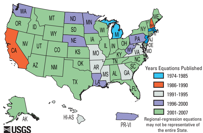
Figure 10. Age map indicating when the last regional-regression analysis for rural peak flows was published by the U.S. Geological Survey.
