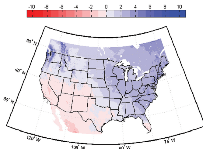
Figure 3. Change in 30-year mean annual precipitation, measured in centimeters per year (cm/year). The median difference between 1971–2000 and 2041–2070 is based on 112 projections obtained from “Statistically Downscaled WCRP CMIP3 Climate Projections” ( http://gdo-dcp.ucllnl.org/downscaled_cmip3_projections ).
