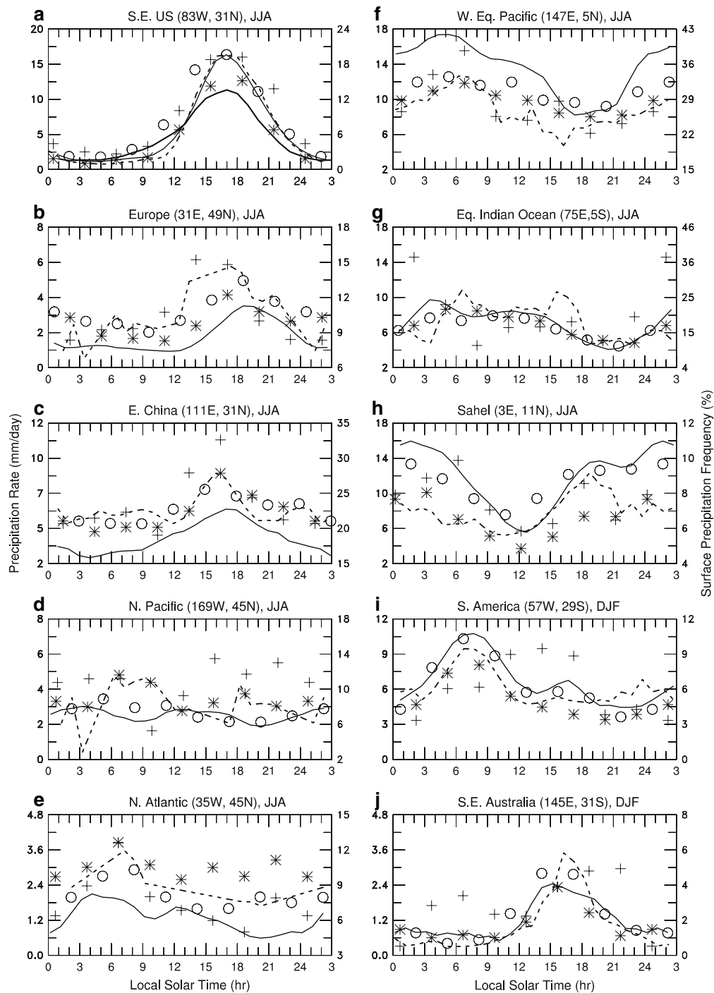
Fig. 4 Mean diurnal cycle of summer precipitation at ten selected 2^\circ \times 2^\circ boxes from surface weather reports (plus indicates frequency in % on the right-hand ordinate, 1975–1997 mean), CMORPH (open circle indicates 2003–2005), TRMM 3B42 (asterisks indicates 1998–2005), PERSIANN (thin solid lines indicates 2002–2005), and MI
