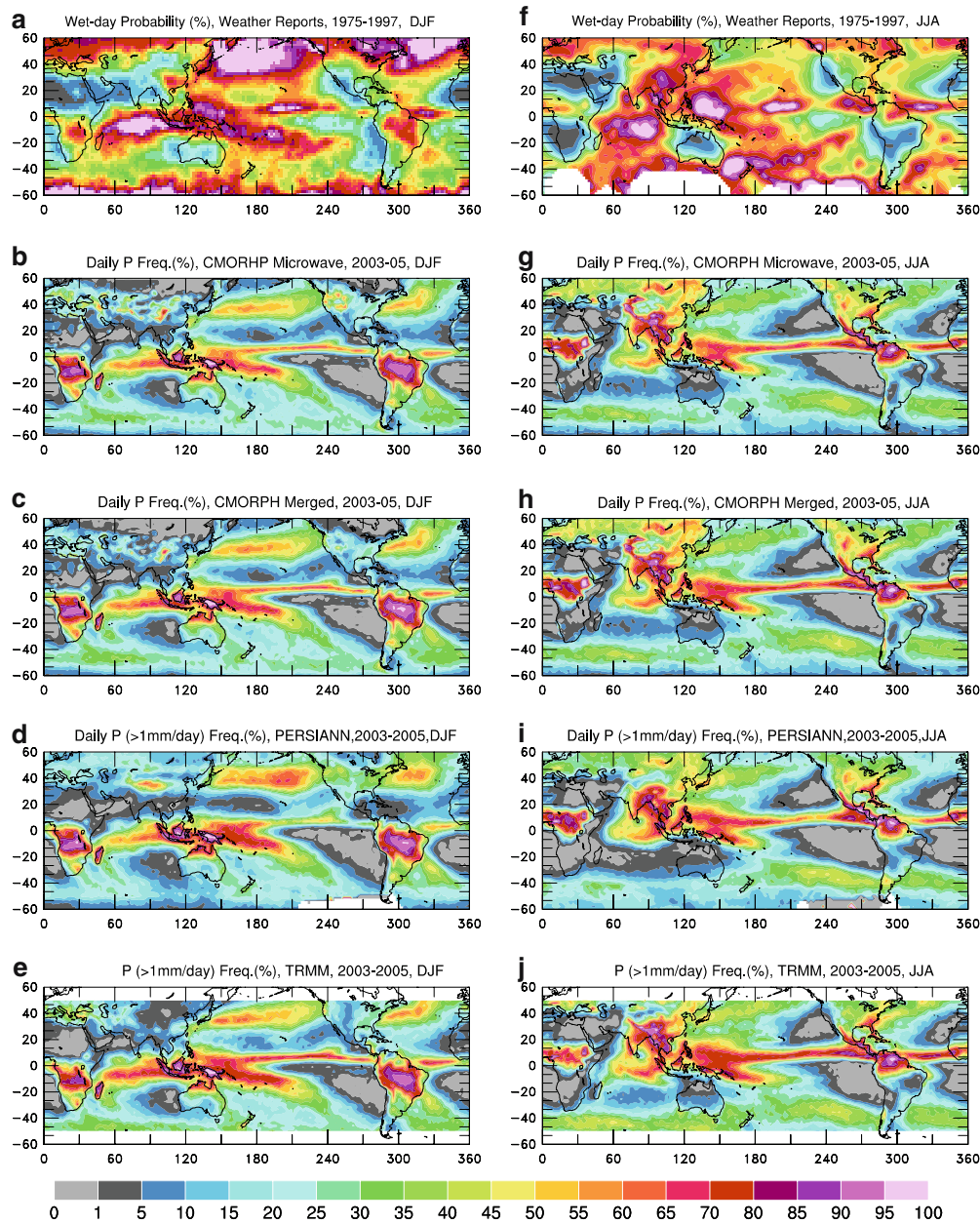
Fig. 2 2003–2005 mean DJF (left column) and JJA (right column) daily precipitation (>1 mm/day) frequency (%) from microwave only (2nd row, from CMORPH), merged CMORPH (3rd row), PERSI-
