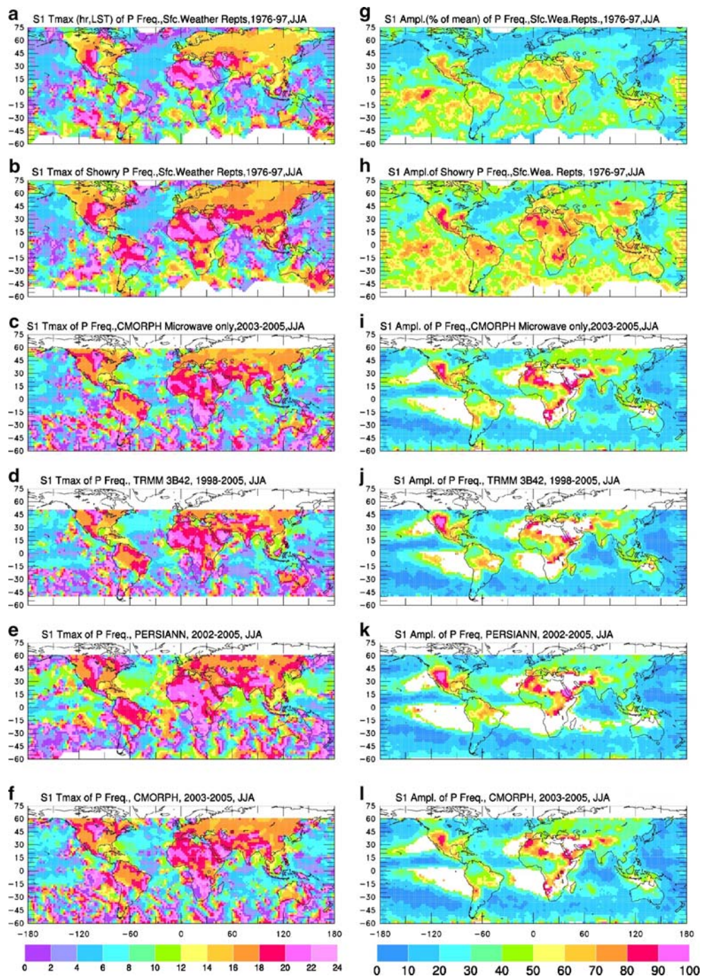
Fig. 10 Same as Fig. 5 but for precipitation frequency from weather reports and the satellite observations (in contrast to precipitation amount from satellite observations in Fig. 5)
