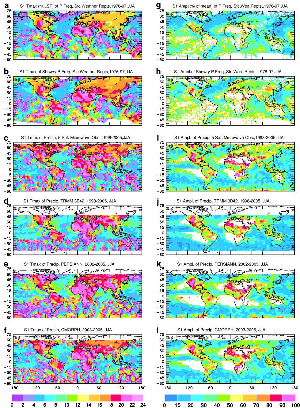
Fig. 5 The phase (local solar time in hours of the maximum, left column ) and amplitude (in % of daily mean, right column ) of the 24-h harmonic estimated from the mean diurnal anomalies of JJA precipitation frequency for non-drizzle and showery precipitation from surface weather reports ( top two rows ), and of JJA precipitation
