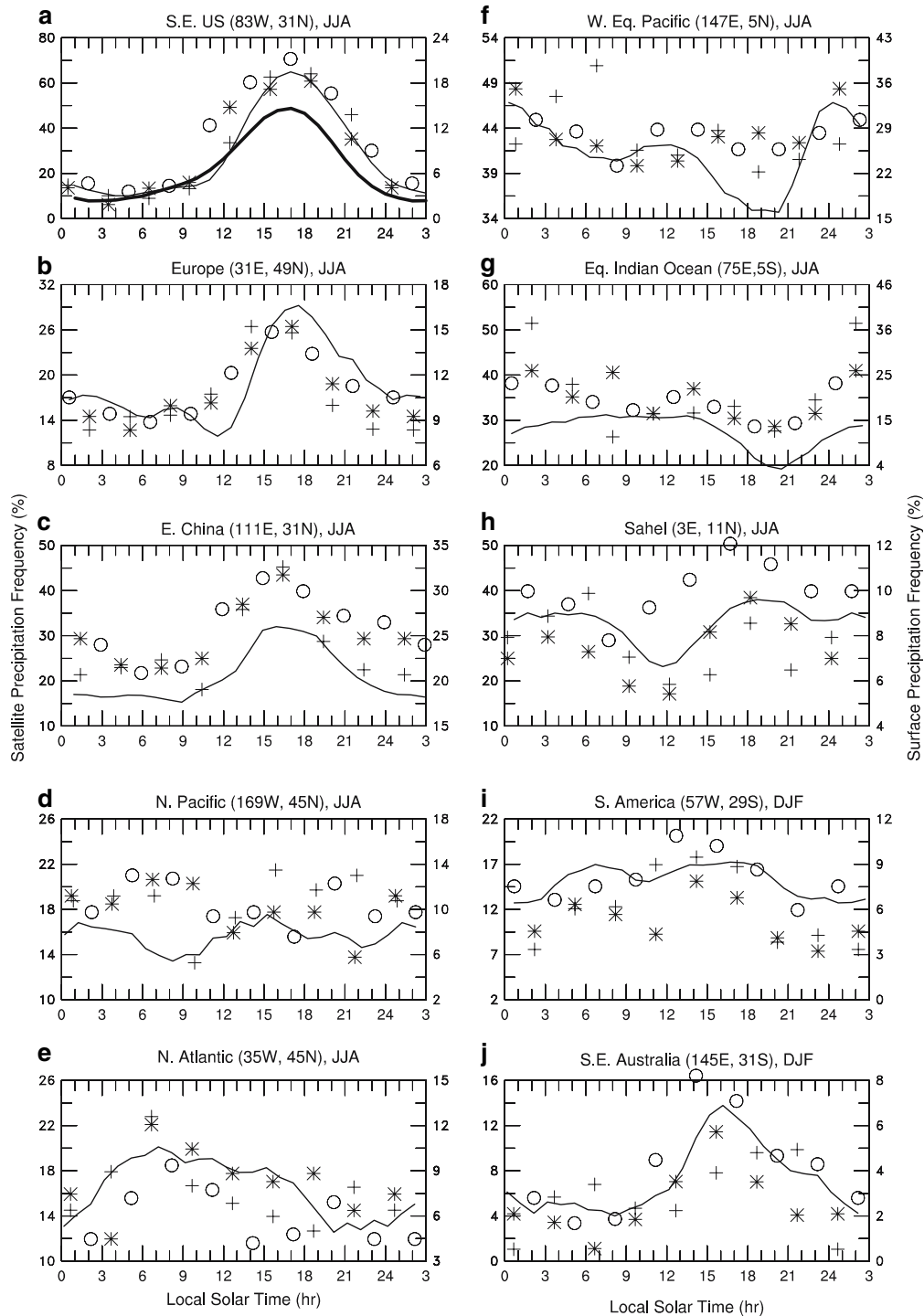
Fig. 8 Same as Fig. 4 but for the mean diurnal cycle of precipitation frequency
