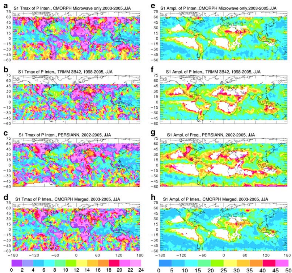
Fig. 11 Same as Fig. 5 but for precipitation intensity from satellite observations
