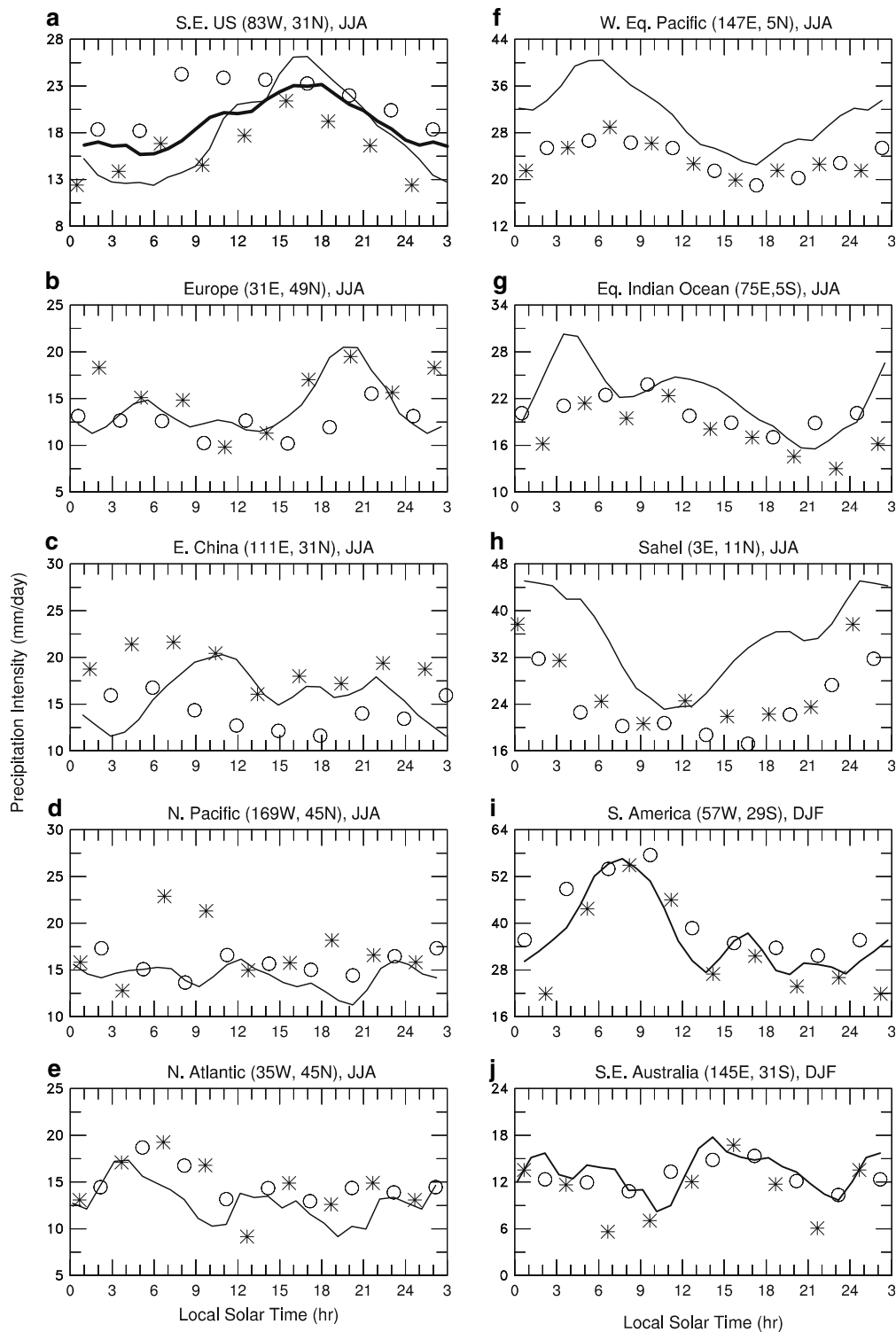
Fig. 9 Same as Fig. 4 but for the mean diurnal cycle of precipitation intensity
