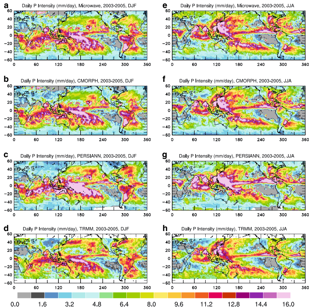
Fig. 3 Same as Fig. 2 but for daily precipitation intensity (mm/day) from satellite observations
