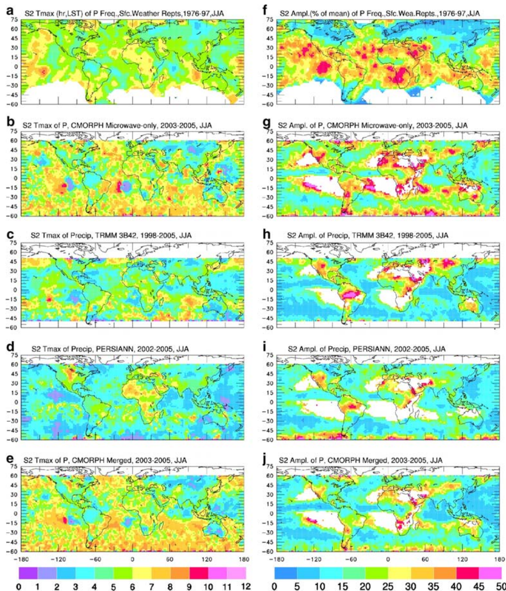
Fig. 7 The phase (local solar time in hours of the first maximum, left column ) and amplitude (in % of daily mean, right column ) of the 12-h harmonic estimated from the mean diurnal anomalies of JJA precipitation frequency for non-drizzle precipitation from surface weather reports ( top row ), and of JJA precipitation amount from
