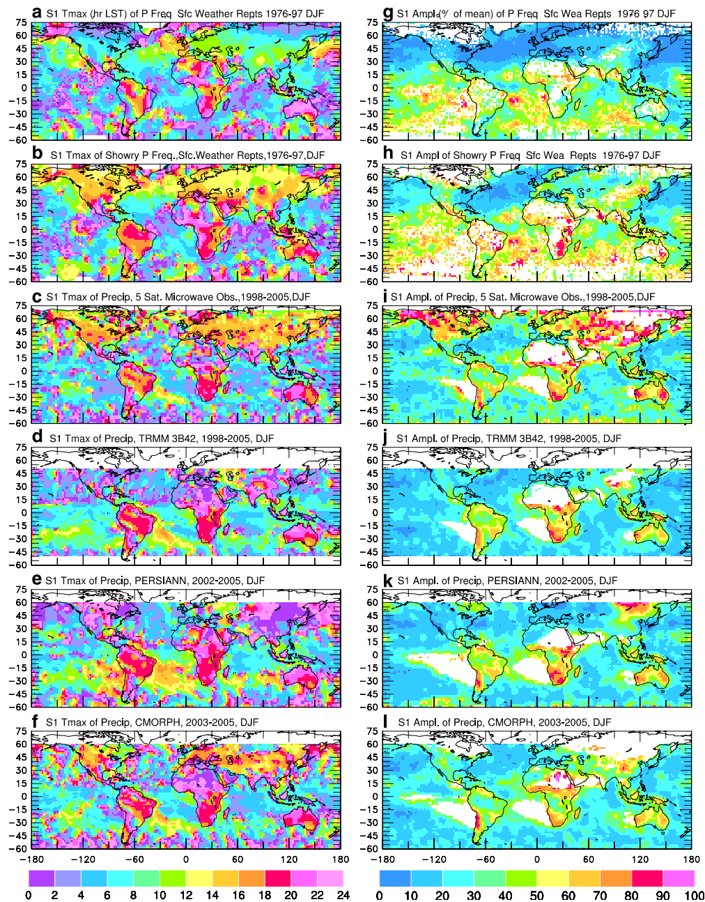
Fig. 6 Same as Fig. 5 but for December–February
