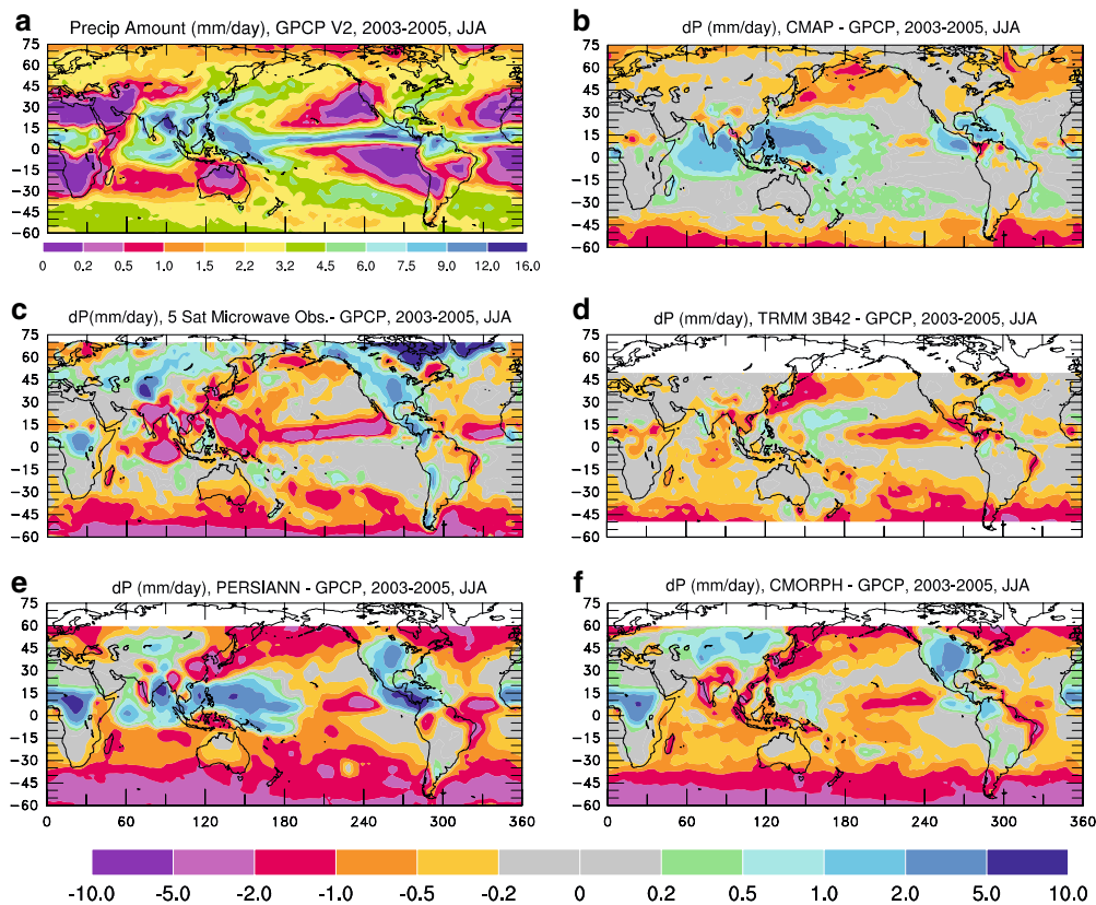
Fig. 1 2003–2005 mean June–August precipitation from GPCP (Adler et al. 2003), and the difference between CMAP (Xie and Arkin 1997) and GPCP (top right) and between each of the four pure satellite estimates and GPCP
