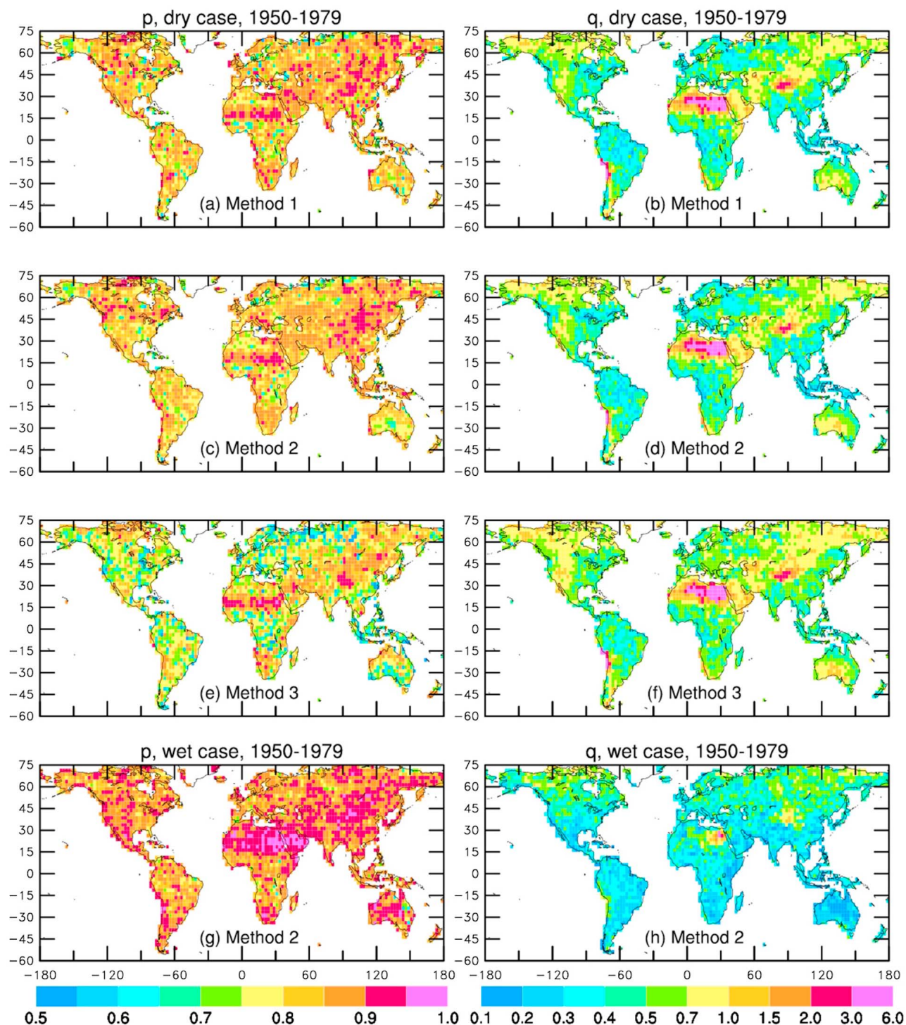
Figure A2. The (a, c, e, g) p and (b, d, f, h) q parameters used in the sc\_PDSI calculations for (a-f) dry cases using three slightly different methods (Figures A2a-A2f) and for wet cases using method 2 (Figures A2g and A2h). The PE\_pm was used in the calculations (similar if PE\_th was used).
