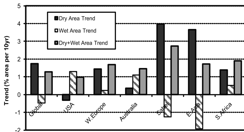
Figure 15. Linear trends in the smoothed time series of the percentage dry, wet, and dry plus wet areas shown in Figures 14 and 16. The trends are based the sc\_PDSI\_pm , and they are statistically significant at the 5% level. Results are similar for the other forms of the PDSI, with the drying trend slightly larger when PE\_th is used.
