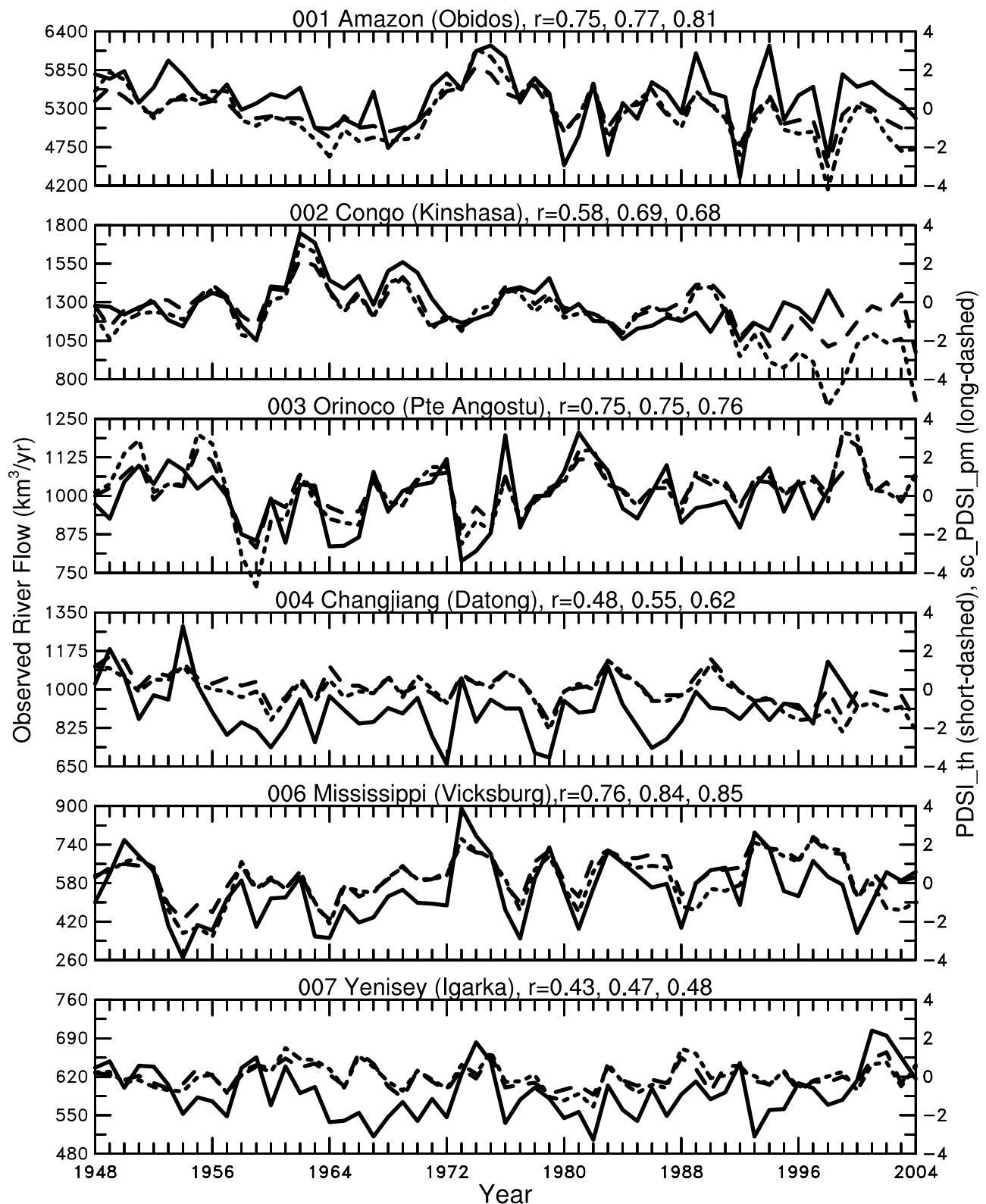
Figure 6. Time series of observed water-year (1 October to 30 September) streamflow ( \text{km}^3 \text{ yr}^{-1} , solid line) at the farthest downstream station for the world's six largest rivers compared with basin-averaged PDSI_th (short dashed line) and sc_PDSI_pm (long dashed line). The lines for PDSI_pm are similar to those for sc_PDSI_pm and thus are not shown. The correlation coefficients ( r ) are for streamflow versus, from left to right, PDSI_th, PDSI_pm, and sc_PDSI_pm. Note the streamflow for Yenisey was detrended before the correlation analysis (same for Figures 7 and 8).
