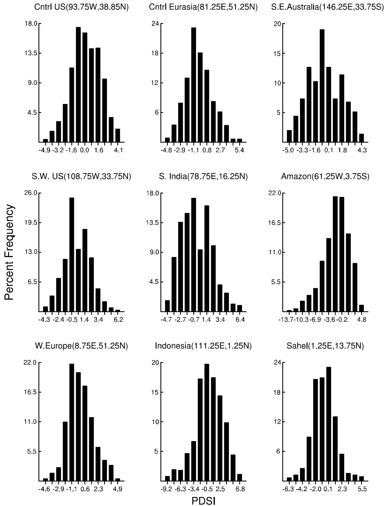
Figure 3. Same as Figure 2 but for sc\_PDSI\_pm . To increase the comparability of the shapes of the histograms in Figures 2 and 3, the same number of bins (not the same intervals for the bins) is used in Figures 2 and 3 given the same sample size and different value ranges between the PDSI\_pm and sc\_PDSI\_pm cases.
