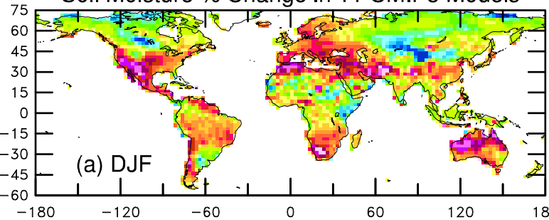
Soil Moisture % Change in 11 CMIP5 Models
