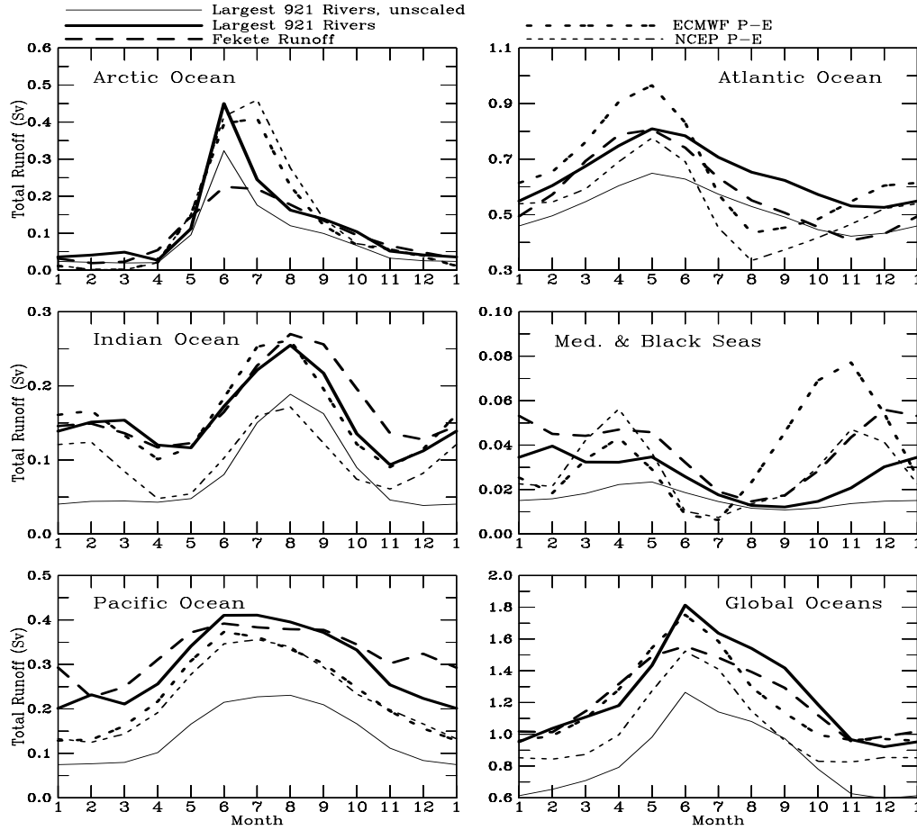
Fig.5: Mean annual cycle of freshwater discharge (Sv) into individual and global oceans based on various estimates. The thin solid line is for the estimate based on the 921 rivers without scaling to account for the un-monitored areas.
