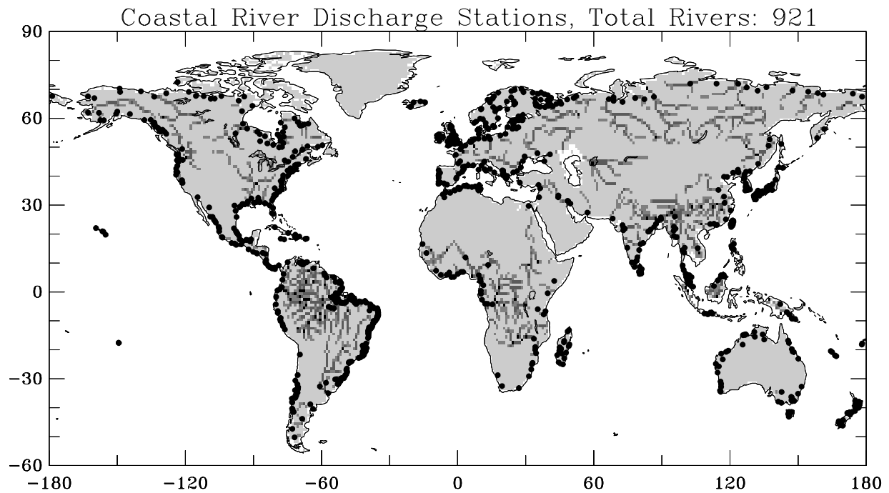
Fig.1: Distribution of the farthest downstream stations for world largest 921 rivers included in these studies. Also shown are the worlds major river systems simulated by a river transport model.
