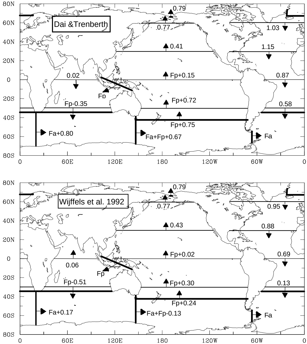
Fig.7: Top: Oceanic freshwater flux (Sv) at selected latitudes estimated by this study using the 921-river based discharge and the ECMWF reanalysis based oceanic P-E (Table 1). The solid lines are ocean basin boundaries. Bottom: Same as Top but from Wijffels et al. (1992).
