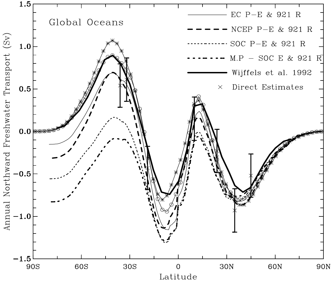
Fig.6: Latitudinal distribution of annual freshwater transport (Sv, positive northward) by the global oceans estimated using various oceanic P-E (see text for more details) and continental runoff estimated based on streamflow data of world largest 921 rivers. The thin-solid line with circles and stars are inferred oceanic transport of freshwater from atmospheric moisture transport in the ECMWF and NCEP/NCAR reanalyses, respectively. The thick solid line is an estimate by Wijffels et al. (1992) based on BR75. Also shown are some direct estimates (crosses) adopted from Wijffels (2001).
