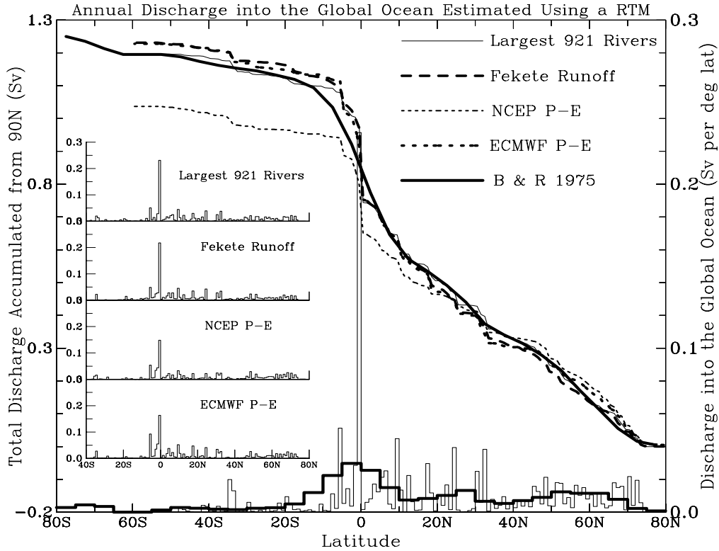
Fig.4: Estimates of annual mean continental freshwater discharge (Sv) into the global oceans for each 1^\circ latitude zone (right ordinate and lower stepwise lines, and the insert) and the cumulated discharge starting from 90^\circ\text{N} (Sv, upper curves). Each line pattern represents an estimate based either on the largest 921 rivers (thin solid line) or on a runoff field (dashed lines), which was used to force a river transport model to derive the discharge. Also shown is an estimate from Baumgartner and Reichel (1975, thick solid line).
