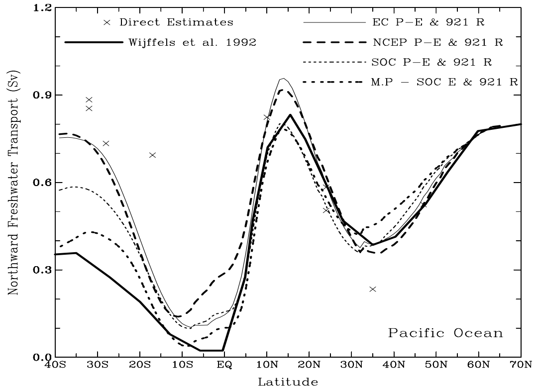
Fig.9: Same as Fig.6 but for the Pacific Ocean, with the Indonesia Throughflow excluded
