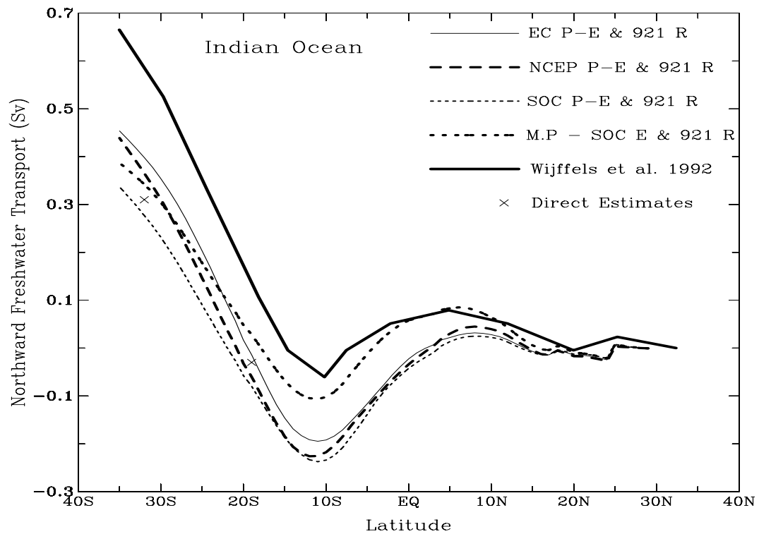
Fig.10: Same as Fig.9 but for the Indian Ocean, with only two direct estimates at 19°S and 32°S.
