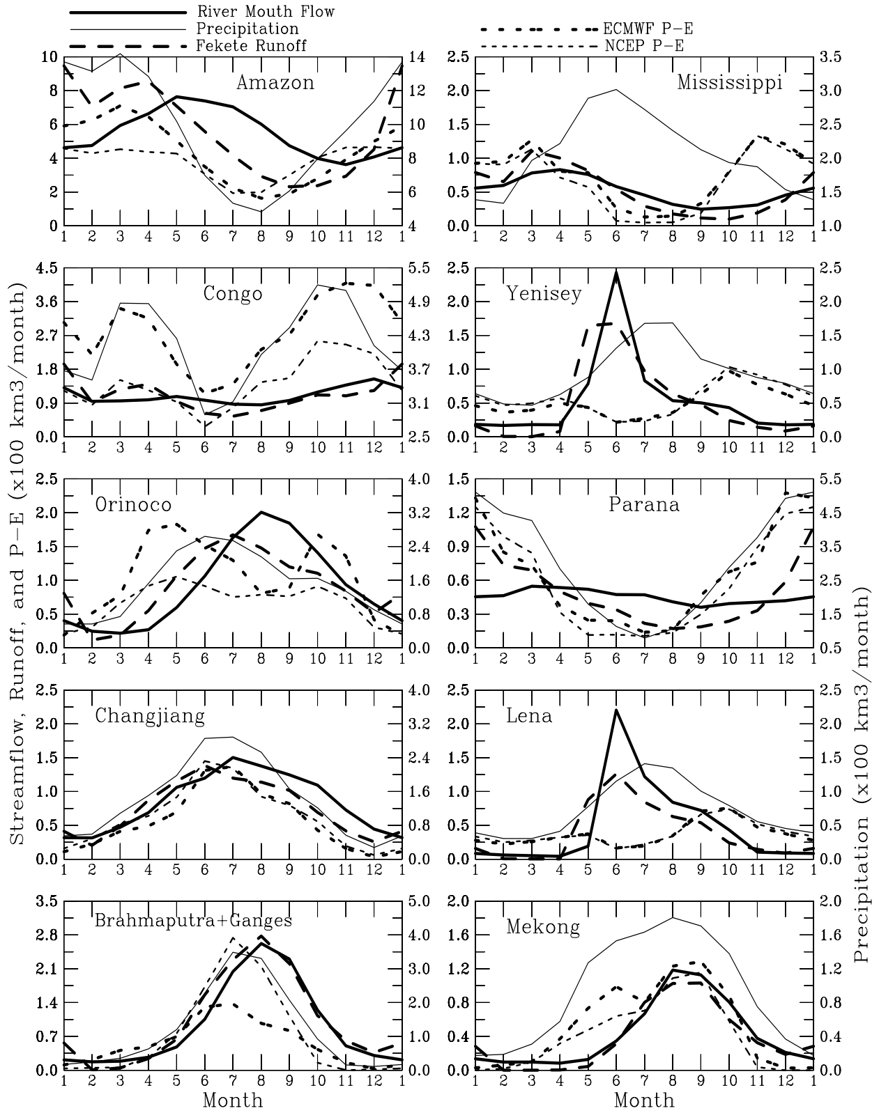
Fig.2: Mean annual cycle of river discharge, river-basin integrated precipitation (read on the right ordinate), runoff, and reanalysis P-E for world largest 10 rivers. Note that the RTM was not used for this plot
