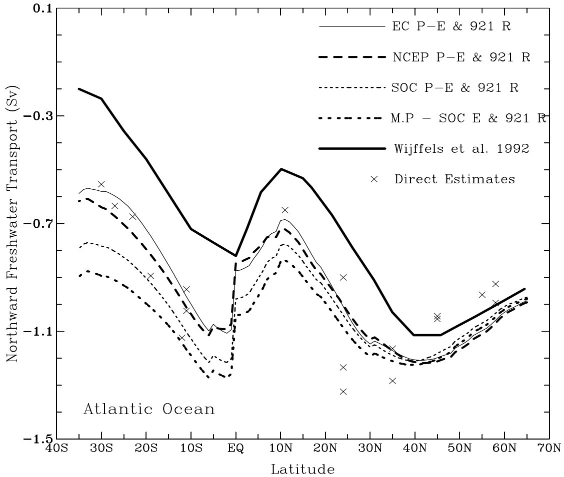
Fig.8: Same as Fig. 6 but for the Atlantic Ocean.
