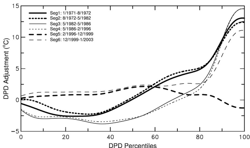
FIG. 11. The amount of DPD adjustment (based on QM) applied to the individual DPD reports at 1200 UTC for the 300-hPa level at a Japanese station (47580) for different segments (represented by different line styles) separated by detected changepoints as a function of the DPD percentiles, with larger DPD values in the higher percentiles.
