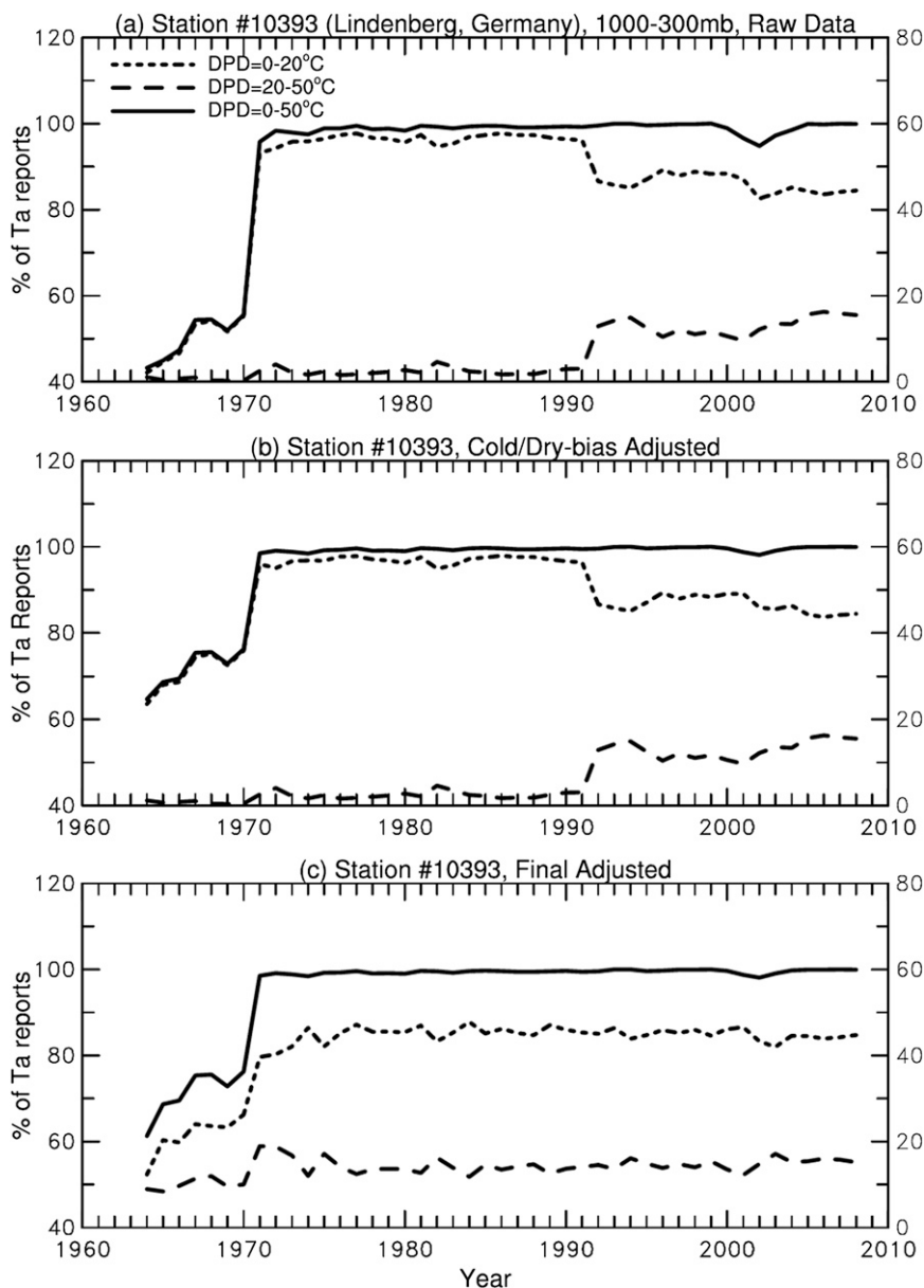
FIG. 9. Time series of annual DPD reports as a percentage of the total number of air temperature reports at the 1000-, 850-, 700-, 500-, 400-, and 300-hPa levels for \text{DPD} = 0^{\circ}\text{--}20^{\circ} , 20^{\circ}\text{--}50^{\circ} , and 0^{\circ}\text{--}50^{\circ}\text{C} cases in the (a) raw, (b) cold and dry bias-adjusted, and (c) final adjusted DPD data at the Lindenberg station. Note the \text{DPD} = 20^{\circ}\text{--}50^{\circ}\text{C} case (long-dashed line) is shown on the right-side ordinate.
