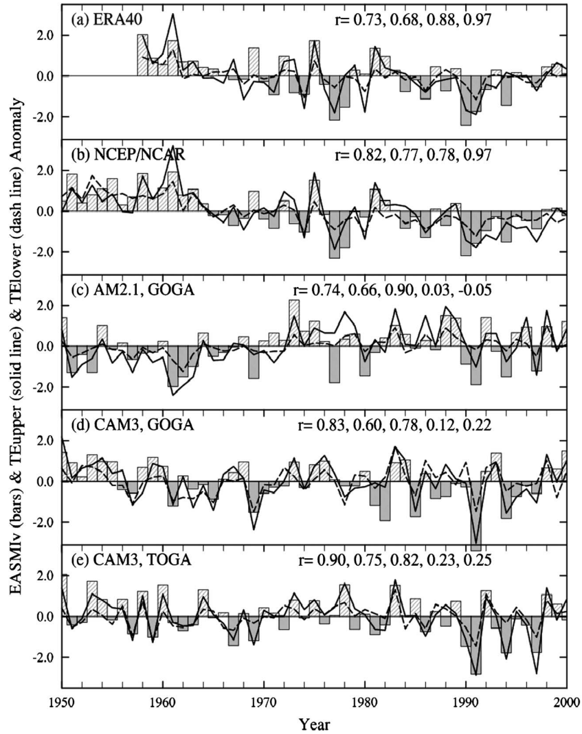
Figure 9. Same as Figure 8 but for the East Asian summer monsoon V index (EASMIv, bars) and the associated thermal contrasts TEupper and TELower over 20°–40°N.
