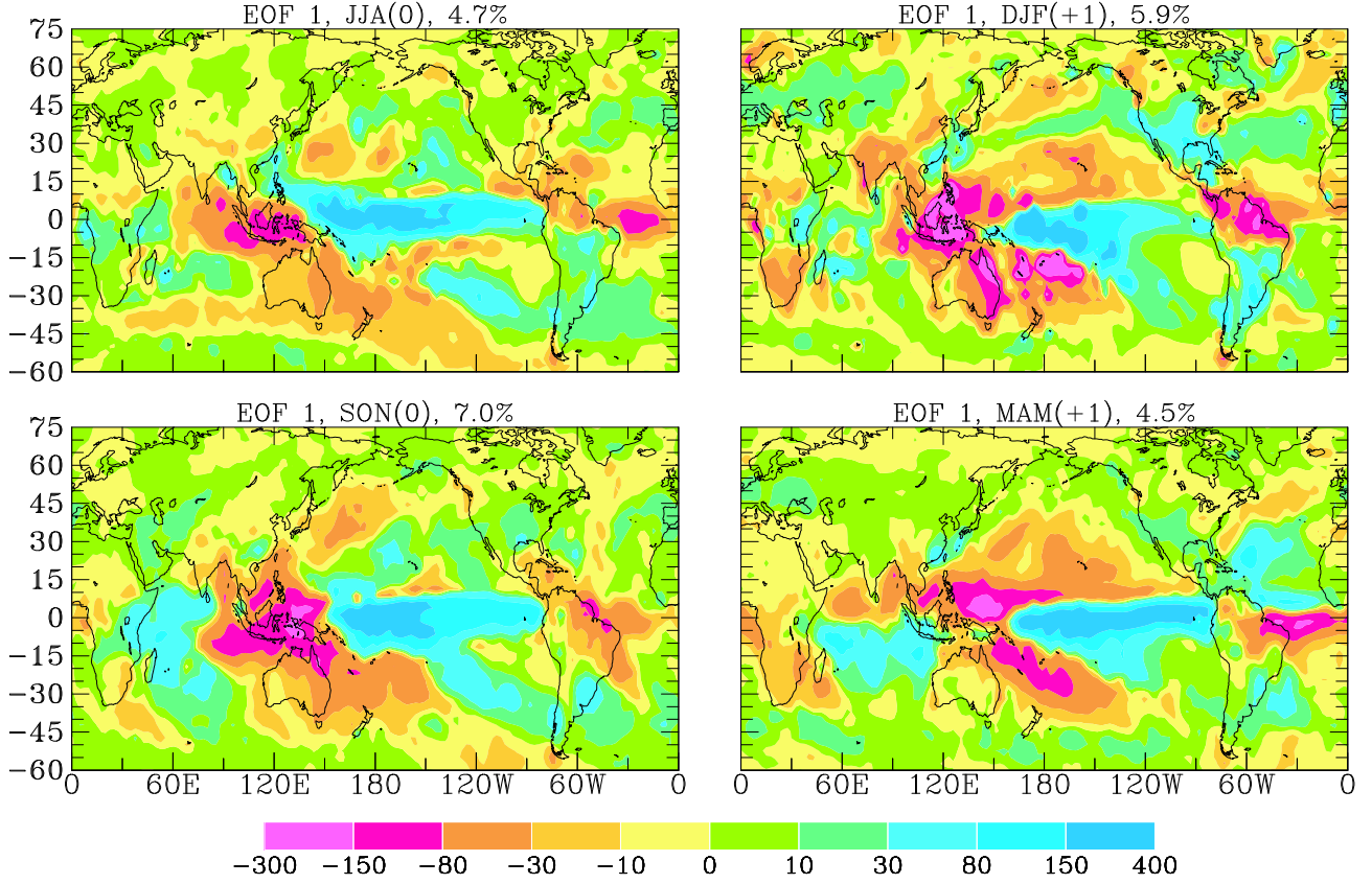
Figure 2. Same as Fig. 1c but for seasonal precipitation.
