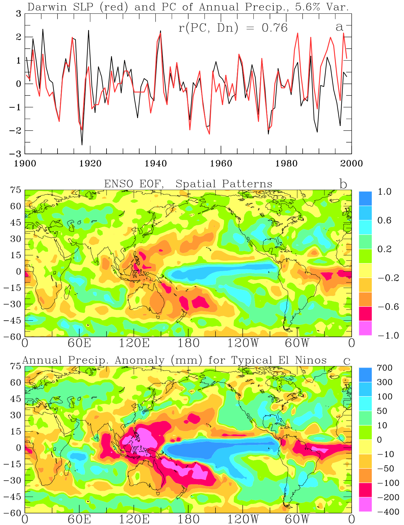
Figure 1. a: EOF 1 amplitudes (black line) for annual precipitation compared with normalized Darwin sea level pressure (red line) through 1998. Year n is plotted as n+0.5 . b: EOF 1 pattern normalized to represent the grid-box correlation between the amplitude and annual precipitation. c: annual precipitation anomalies (mm) associated with a +1.0 anomaly in the EOF 1 time series (i.e., \sim 1.5 standard deviations for annual Darwin SLP). Note that yellow and light-green colors indicate statistically insignificant values.
