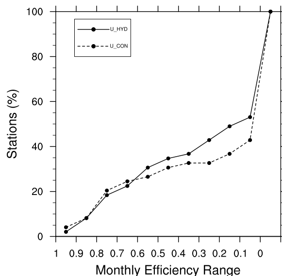
Figure 6. Cumulative efficiency distribution of monthly river discharge for the world's largest 50 rivers. The efficiency, Eff , is calculated from equation (1) in the text.
