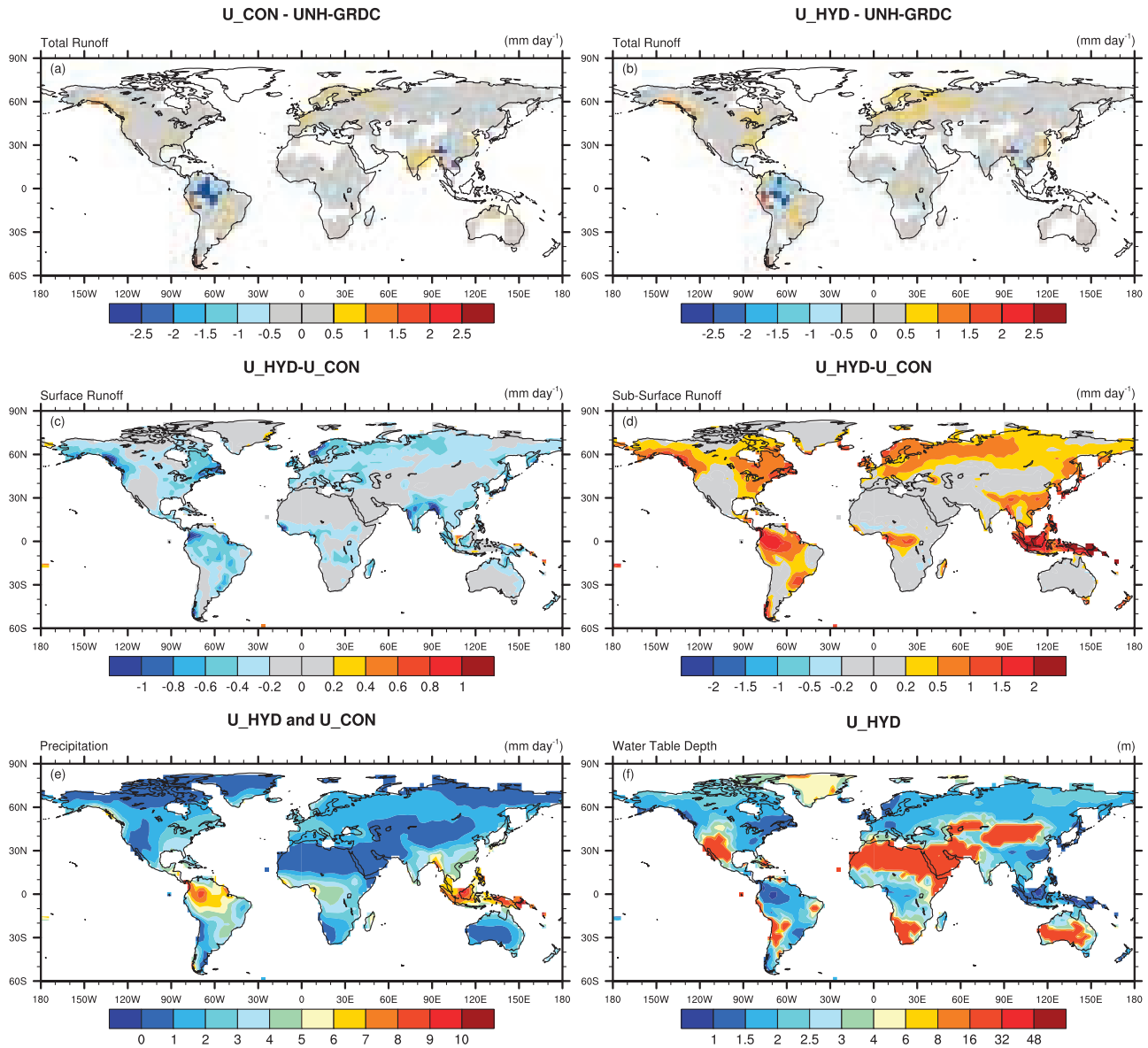
Figure 2. Annual mean of (a) U\_CON minus UNH-GRDC total runoff, (b) U\_HYD minus UNH-GRDC total runoff, (c) U\_HYD-U\_CON surface runoff, (d) U\_HYD-U\_CON subsurface runoff, (e) precipitation, and (f) U\_HYD water table depth, at the model T42 resolution. All in \text{mm day}^{-1} except for water table depth in m. For Figures 2a and 2b, UNH-GRDC runoff is from 0.5^\circ composite runoff fields [Fekete et al. , 2000, 2002] area-averaged to the model resolution but masked by UNH-GRDC observed runoff fields. Land areas in white indicate grid cells for which UNH-GRDC observed runoff is missing for more than 50% of the T42 grid cell.
