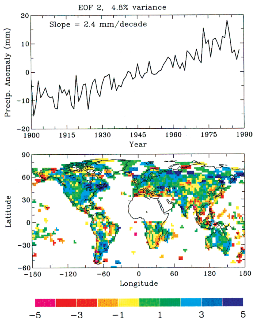
FIG. 10. Temporal coefficients and spatial patterns of the second leading EOF of annual precipitation anomalies over the globe, excluding northern Africa. Note that the coefficients are converted into globally aggregated precipitation anomalies associated with the EOF. Areas without data are in white.
