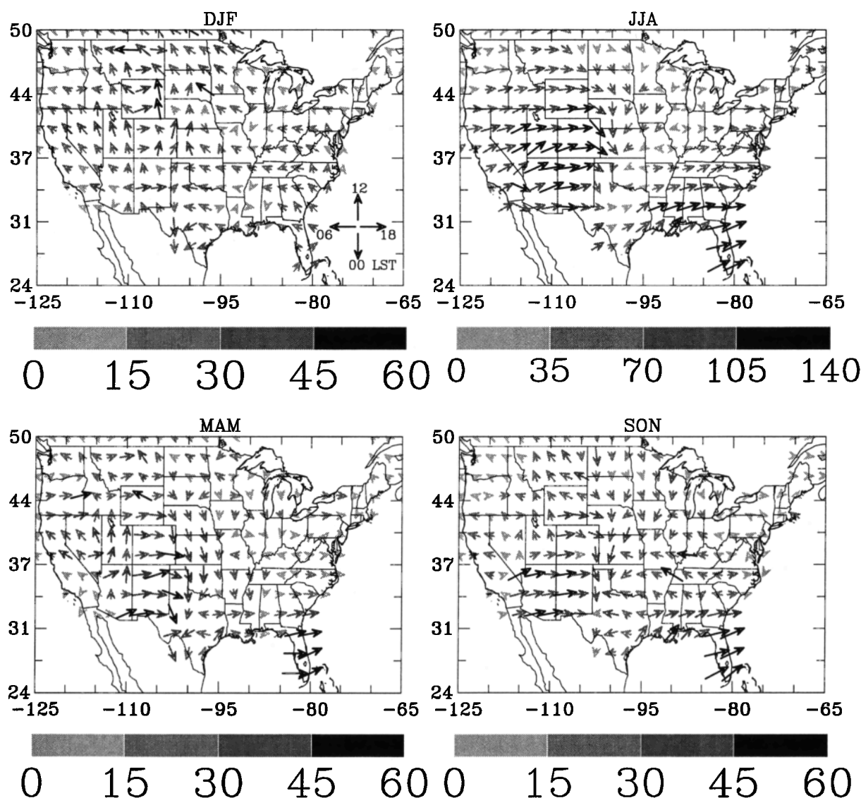
Figure 3. Vector plots of diurnal cycle of mean (1963-1993) precipitation amount. The vector length and grey levels represent the normalized amplitude in percentage (see section 2.1 for more details). The direction to which an arrow points denotes the local time at which the maximum amplitude occurs as indicated by the phase clock in the top left panel. (South = 0000 LST, West = 0600 LST, North = 1200 LST, and East = 1800 LST). For example, a vector pointing east means that the maximum amplitude occurs at 1800 LST.
