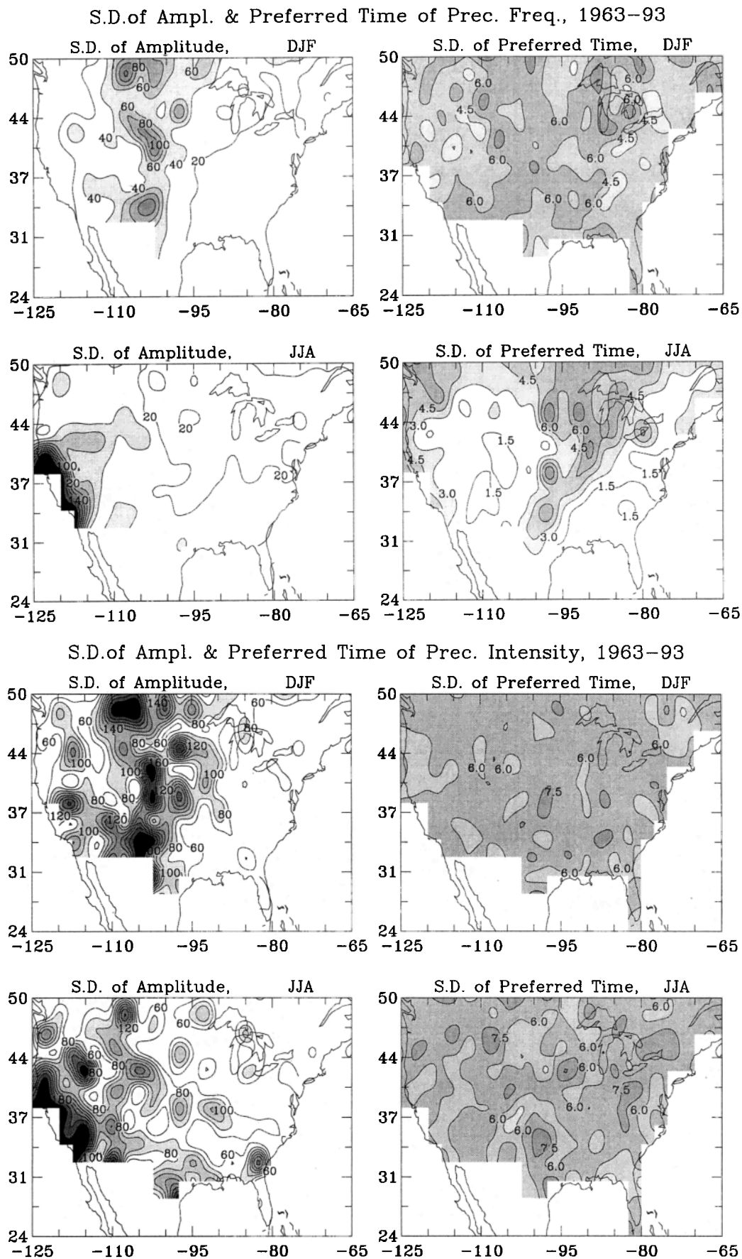
Figure 6. Standard deviations of the normalized amplitude (%) and preferred time (hour) for winter and summer precipitation frequency (a) and intensity (b) during the 1963–1993 period.
