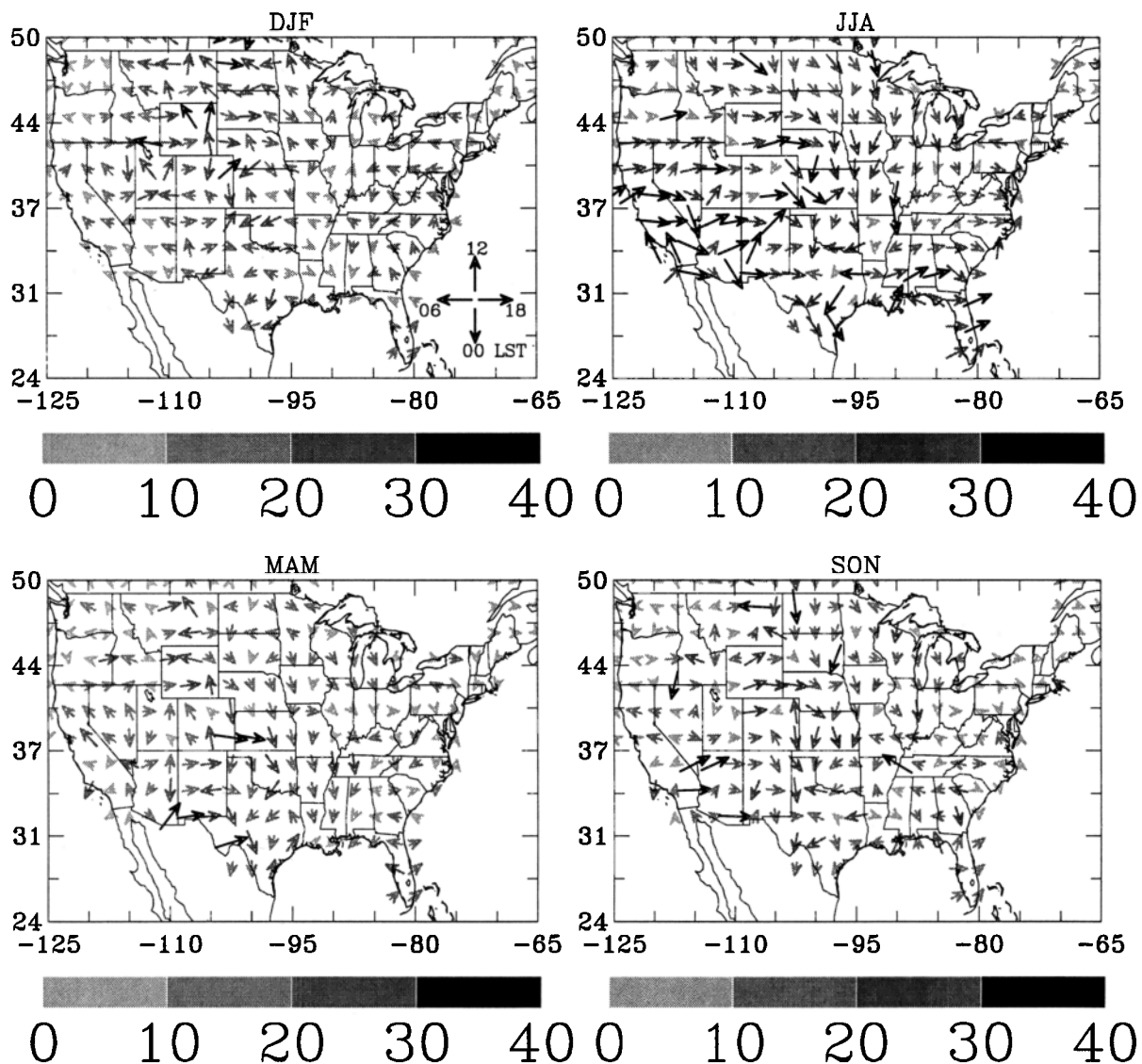
Figure 5. As for Figure 3 but for precipitation intensity.
