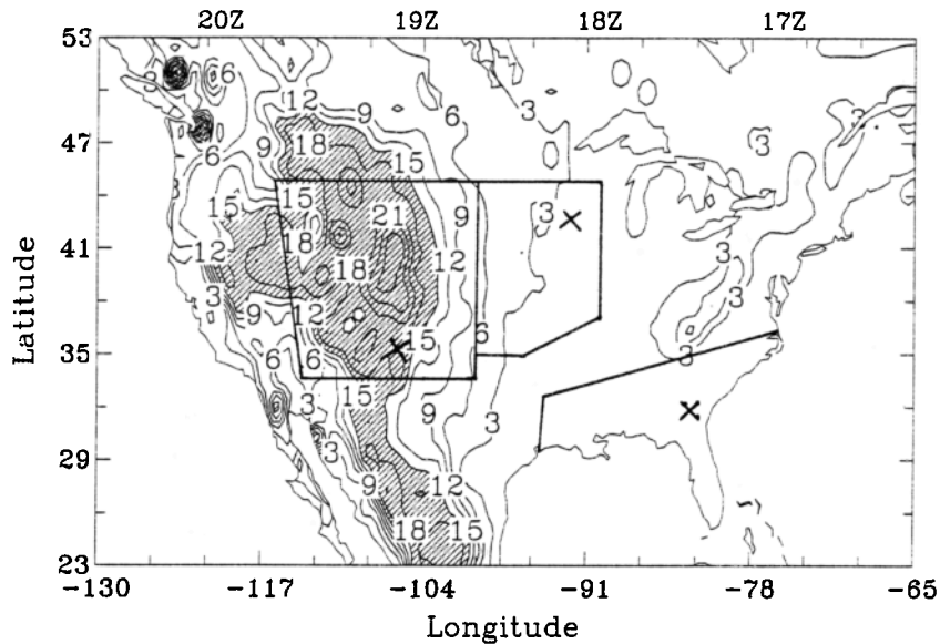
Figure 1. Approximate domain of simulation in the NCAR regional climate model (RegCM). Also shown are contour lines of topography (in 100 m, areas over 1500 m are hatched), the locations (marked by a cross) of the three grid boxes referred to in Figure 2, and the approximate definition of the southeastern United States, the Rocky Mountains, and the region east of the Rockies and the adjacent plains used in this study. The Greenwich time corresponding to local noon is shown at the top.
