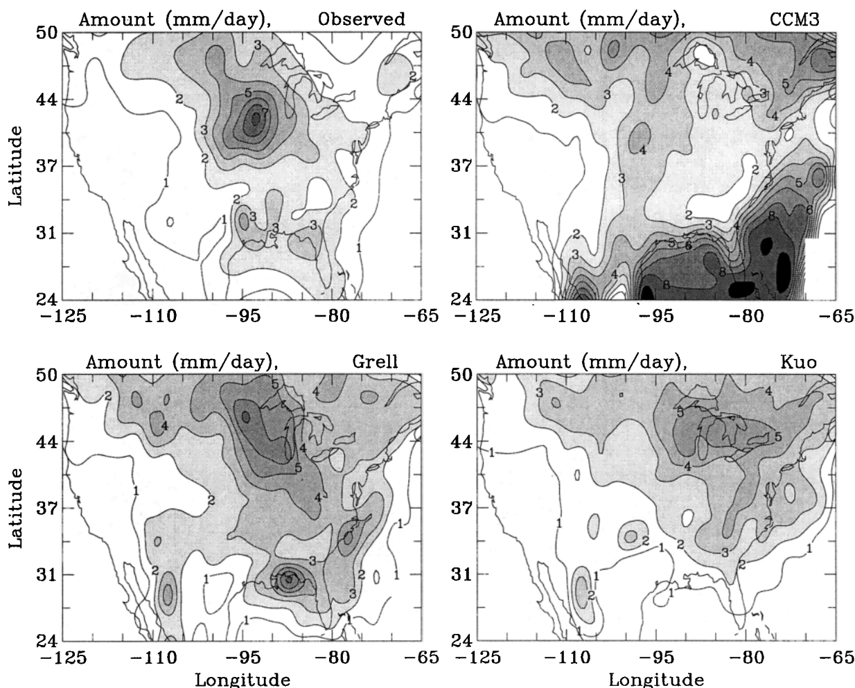
Figure 10. Observed and model simulated (with the three versions of cumulus convection schemes) total precipitation (mm/day) over the United States during the summer (JJA) of 1993.
