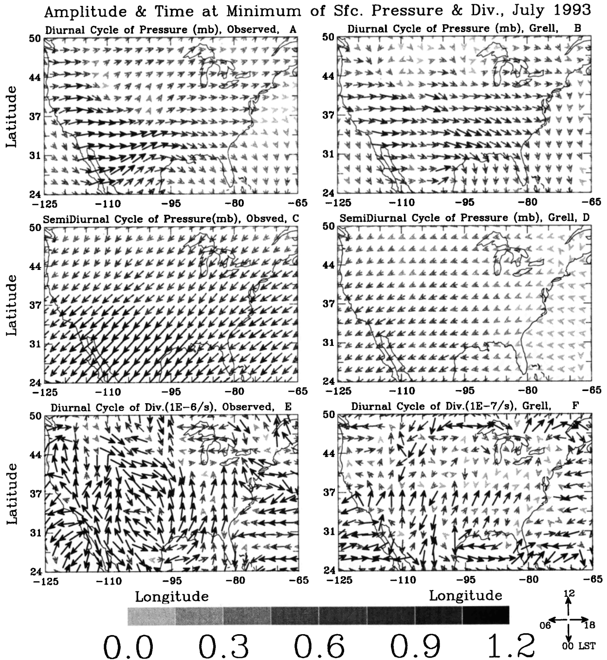
Figure 16. Vector plots of the diurnal (top row) and semidiurnal (middle row) harmonics in observed (left column) and simulated (right column) with the Grell scheme surface pressure, and the magnitude of the diurnal maximum convergence and its time of occurrence (bottom row) which result from the two pressure harmonics. The vector length and grey levels represent the amplitude (mbar) of the pressure harmonics or the magnitude of the maximum convergence ( 10^{-6} \text{ s}^{-1} for the observed, E , and 10^{-7} \text{ s}^{-1} for the Grell scheme, F ). The arrow direction denotes the local time of minimum values for the pressure harmonics and of maximum values for the convergence (same clock definition as in Figure 3). Plots for the Kuo and CCM3 schemes are similar to the Grell scheme.
