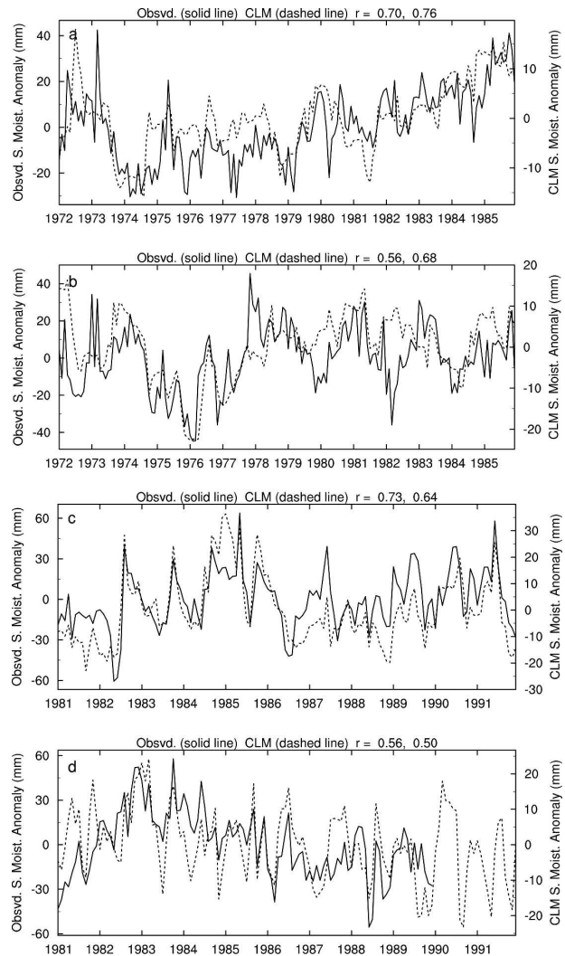
FIG. 14. Monthly anomaly time series of observed soil moisture content within the top 1-m depth (solid) averaged over (a) the former USSR region 1 ( 50^{\circ} – 55^{\circ}\text{N} , 70^{\circ} – 100^{\circ}\text{E} ), (b) region 2 ( 47.5^{\circ} – 55^{\circ}\text{N} , 45^{\circ} – 60^{\circ}\text{E} ), (c) east China ( 32.5^{\circ} – 35.0^{\circ}\text{N} , 110^{\circ} – 120^{\circ}\text{E} ), and (d) south China ( 22.5^{\circ} – 25.0^{\circ}\text{N} , 102.5^{\circ} – 110.0^{\circ}\text{E} ) compared with the CLM3-simulated values (dashed). Also shown on the top of each panel are (from left to right) the correlation coefficients ( r ) between the two anomaly curves and monthly time series with the annual cycle.
