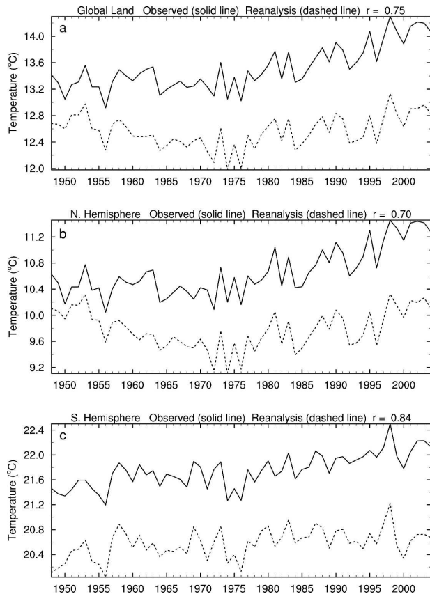
FIG. 3. Time series of annual surface air temperature averaged over global (60°S–75°N) and hemispheric land areas from surface observations (solid line) and the NCEP–NCAR reanalysis (dashed line). The observations are from CRU (Jones and Moberg 2003) with missing values being filled by the reanalysis temperature anomaly added to the CRU 1961–90 climatology.
