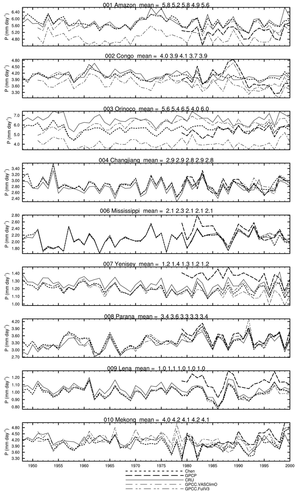
FIG. 1. Time series of annual precipitation averaged over world's major river basins based on five observational datasets: Chen et al. (2002), GPCP, CRU, and GPCC fixed-station (VASclimO) and all-station (FullV3) products. Also shown on the top of each panel are long-term means of these products in the above order.
