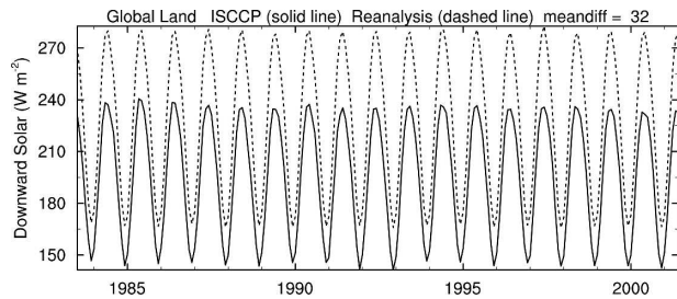
FIG. 6. Comparisons of monthly surface downward solar radiation averaged over global ( 60^{\circ}\text{S} – 75^{\circ}\text{N} ) land areas from the ISCCP-based radiation dataset (solid line; from Zhang et al. 2004) and the cloud-adjusted reanalysis radiation (dashed line) from July 1983 to June 2001. Also shown on the top of the panel is the mean difference (cloud-adjusted reanalysis minus ISCCP).
