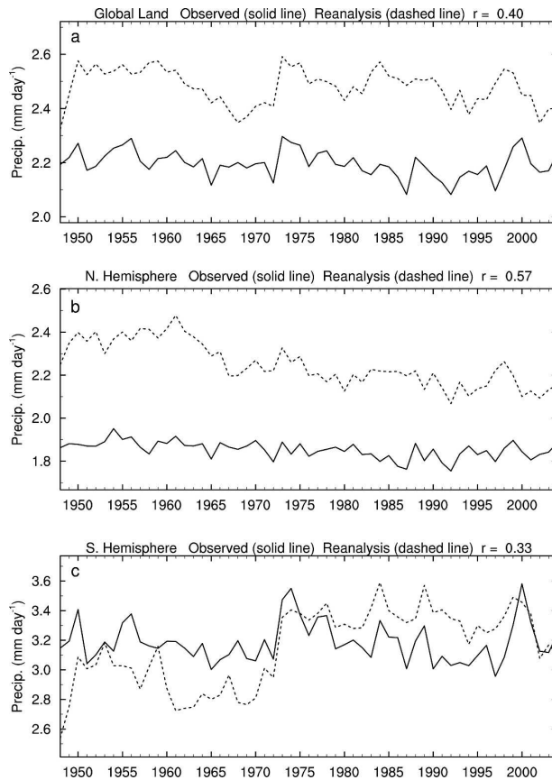
FIG. 2. Time series of annual precipitation averaged over global (60°S–75°N) and hemispheric land areas from rain gauge observations (solid line) and the NCEP–NCAR reanalysis (dashed line). The observations are derived from Chen et al. (2002) for 1948–96 and GPCP v2 (Adler et al. 2003) for 1997–2004 as described in the text.
