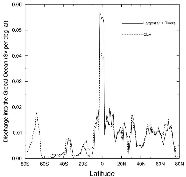
FIG. 10. Long-term-mean annual freshwater discharge (Sv) into the global oceans smoothed using a 5^{\circ} lat running mean from observation-based estimates (solid line; from Dai and Trenberth 2002) and the standard CLM3 simulation (dashed line).
