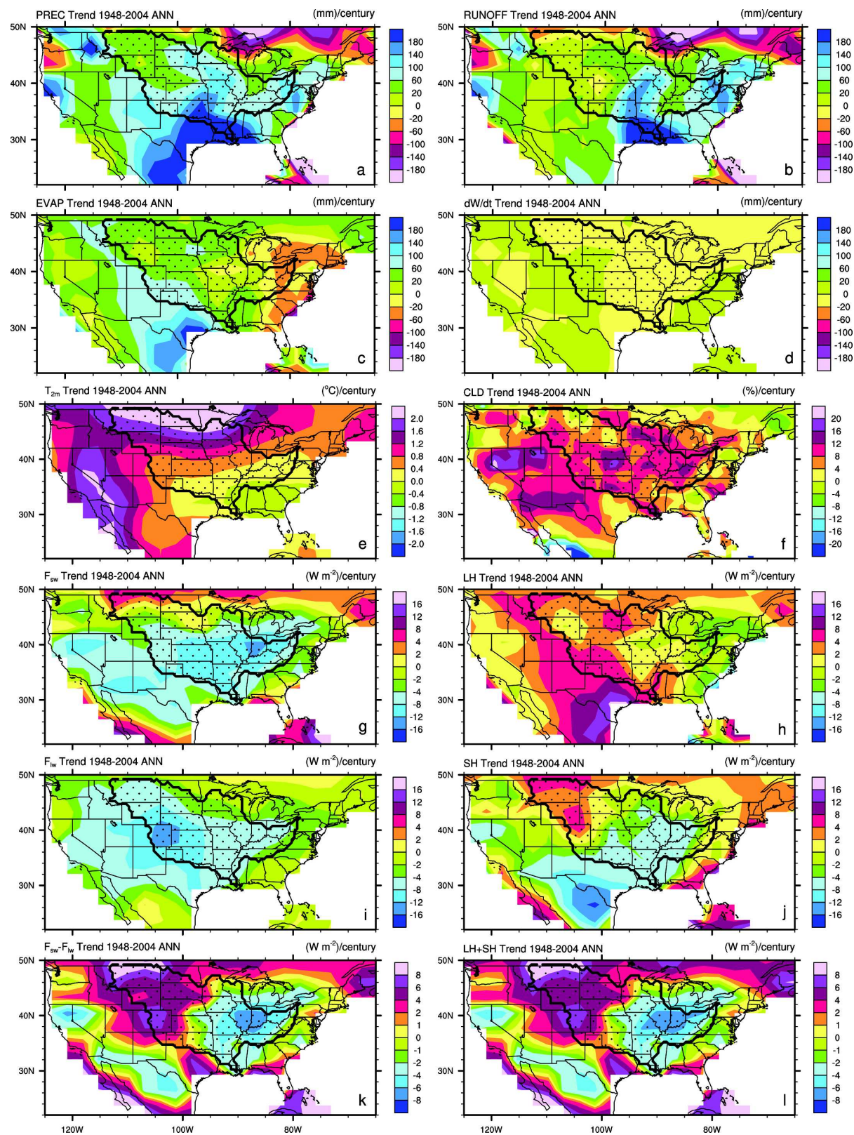
FIG. 5. Spatial distributions of the linear trend from October 1948 to September 2004 in annual (water year) (a) observed precipitation; CLM3-simulated (b) runoff, (c) evapotranspiration, and (d) change of water storage; (e) observed surface air temperature; (f) observed cloud amount; and CLM3-simulated (g) net shortwave radiation, (h) latent heat flux, (i) net longwave radiation, (j) sensible heat flux, (k) net radiative heating, and (l) net turbulent flux. The stippled area is the Mississippi basin with the dark line as the boundary.
