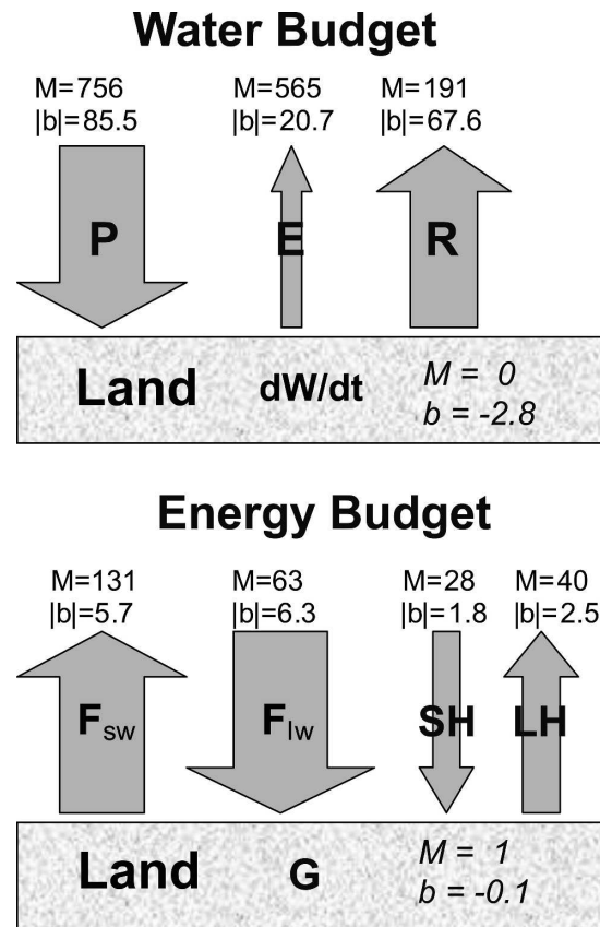
FIG. 6. Basin-averaged trends in the water and energy budget components for the Mississippi River basin: M is the long-term (1948–2004) annual (water year) mean (in mm for water components and W m -2 for energy components) and b is the annual linear trend during 1948–2004 (in mm century -1 for water components and W m -2 century -1 for energy components, proportional to arrow shaft width). Note that the downward arrow means that the flux increases the trend of dW/dt or G .
