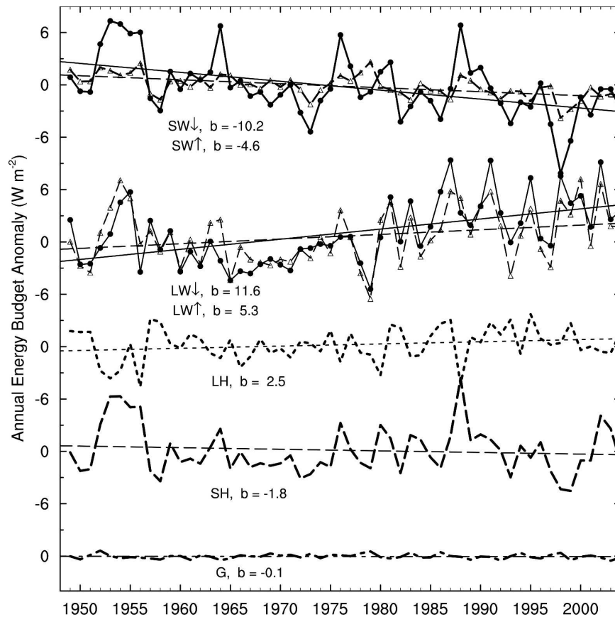
FIG. 3. Annual (water year) anomaly time series of surface energy budget components averaged over the Mississippi River basin and associated linear trends (straight lines: b is the slope, in \text{W m}^{-2} \text{ century}^{-1} ). Except for downward shortwave ( \text{SW}\downarrow , thick solid line with dots), which is derived from observed cloud cover, all other components are from the observation-constrained CLM3 simulation: upward shortwave ( \text{SW}\uparrow , thick dashed line with triangles), downward longwave ( \text{LW}\downarrow , thin solid line with dots), upward longwave ( \text{LW}\uparrow , thin dashed line with triangles), latent heat flux ( \text{LH} , short dashed line), sensible heat flux ( \text{SH} , long dashed line), and heat flux into the ground ( G , bottom line).
