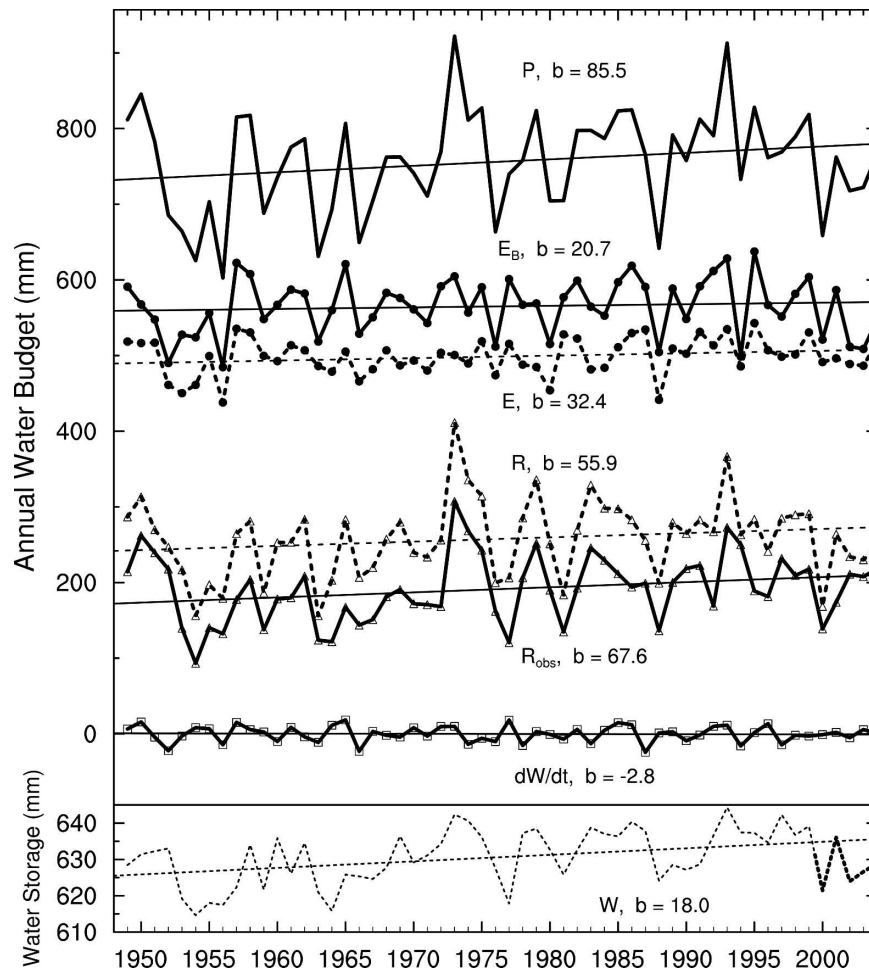
FIG. 1. Time series of annual (water year) surface water budget components averaged over the Mississippi River basin and associated linear trends (straight lines: b is the slope in \text{mm century}^{-1} ). Given are the observed basin precipitation ( P , solid line), runoff ( R_{\text{obs}} , solid line with triangles), the water budget-derived evapotranspiration ( E_B , solid line with dots), and CLM3-simulated runoff ( R , dashed line with triangles), evapotranspiration ( E , dashed line with dots), change of land water storage [ dW/dt , solid line with quadrangles; note that b for this quantity is d(dW/dt)/dt ] and (bottom) land water storage ( W , dashed line; b is the trend in W ).
