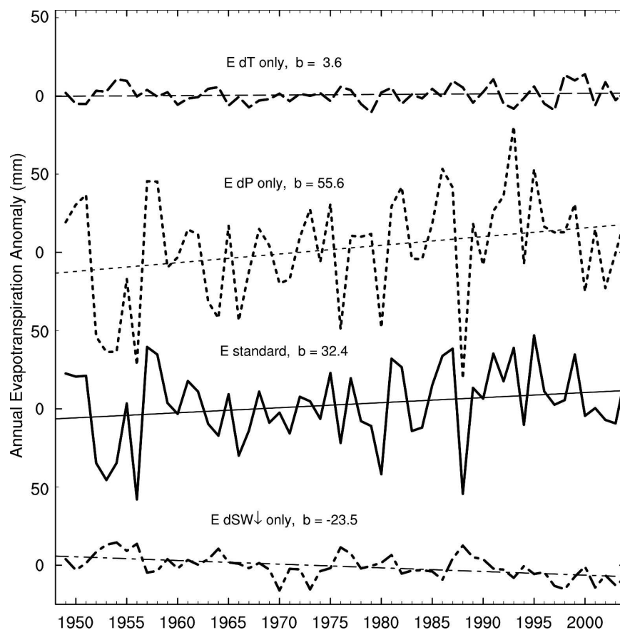
FIG. 4. Anomaly time series of annual (water year) surface evapotranspiration averaged over the Mississippi River basin and associated linear trends (straight line: b is the slope, in \text{mm century}^{-1} ) from CLM3 sensitivity experiments: Standard = all forcing run (solid line); dP only = with only precipitation changing and other forcings fixed (short dashed line); dT only = run with only temperature changing (long dashed line); dSW\downarrow only = with only downward solar radiation (i.e., cloud) changing (bottom line).
