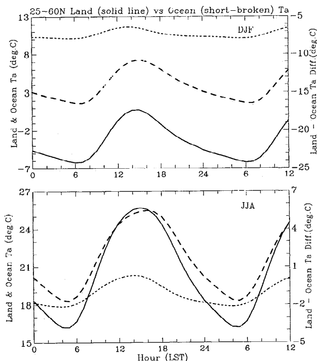
Figure 16. Observed mean surface air temperature ( ^{\circ}\text{C} ) during DJF (top) and JJA (bottom) averaged at each local time over the land (solid curve) and oceanic (short-dashed curve) areas from 25^{\circ}\text{N} to 60^{\circ}\text{N} . The long-dashed curve is the land minus ocean difference of surface air temperature (on the right ordinate). The temperature data are from the same data sets as for surface winds and have a coverage similar to Figure 1.
