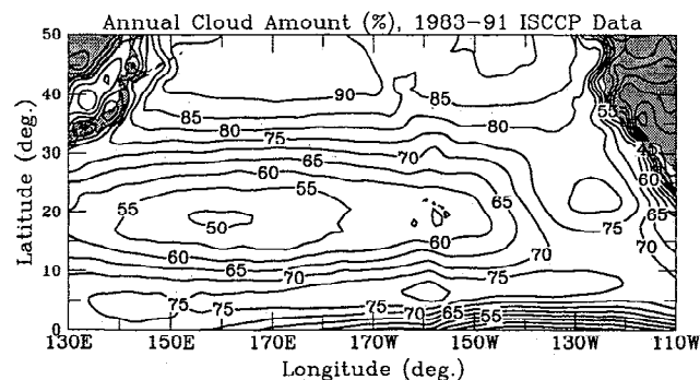
Figure 17. Satellite-observed mean (1983–1991) annual total cloud amount (%) over the northern Pacific derived from the International Satellite Cloud Climatology Project (ISCCP) data sets [Rossow and Schiffer, 1991].
