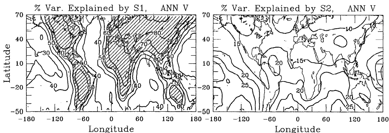
Figure 7. Percentage of the mean daily variance explained by the diurnal (left) and semidiurnal (right) harmonics of the annual mean surface wind speed. Plots for the zonal and meridional wind components are similar to those of wind speed.
