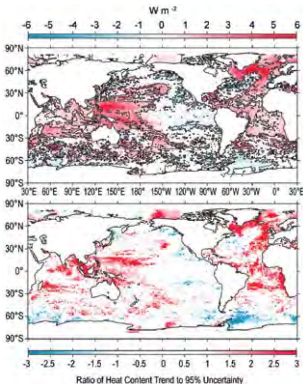
FIG. 3.7. (a) Linear trend from 1993 to 2010 of the combined satellite altimeter and in situ ocean temperature data estimate of upper (0 m–700 m) ocean heat content anomaly OHCA ( \text{W m}^{-2} ) analyzed following Willis et al. (2004). Areas with statistically significant trends are outlined in black. (b) Signed ratio of the linear trend to its 95% uncertainty estimate, with increasing color intensity showing regions with increasingly statistically significant trends.
