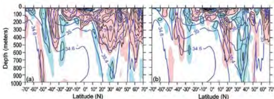
FIG 3.16. (a) Zonal mean 2010 salinity anomaly vs. latitude and depth for the Atlantic Ocean. (b) Salinity anomaly 2010 minus 2009 vs. latitude and depth for the Atlantic Ocean. For both plots blue shading is for areas of negative (fresh) anomaly < -0.01 . Red shading is for areas of positive (salty) anomaly > 0.01 . Contour interval shown for anomalies is 0.02. In the background (thick blue contours) is the zonally averaged climatological mean salinity. Contour intervals for the background are 0.4. All values are on the Practical Salinity Scale. WOA09 was used as the reference climatology for anomalies and for background means.
