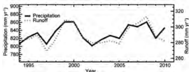
FIG. 2.24. Annual continental precipitation from GPCC full product extended with the monitoring product for 2010 and the corresponding water balance model-simulated runoff using NCEP air temperature forcing.
