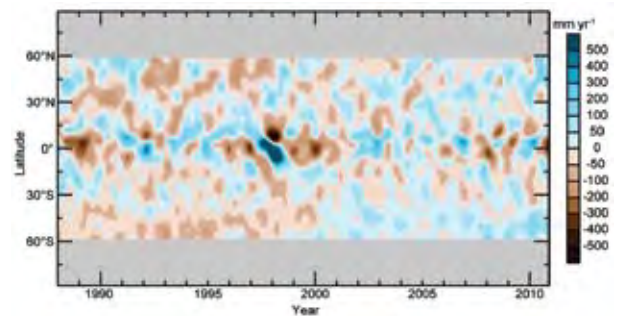
FIG. 2.19. RSS measurements of monthly mean precipitation anomalies over ocean by latitude. The anomalies are relative to a base period of 1988–2010. Gray areas indicate regions where data are unavailable.
