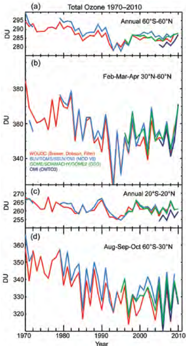
FIG. 2.58. Annual mean total ozone time series of ground-based measurements combining Brewer, Dobson, and filter spectrometer data (red; Fioletov et al. 2002), merged BUUV/SBUV/TOMS/OMI MOD V8 (blue; Frith et al. 2004), GOME1/SCIAMACHY/GOME2 GSG (green; Weber et al. 2007), and OMI DMTO3 (OMI-TOMS; Kroon et al. 2008; McPeters et al. 2008) satellite data in the (a) 60°S–60°N, (b) 30°N–60°N, (c) 20°S–20°N, and (d) 30°S–60°S zonal bands.
