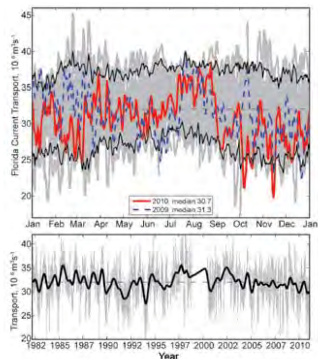
FIG. 3.24. (top) Daily estimates of the transport of the Florida Current during 2010 (red solid line) compared to 2009 (dashed blue line). The daily values of the Florida Current transport for other years since 1982 are shown in light gray and the 90% confidence interval of daily transport values computed from all years is shown in black (solid line); the long-term annual mean is dashed black. The mean transport in 2010 of 30.7 \pm 1.5 Sv decreased for the fourth year in a row, below the long-term mean for the daily values of the Florida Current transport ( 32.2 Sv). (bottom) Daily estimates of the Florida Current transport for the full time series record (light gray), a smoothed version of transport (heavy black line; using a 30-day running mean six times) and the mean transport for the full record (dashed black).
