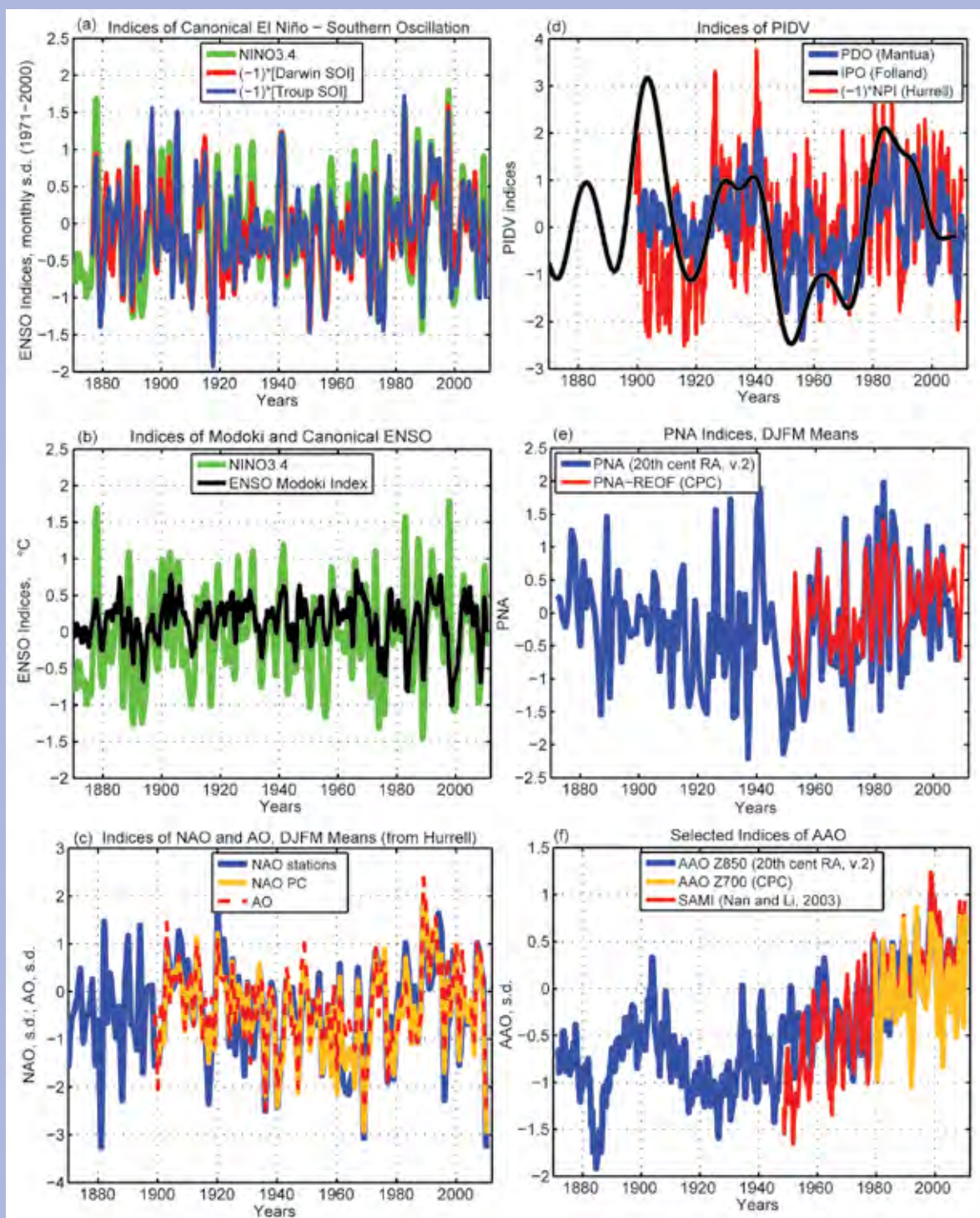
FIG. I.3. Selected indices of climate variability, as specified in Table 2.3, for the period 1880–2010, grouped into categories: (a) Canonical El Niño–Southern Oscillation (ENSO); (b) the Modoki variant of ENSO; (c) Northern Hemisphere oscillations (NAO, AO, NAM) for the boreal cold season; (d) indices of Pacific Interdecadal Variability; (e) Pacific–North American indices for the boreal cold season; (f) Southern
