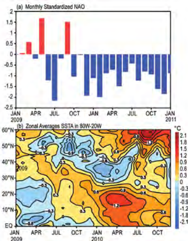
FIG. 3.3. (a) Monthly standardized NAO index from http://www.cpc.ncep.noaa.gov . (b) Time-Latitude section of SST anomalies averaged between 80°W and 20°W. SSTs are the monthly fields temporally averaged from the weekly 1° OISST.
