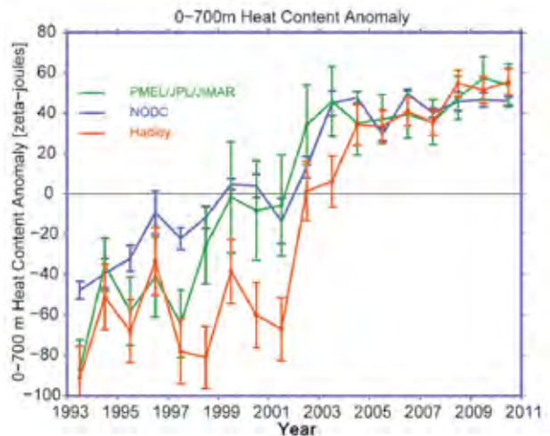
FIG. 3.8. Time series of annual average global integrals of in situ estimates of upper (0 m–700 m) OHCA ( 10^{21} J, or ZJ) for 1993–2010 with standard errors of the mean. The NODC estimate ( http://www.nodc.noaa.gov/OC5/indprod.html ) follows Levitus et al. (2009) with uncertainties derived solely from the variance of quarterly estimates of OHCA. The PMEL/JPL/JIMAR estimate is a weighted integral (Lyman and Johnson, 2008) using Argo and WOD 2009 (Johnson et al. 2009) data relative to a 2004–10 climatology with the Wijffels et al. (2008) Table 2 XBT bias adjustments applied and no XBT data after 2005 with error estimate methodology following Lyman et al. (2010). The Hadley estimate applies XBT bias adjustments from Table 1 of Wijffels et al. (2008) to the EN3 dataset (Ingleby and Huddleston 2007; http://www.metoffice.gov.uk/hadobs ) also relative to a 2004–10 climatology and is computed from estimates of monthly OHCA following Palmer et al. (2007) and Palmer and Brohan (2010) with error estimate methodology similar to Rayner et al. (2006) but adding uncertainty in the XBT bias correction. For comparison, all estimates have been individually offset (vertically on the plot), first to their individual 2004–10 means (the best sampled time period), and then to their collective 1993–2010 mean (the record length).
