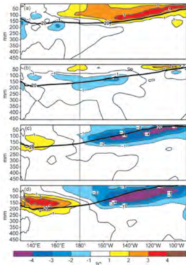
FIG. 4.3. Equatorial depth-longitude section of ocean temperature anomalies ( ^{\circ}\text{C} ) averaged between 5^{\circ}\text{N} and 5^{\circ}\text{S} during (a) DJF 2009/10, (b) MAM 2010, (c) JJA 2010, and (d) SON 2010. The 20^{\circ}\text{C} isotherm (thick solid line) approximates the center of the oceanic thermocline. The data are derived from an analysis system that assimilates oceanic observations into an oceanic global circulation model (Behringer et al. 1998). Anomalies are departures from the 1971–2000 period monthly means.
