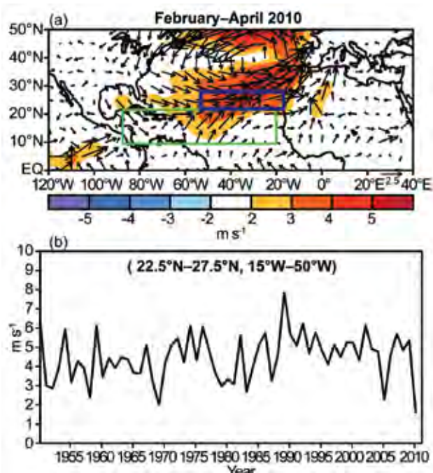
FIG. 4.14. (a) Map of February–April 2010 1000-hPa anomalous wind speed (shaded, \text{m s}^{-1} ) and vector winds, and (b) time series of consecutive area-averaged total wind speed ( \text{m s}^{-1} ) at 1000 hPa in the area bounded by 22.5^{\circ}\text{N} – 27.5^{\circ}\text{N} , 15^{\circ}\text{W} – 50^{\circ}\text{W} (blue box in panel a). Green box in (a) denotes the Main Development Region.
