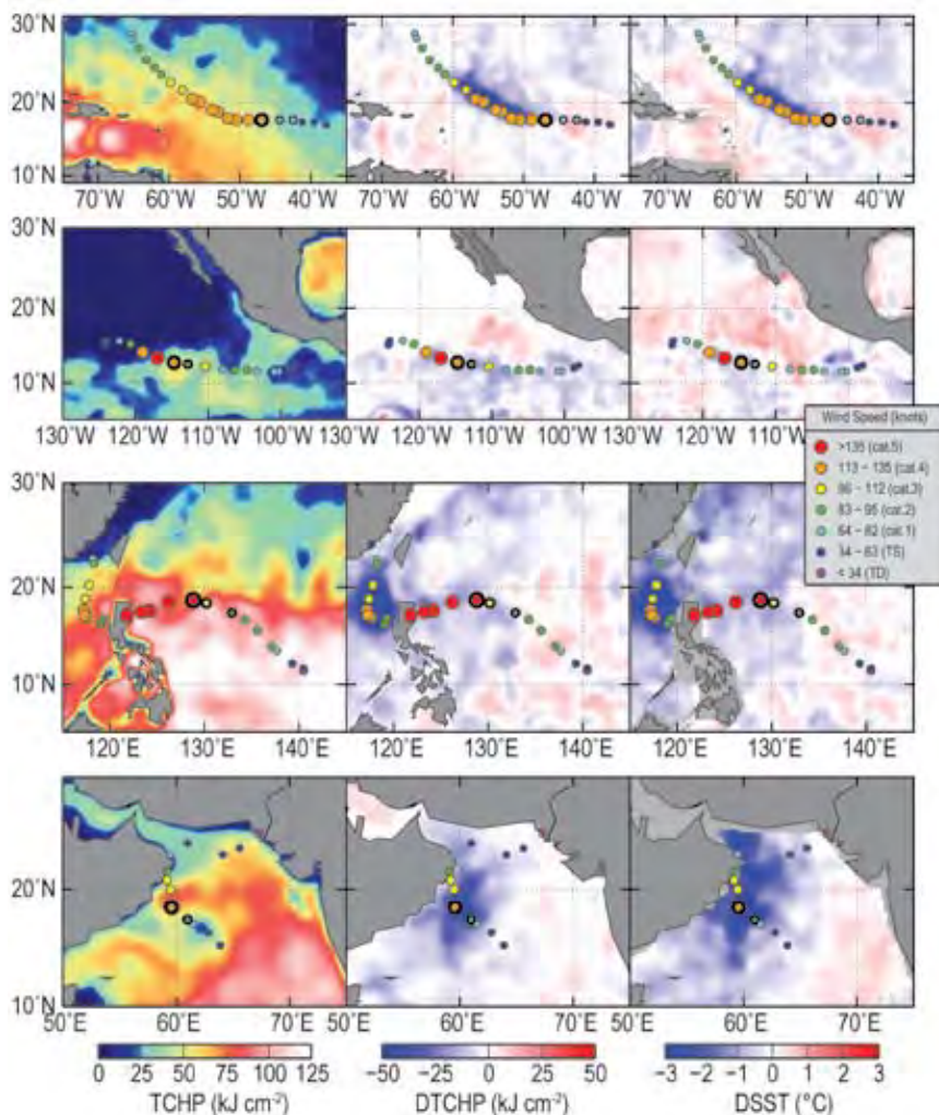
FIG. 4.29. (left) Tropical Cyclone Heat Potential (TCHP) and surface cooling given by the difference between post- and pre-storm values of (center) tropical cyclone heat potential and (right) sea surface temperature for (from top to bottom) Hurricane Igor, Hurricane Celia, Typhoon Megi, and Cyclone Phet.
