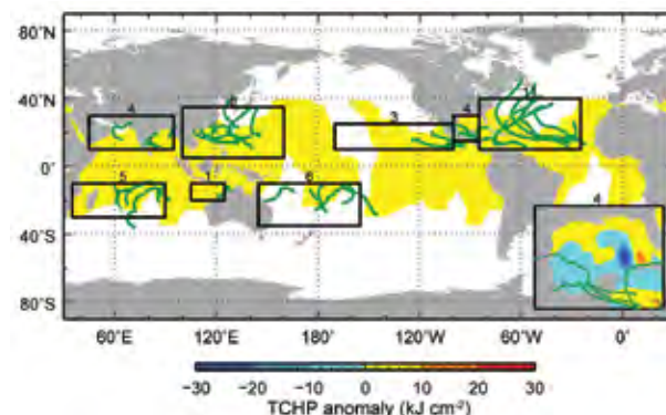
FIG. 4.27. Global anomalies of Tropical Cyclone Heat Potential (TCHP) corresponding to 2010 computed as described in the text. The boxes indicate the seven regions where tropical cyclones occur: from left to right, Southwest Indian, North Indian, West Pacific, Southeast Indian, South Pacific, East Pacific, and North Atlantic (shown as Gulf of Mexico and tropical Atlantic separately). The green lines indicate the trajectories of all tropical cyclones reaching at least Category 1 [one-minute average wind \geq 64 kts (33 m s -1 )] and above during November 2009–April 2010 in the Southern Hemisphere and June–November 2010 in the Northern Hemisphere. The numbers above each box correspond to the number of Category 1 and above cyclones that travel within each box. The Gulf of Mexico conditions during June–November 2010 are shown in detail in the insert shown in the lower right corner.
