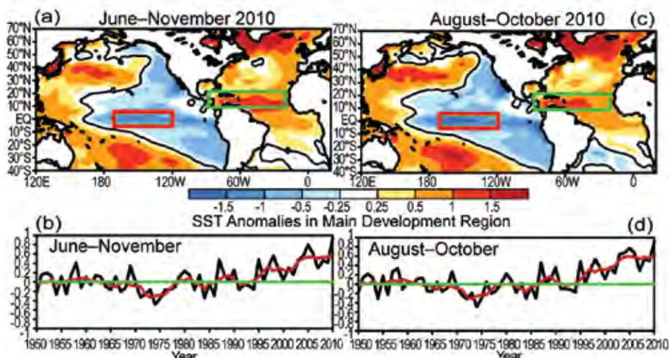
FIG. 4.13. (Top) Sea surface temperature (SST) anomalies ( ^{\circ}\text{C} ) during (a) June–November 2010 and (c) August–October 2010. (Bottom) Time series of consecutive area-averaged SST anomalies in the Main Development Region (MDR) during (b) June–November, and (d) August–October. Red line shows the corresponding five-year running mean. Green boxes in (a) and (c) denote the MDR. Anomalies are departures from the ERSST-V3b (Smith et al. 2008) 1971–2000 period monthly means.
