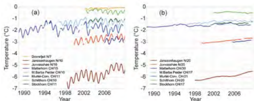
FIG. 2.28. Observed subsurface temperatures at (a) 10 m and (b) 20 m depth for selected boreholes in mountain permafrost: the sites of the PACE transect, the Matterhorn and M.d. Barba Peider sites in Switzerland, and Dovrefjell in Norway. Data for Swiss sites are provided by PERMOS, and for Norwegian sites by the Norwegian Meteorological Institute. [Modified from Haeblerli et al. (2010, figure 4).]
