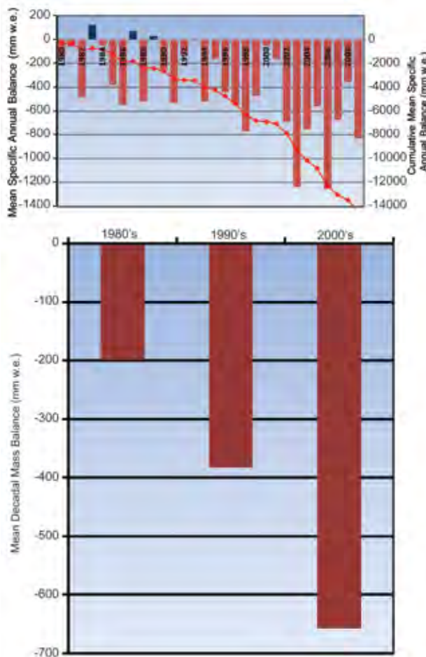
FIG. 2.60. The (top) annual mean and cumulative annual mean balance and (bottom) decadal mean cumulative specific mass balance (mm w.e.) reported for the 30 reference glaciers to the WGMS.
