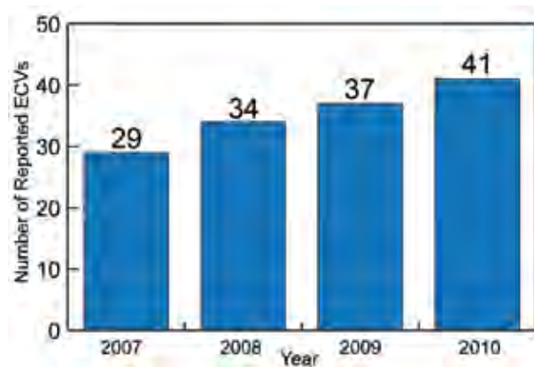
FIG. 1.1. Number of fully or partially monitored Essential Climate Variables (ECVs) reported in the annual State of the Climate editions since 2007. Atmospheric surface water vapor, atmospheric perfluorocarbons, oceanic subsurface salinity, and terrestrial lake levels have been introduced in this current edition.
