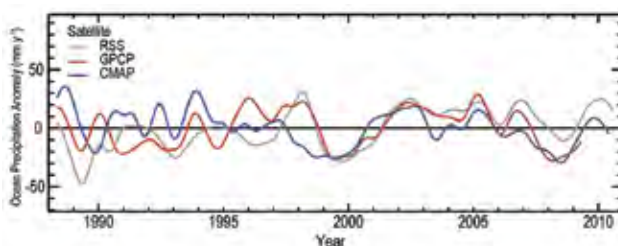
FIG. 2.18. Global average precipitation annual smoothed anomalies over ocean from satellites. All datasets are shown relative to a 1988–2010 base period.
