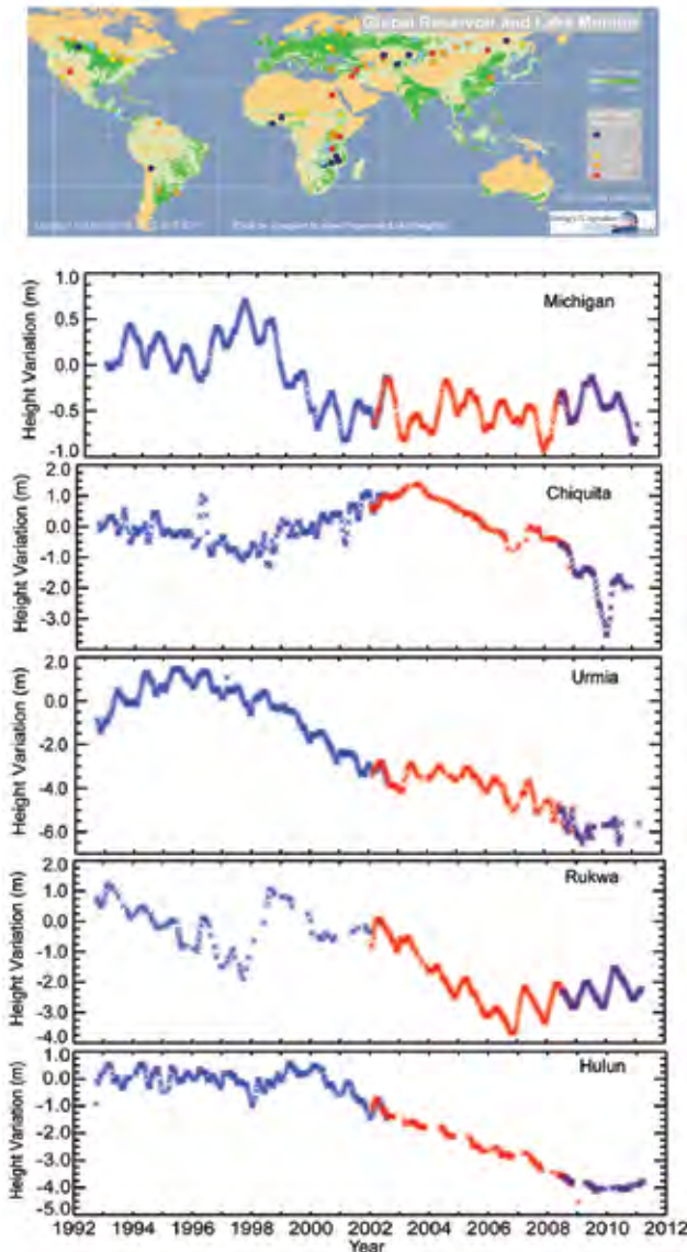
FIG. 2.36. (Top) Map showing the near real time lake level status of ~70 lakes with respect to a short-term mean (1992–2002). Red depicts low water drought and navy depicts high water. (Bottom) Examples of lake level time series for the United States (Michigan), Argentina (Chiquita), Iran (Urmia), Tanzania (Rukwa), and China (Hulun). (Courtesy of the USDA/FAS CropExplorer, http://www.pecad.fas.usda.gov/cropexplorer/global_reservoir/index.cfm )
