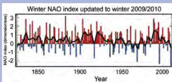
FIG. 7.37. Time series of winter North Atlantic Oscillation (NAO) Index (after Jones et al. 1997, December–March average). (Image from http://www.cru.uea.ac.uk/~timol/datapages/naoi.htm , updated 28 Jan 2011.)
