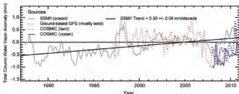
FIG. 2.14. Anomaly time series of total column water vapor both from SSM/I, ground-based GPS, and COSMIC (1997–2009 base period). The COSMIC ocean anomalies are calculated relative to an SSM/I climatology for 1997–2009. The COSMIC land anomalies are calculated only at the locations of GPS ground stations, and are relative to a 1997–2009 ground-based GPS climatology. The time series have been smoothed to remove variability on time scales shorter than six months.
