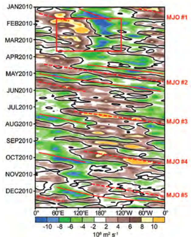
FIG. 4.7. Time-longitude section for 2010 of anomalous 200-hPa velocity potential ( \times 10^6 \text{ m}^2 \text{ s}^{-1} ) averaged between 5°N and 5°S. For each day, the period mean is removed prior to plotting. Green (brown) shading highlights likely areas of anomalous divergence and rising motion (convergence and sinking motion). Red lines and labels highlight the main Madden Julian Oscillation episodes. Anomalies are departures from the 1971–2000 base period daily means.
