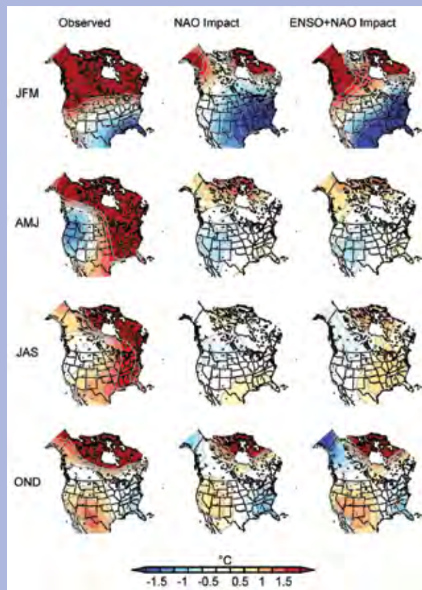
FIG. 7.5. (Left panels) North American surface air temperature departures ( ^{\circ}\text{C} ) during 2010 for winter (JFM), spring (AMJ), summer (JAS), and fall (OND) based on NASA gridded departures (based on 1961–90); (middle panels) surface temperature signal ( ^{\circ}\text{C} ) attributable to the state of the 2010 North Atlantic Oscillation (NAO); (right panels) surface temperature signal ( ^{\circ}\text{C} ) attributable to the combined effects of the state of NAO and ENSO. The NAO signal is calculated by regressing the monthly surface temperatures upon the Climate Prediction Center's NAO index time series for 1950–2009, and the 2010 anomalies are derived by multiplying the regression pattern by the observed 2010 standardized NAO index for each season. The ENSO signal is calculated by regressing the monthly surface temperatures upon a Nino-3.4 SST index time series for 1950–2009 and then scaling by the observed 2010 index values of Nino-3.4 SSTs. The combined 2010 anomalies are derived by adding the separate NAO and ENSO signals. All data used in regression were detrended. (Source: NOAA/ESRL-PSDI/GISS.)
