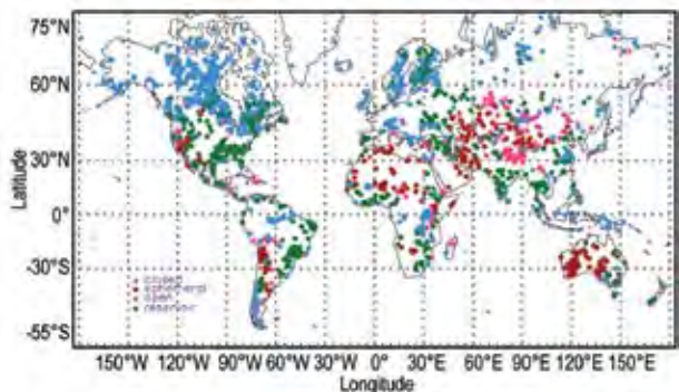
FIG. 2.37. Global location of large (> 100 km 2 ) lakes; closed (pink), ephemeral (red), open (blue), and reservoirs (green). Based on Birkett and Mason (1995).
