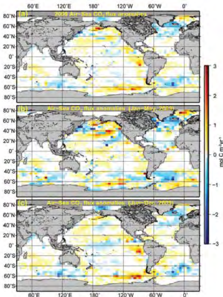
FIG. 3.31. Global distributions of air-sea \text{CO}_2 flux anomalies for the full year of 2009 (a) January to May, (b) and June to December, and (c) compared to the 28-year mean values for the corresponding months as calculated from the Park et al. (2010) approach. Positive values indicate less uptake or more release of \text{CO}_2 by the ocean 1 . The results for air-sea \text{CO}_2 flux anomalies are for the calendar year 2009 due to lags in data availability.
