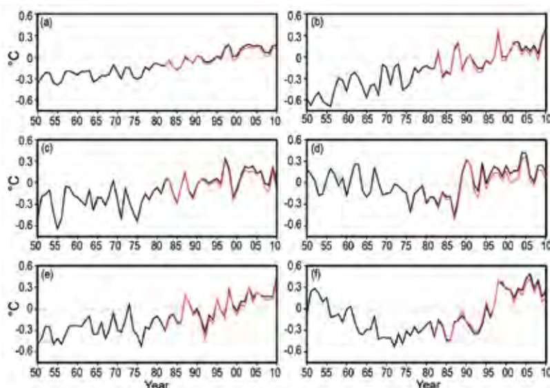
FIG. 3.4. Yearly mean SST anomalies ( ^{\circ}\text{C} ) from ERSST in 1950–2010 (black) and OISST in 1982–2010 (red) averaged in the (a) global ocean, (b) tropical Indian Ocean, (c) tropical Pacific, (d) North Pacific, (e) tropical Atlantic, (f) North Atlantic.
