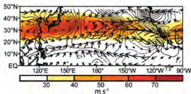
FIG. 4.6. DJF 2009/10: Total 200-hPa wind speed ( \text{m s}^{-1} , shaded), anomalous wind vector, and anomalous horizontal wind speed tendency ( \text{d}/\text{dt} ) (contours, interval is 1 \times 10^{-4} \text{ m s}^{-2} ). Solid (dashed) contours show anomalous speed acceleration (deceleration), where
