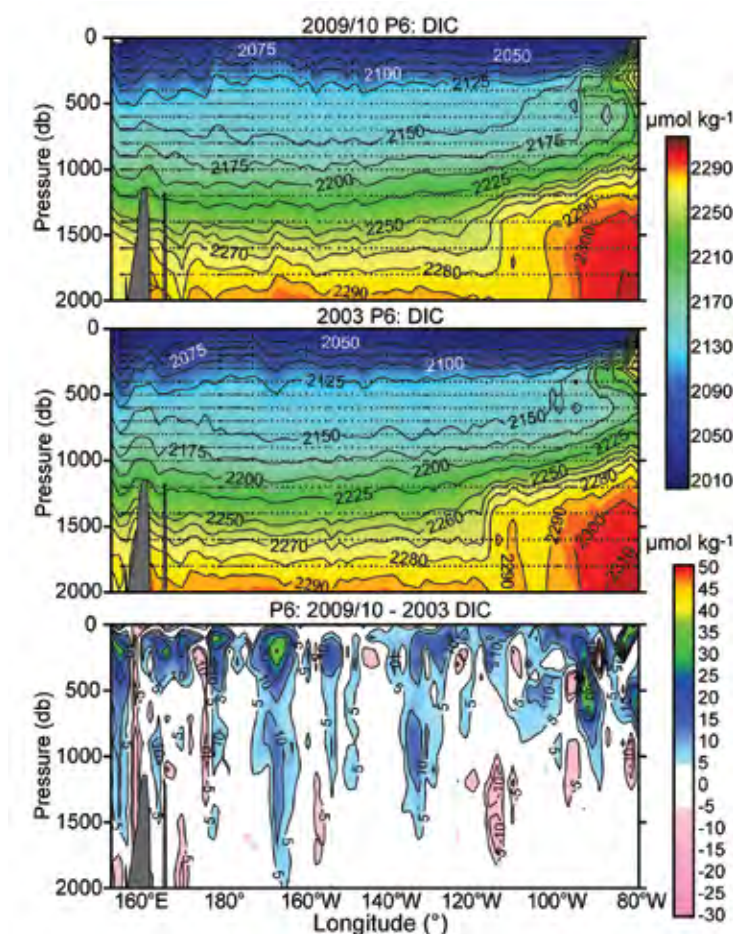
FIG. 3.34. Sections of dissolved inorganic carbon (μmol kg -1 ) nominally along 32°S in 2009/10 conducted as part of the U.S. CLIVAR/CO 2 Repeat Hydrography Program (top) and 2003 BEAGLE cruise conducted by the Japan Agency for Marine-Earth Science and Technology (middle). Black dots show sample locations. The bottom section shows the DIC change (μmol kg -1 ) between the two cruises (2009/10 minus 2003).
