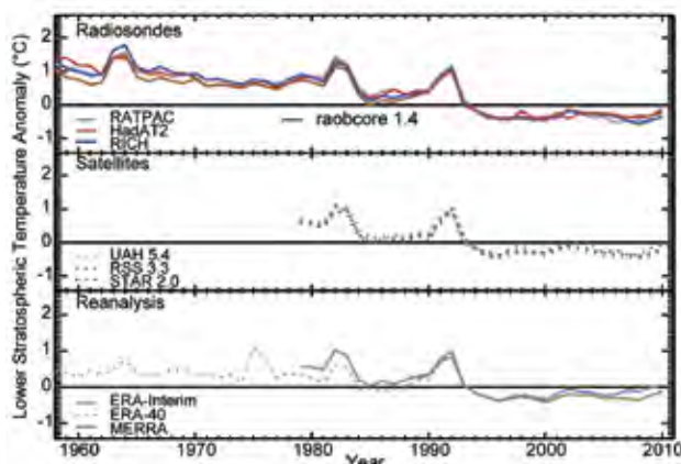
FIG. 2.7. Global average lower stratospheric temperature annual anomalies for the MSU 4 (or equivalent) layer. Radiosonde [HadAT2 (Thorne et al. 2005–465 day, 384 night stations), RATPAC (Free et al. 2005–85 stations), RAOBCORE 1.4 (Haimberger 2007–1184 stations) and RICH (Haimberger et al. 2008–1184 stations)] and Satellite [UAHv5.4 (Christy and Norris 2009), RSSv3.3 (Mears and Wentz 2009) and STAR 2.0 (Zou et al. 2009)] datasets use the 1981–2010 base period. ERA-40 uses the 1961–90 base period and all other reanalysis datasets use the 1989–2008 base period. All time series have been adjusted such that they give a mean of zero over the common period 1989–2001 to aid comparison.
