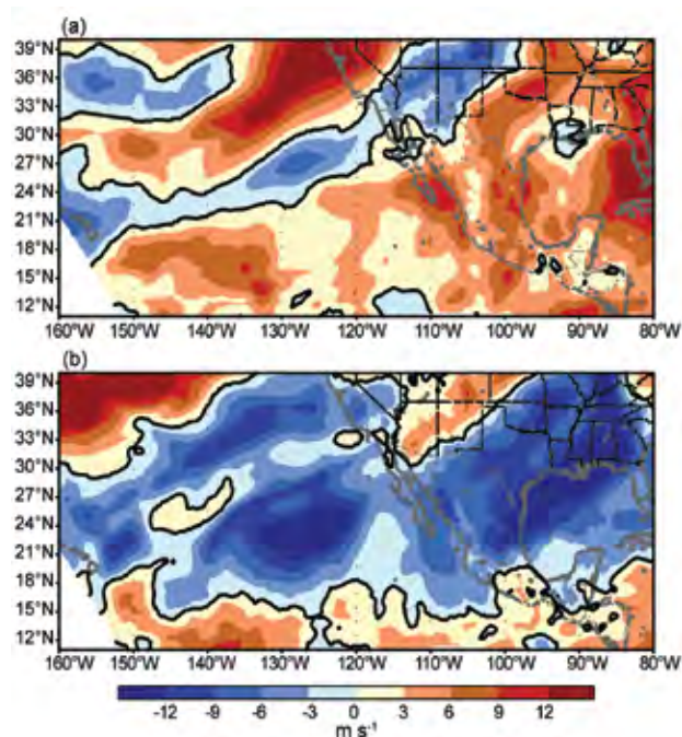
FIG. 4.21. The 200 hPa–850 hPa vertical wind shear anomalies ( \text{m s}^{-1} ) averaged over (a) June–August 2010 and (b) September–November 2010, with anomalies determined relative to the 1979–2004 base period mean. [Source: North American Regional Reanalysis (NARR) dataset, provided by the NOAA National Operational Model Archive and Distribution System.]
