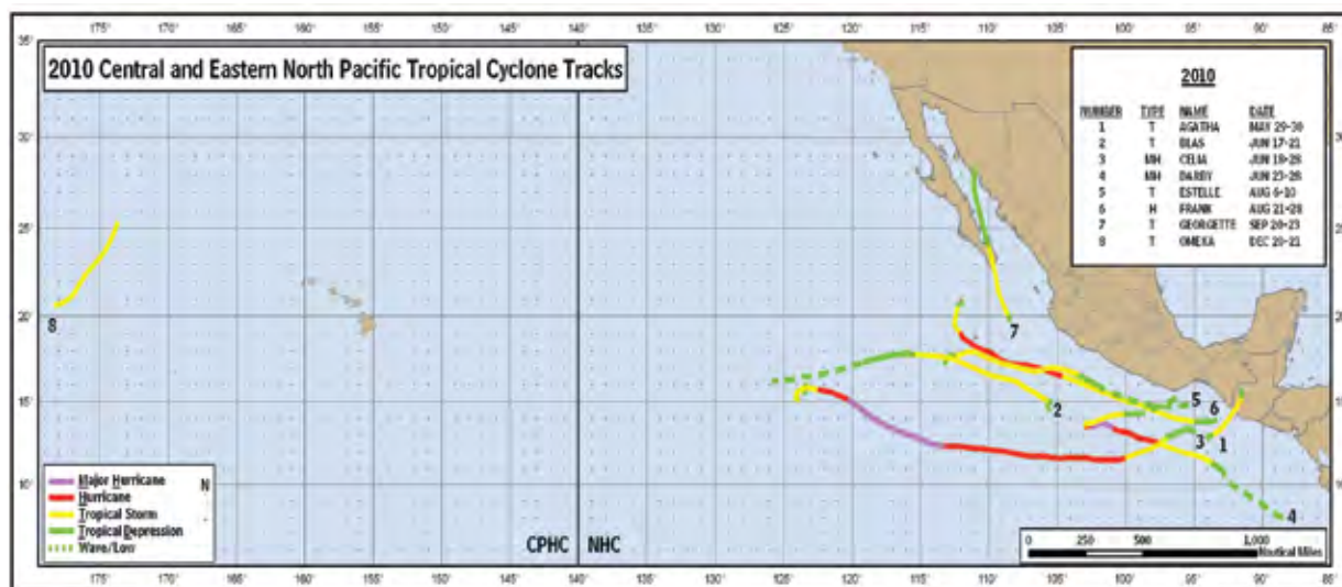
FIG. 4.19. Storm track map for the Eastern North Pacific hurricane basins, including all tropical cyclones that occurred in the Eastern North Pacific and Central North Pacific basins [Source: NOAA's National Hurricane Center (NHC) and Central Pacific Hurricane Center (CPHC)]. Tracks are color coded by intensity (wave/low, tropical depression, tropical storm, hurricane, and major hurricane). Also shown is the delineation of the forecast area of responsibility at 140°W between NOAA's NHC and CPHC.
