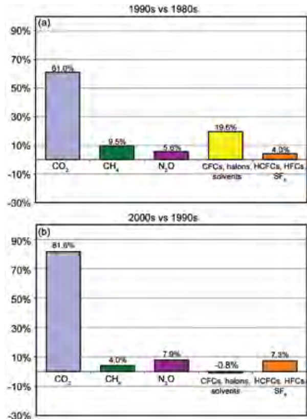
FIG. 2.53. Average relative contributions to changes in direct radiative forcing due to various trace gases through three decades. For example, comparing decadal averages, changes in \text{CO}_2 are responsible for 61% of the change in radiative forcing between the 1980s and 1990s.
