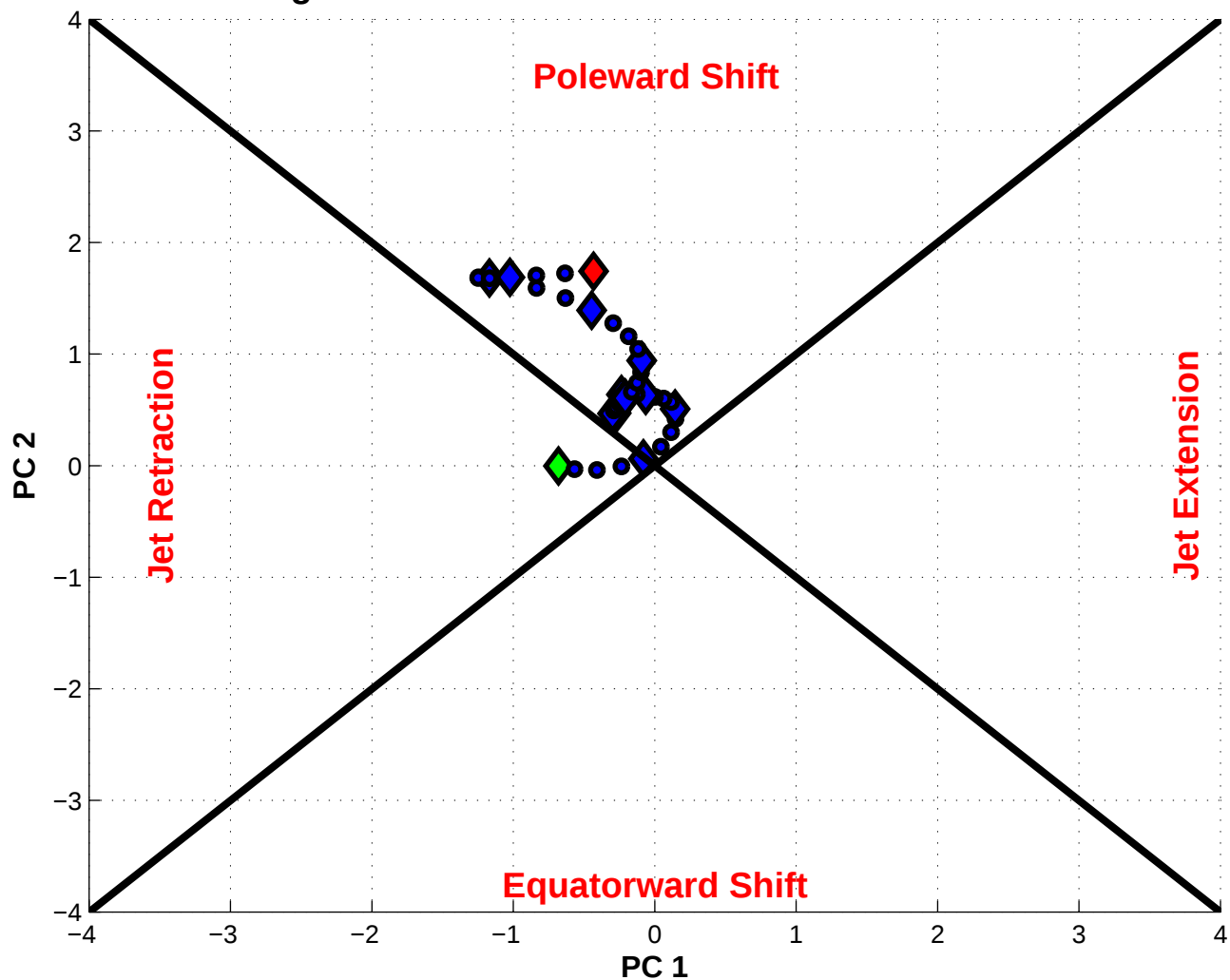
NPJ Phase Diagram valid 1800 UTC 03 Dec 2001 – 1200 UTC 15 Dec 2001
