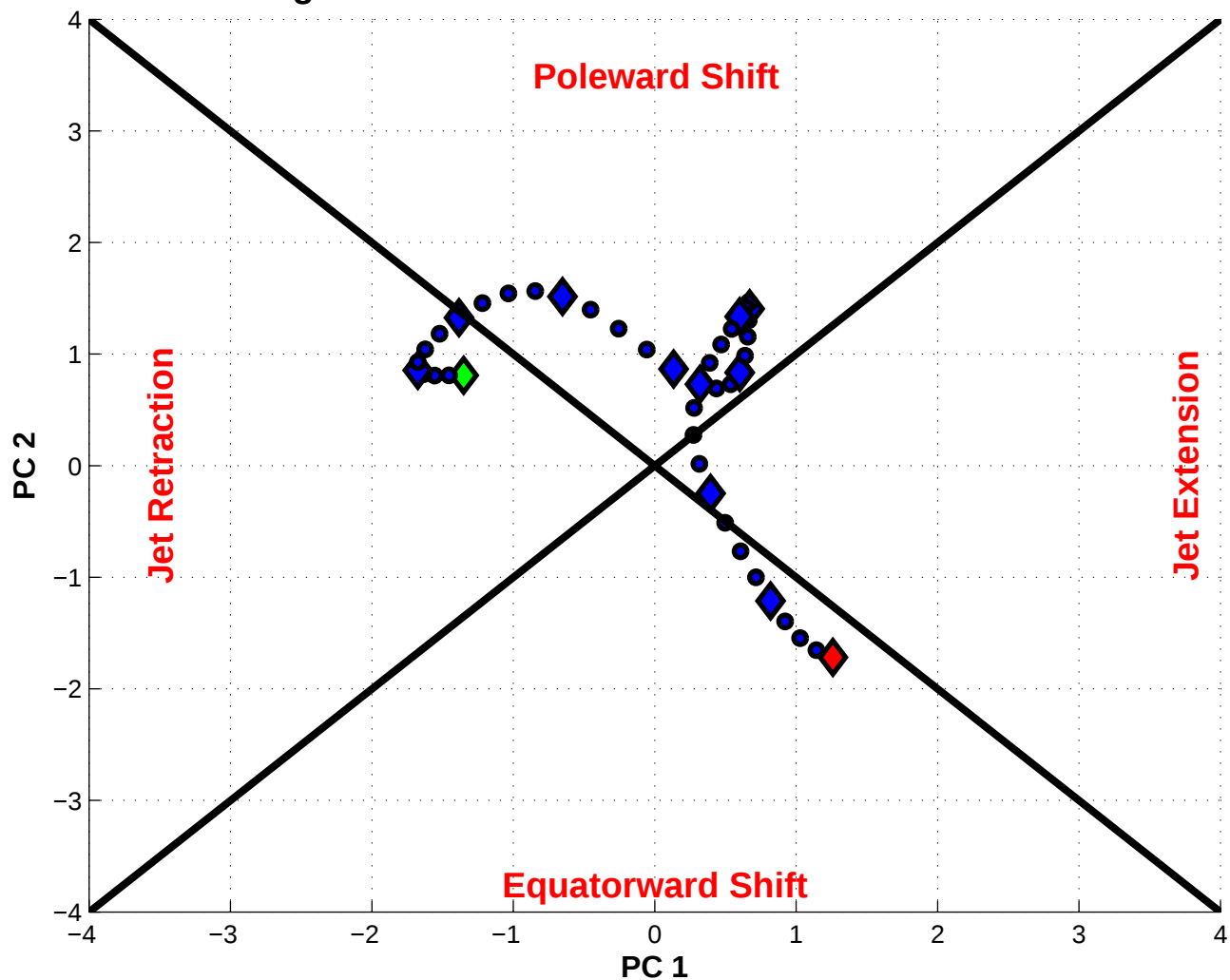
NPJ Phase Diagram valid 0600 UTC 06 Mar 1990 – 0600 UTC 17 Mar 1990
