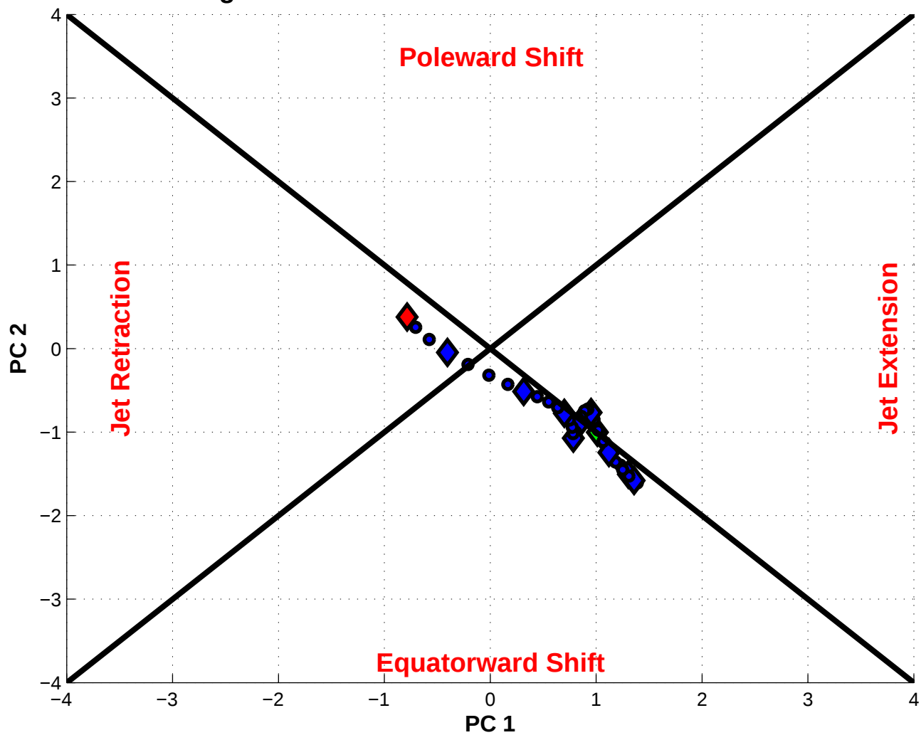
NPJ Phase Diagram valid 0600 UTC 07 Feb 1991 – 0000 UTC 17 Feb 1991
