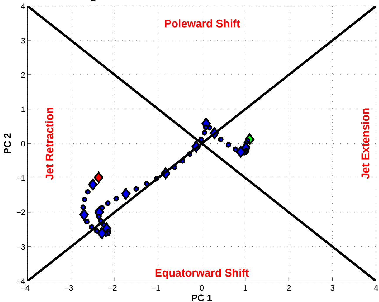
NPJ Phase Diagram valid 0000 UTC 08 Feb 1996 – 0600 UTC 20 Feb 1996
