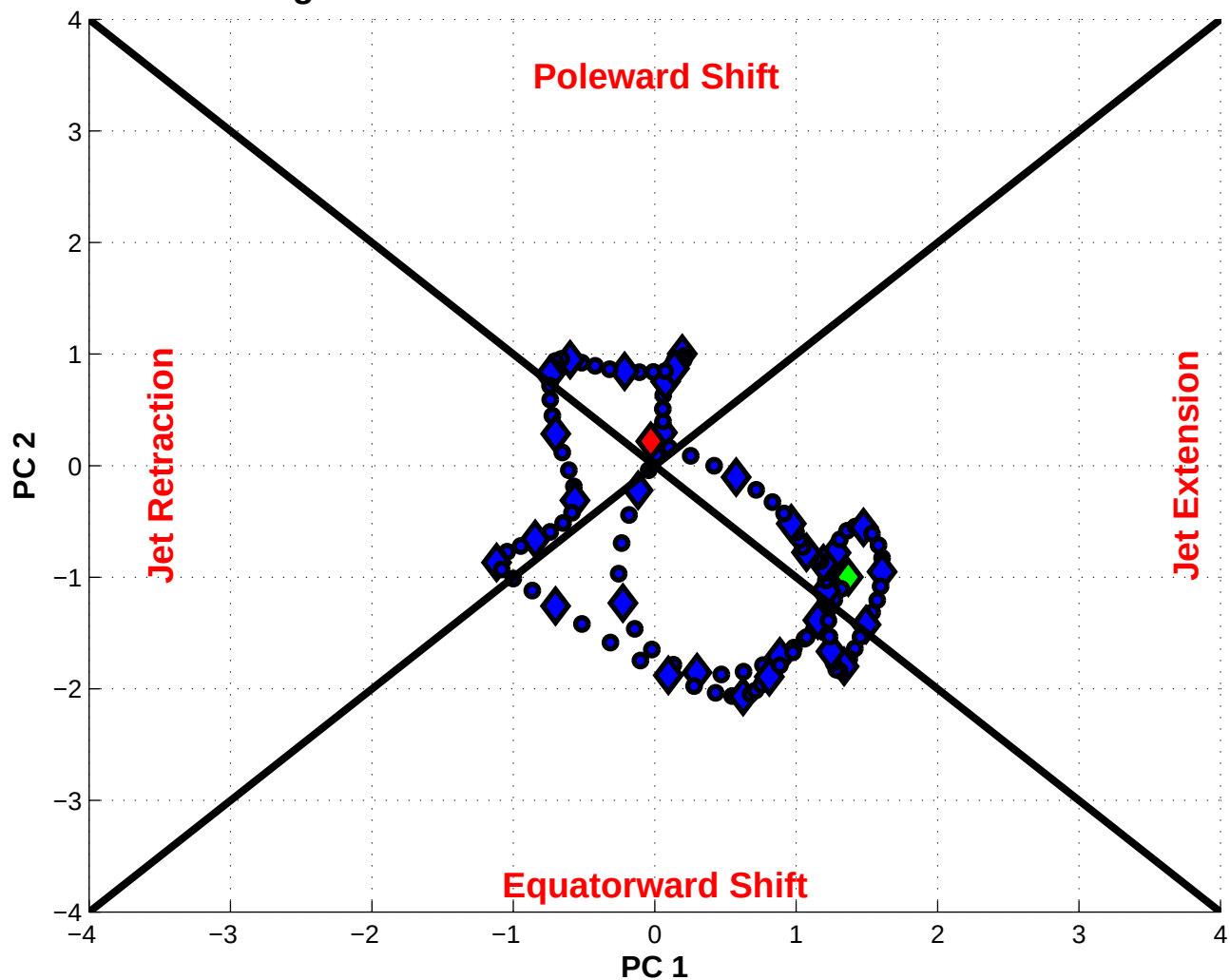
NPJ Phase Diagram valid 0000 UTC 09 Feb 1987 – 0000 UTC 14 Mar 1987
