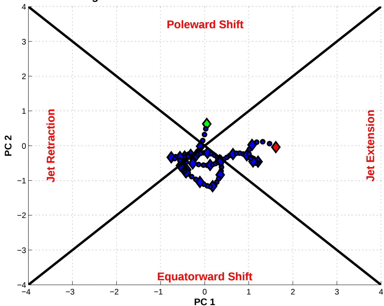
NPJ Phase Diagram valid 1800 UTC 09 Feb 2005 – 1800 UTC 06 Mar 2005
