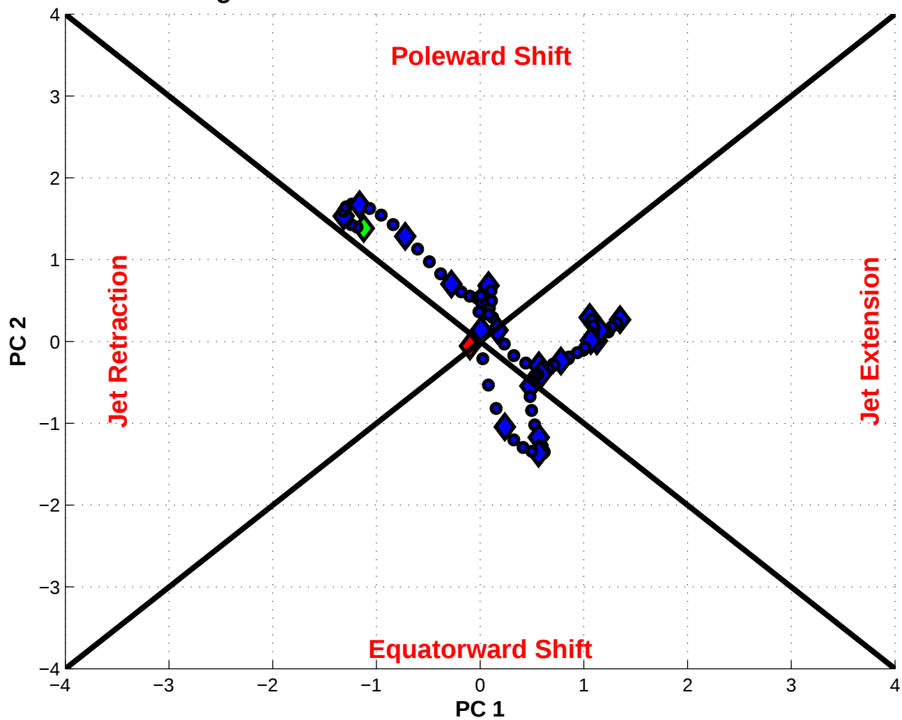
NPJ Phase Diagram valid 0600 UTC 09 Jan 2014 – 1200 UTC 30 Jan 2014
