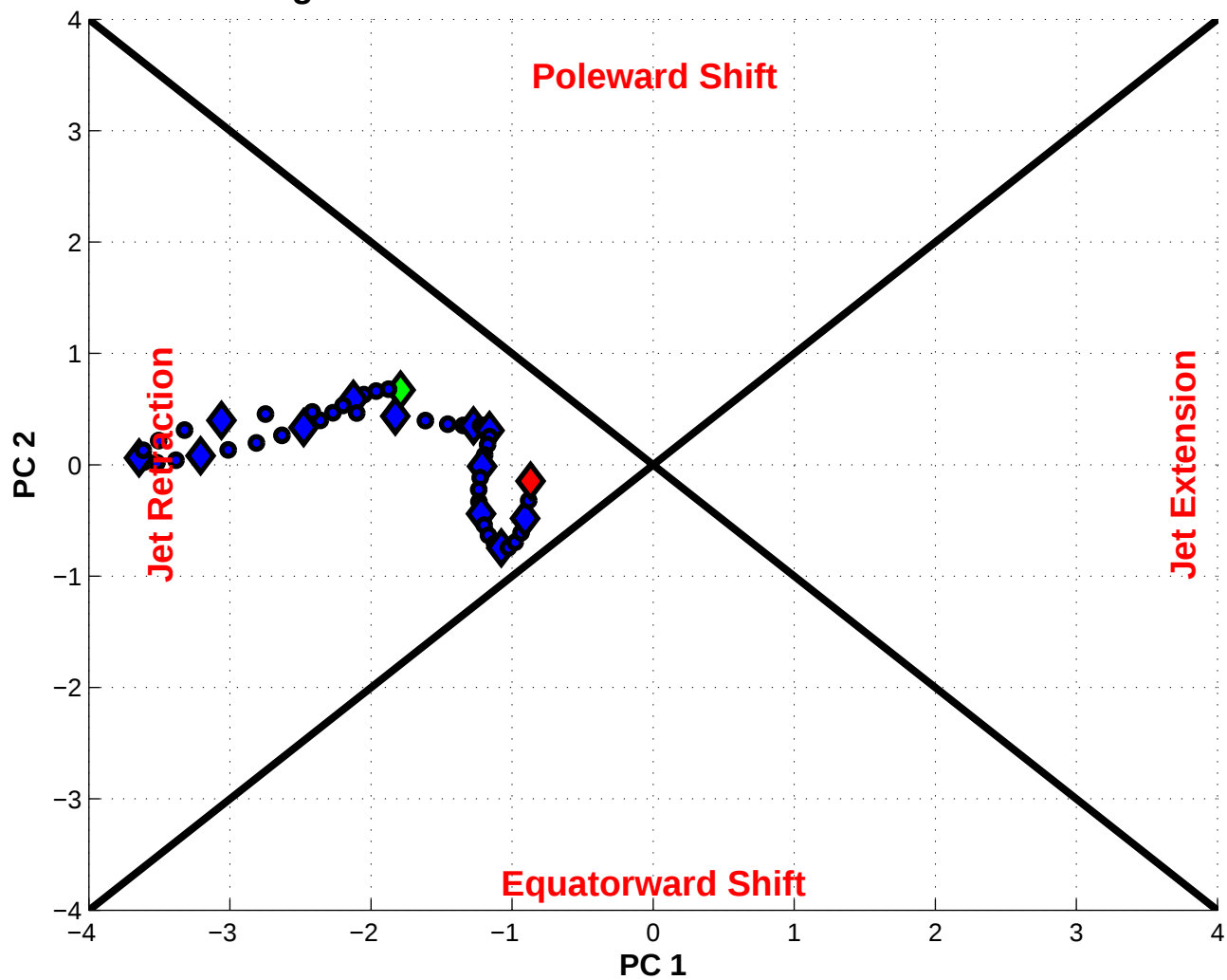
NPJ Phase Diagram valid 1800 UTC 09 Mar 2009 – 0600 UTC 22 Mar 2009
