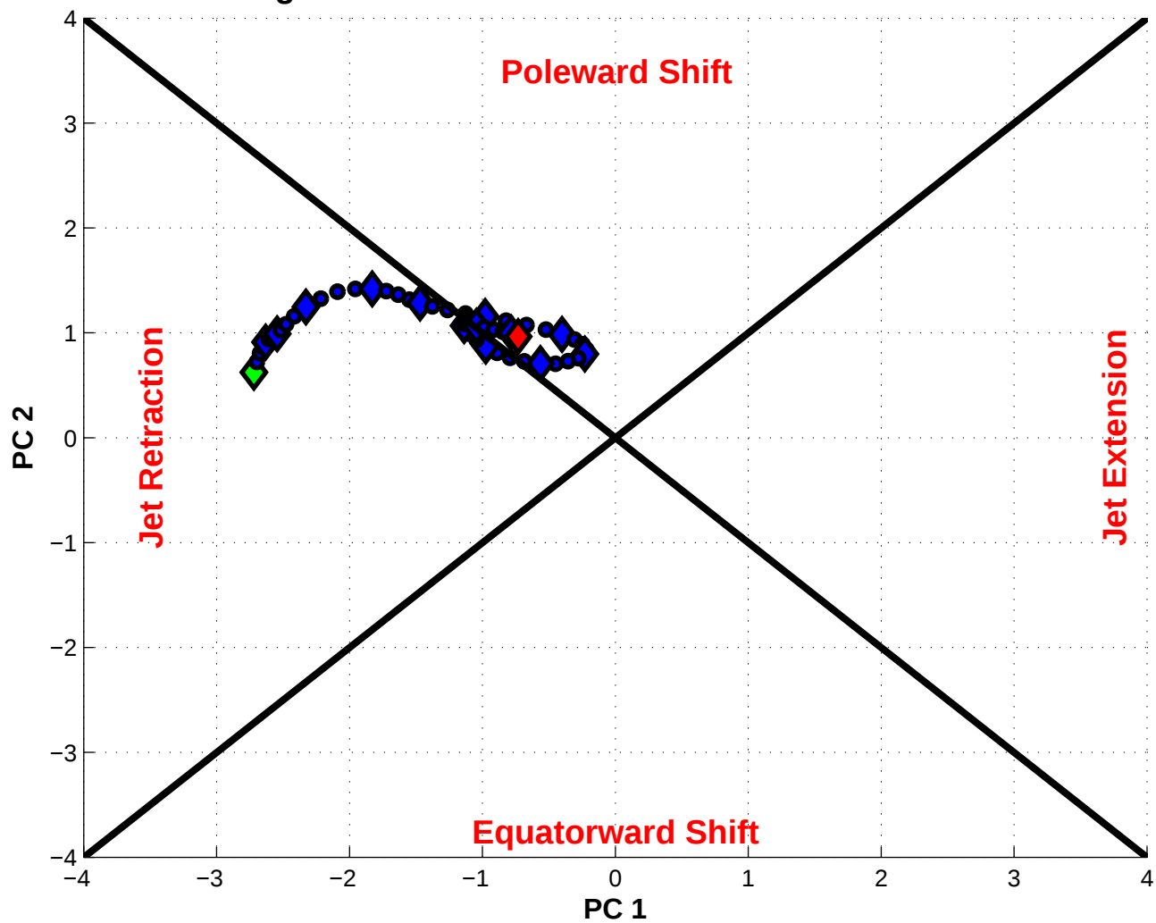
NPJ Phase Diagram valid 1200 UTC 10 Mar 1985 – 0000 UTC 24 Mar 1985
