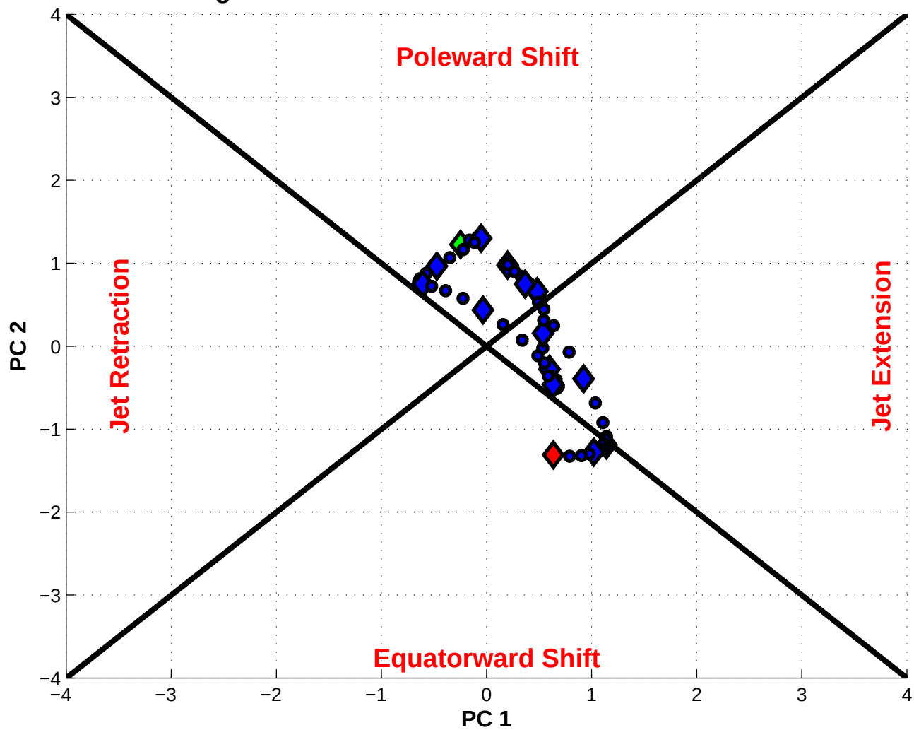
NPJ Phase Diagram valid 0000 UTC 10 Nov 1995 – 0000 UTC 24 Nov 1995
