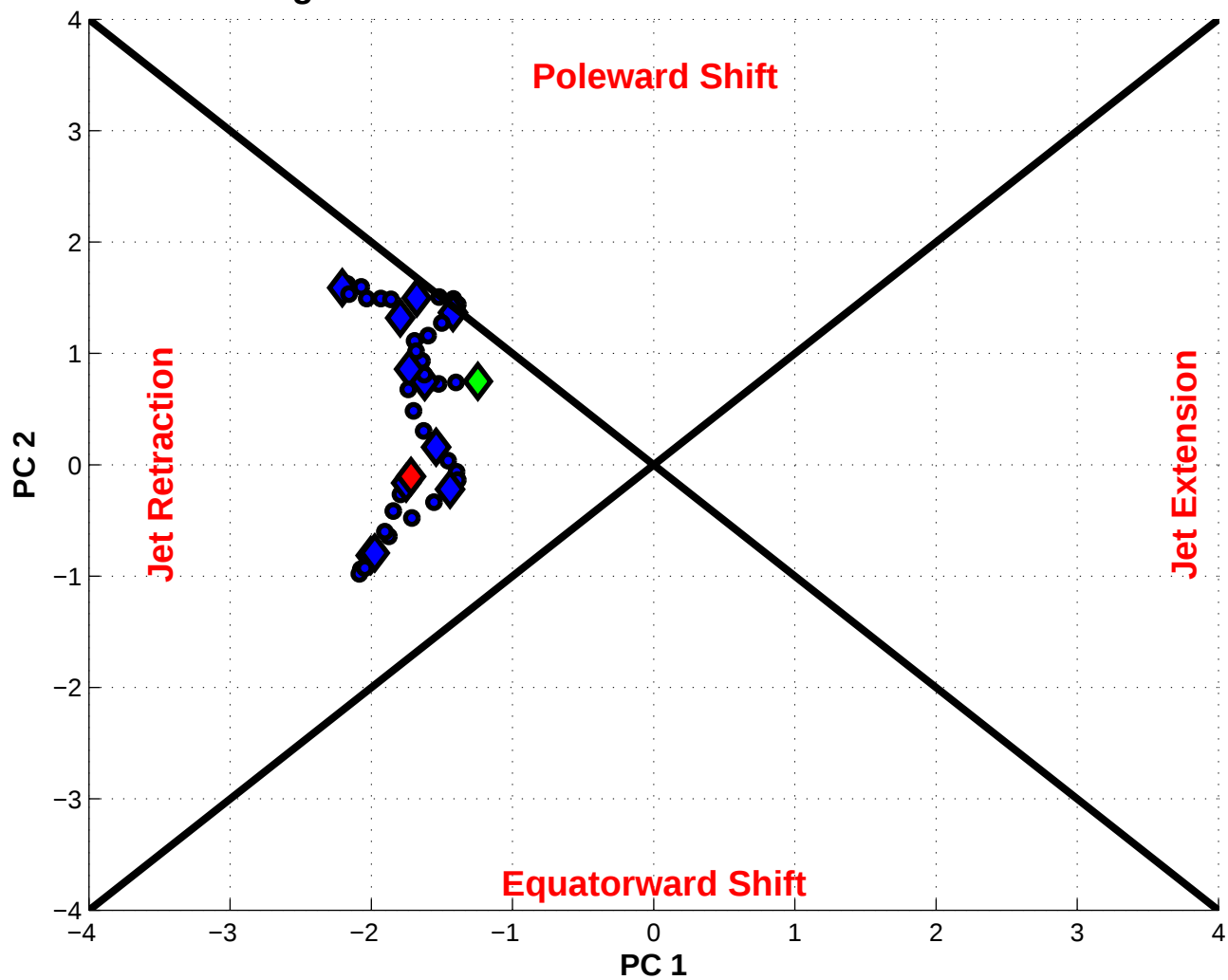
NPJ Phase Diagram valid 0000 UTC 11 Feb 2009 – 0600 UTC 22 Feb 2009
