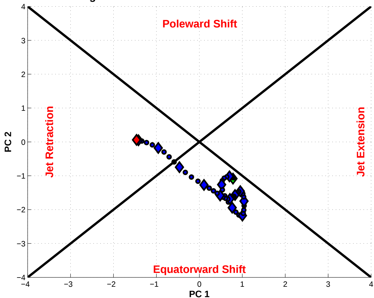
NPJ Phase Diagram valid 1800 UTC 12 Feb 2015 – 0600 UTC 26 Feb 2015
