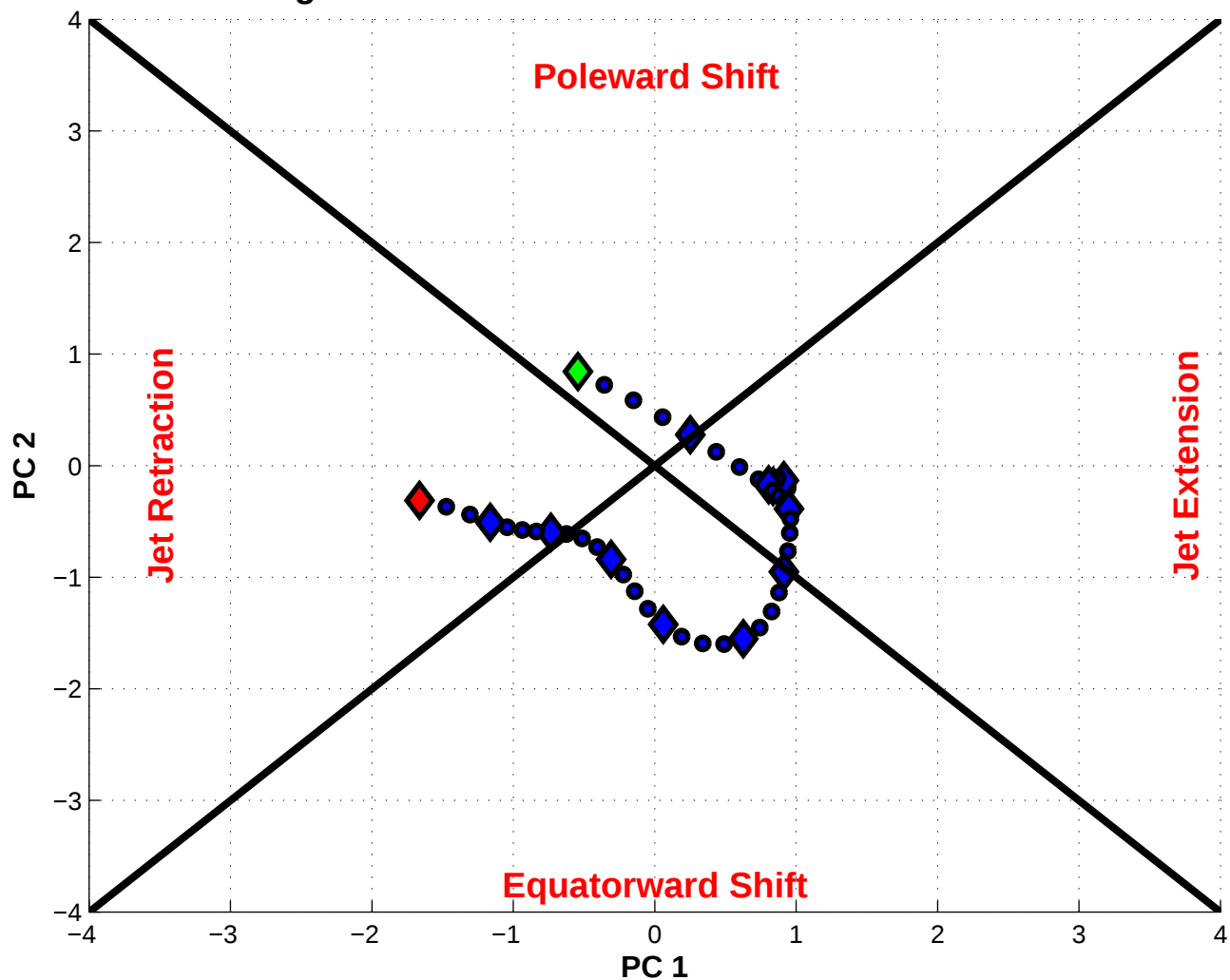
NPJ Phase Diagram valid 0000 UTC 12 Jan 2009 – 1800 UTC 23 Jan 2009
