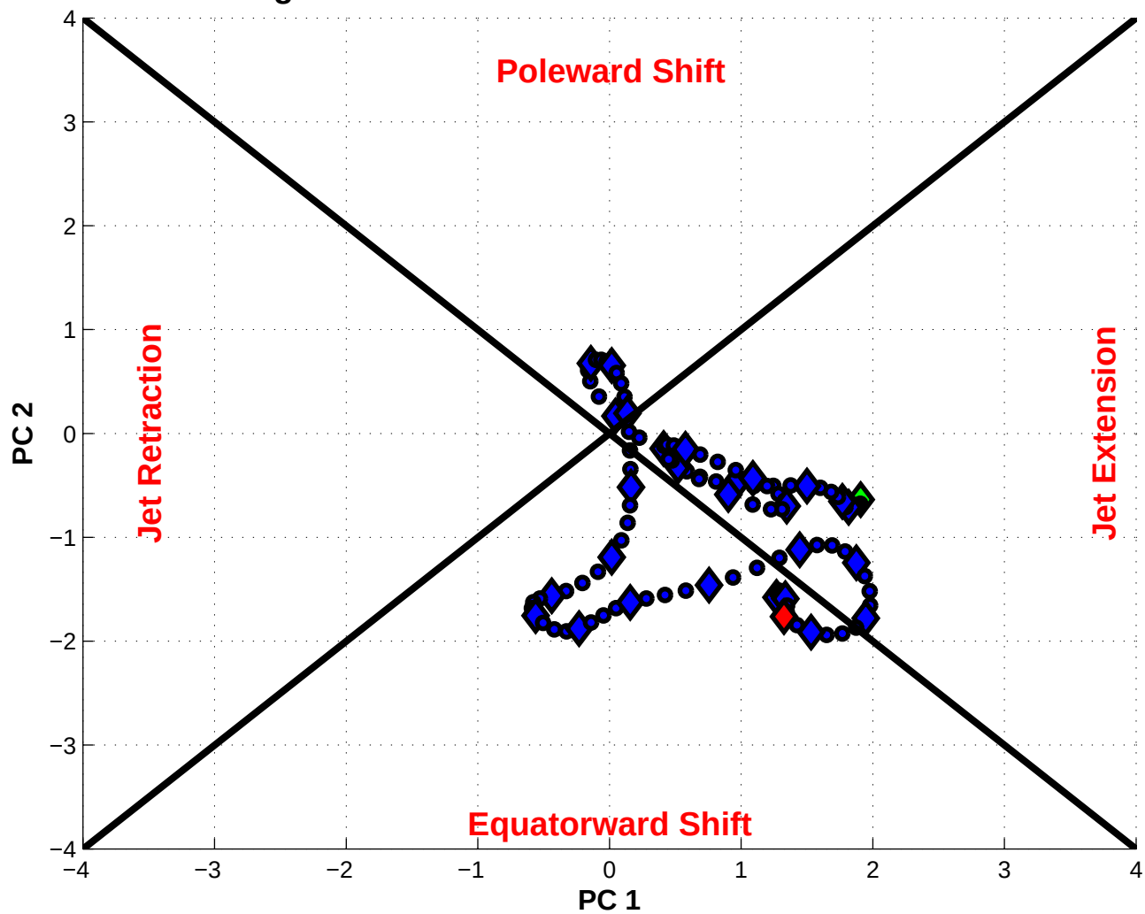
NPJ Phase Diagram valid 1200 UTC 12 Jan 2015 – 0600 UTC 09 Feb 2015
