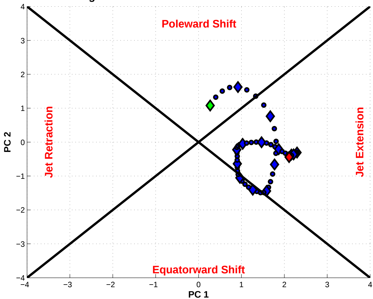
NPJ Phase Diagram valid 1200 UTC 13 Mar 2015 – 0000 UTC 28 Mar 2015
