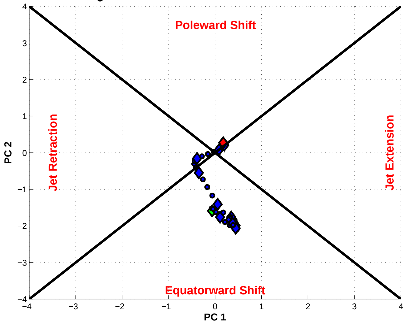
NPJ Phase Diagram valid 1800 UTC 14 Jan 2004 – 0600 UTC 25 Jan 2004
