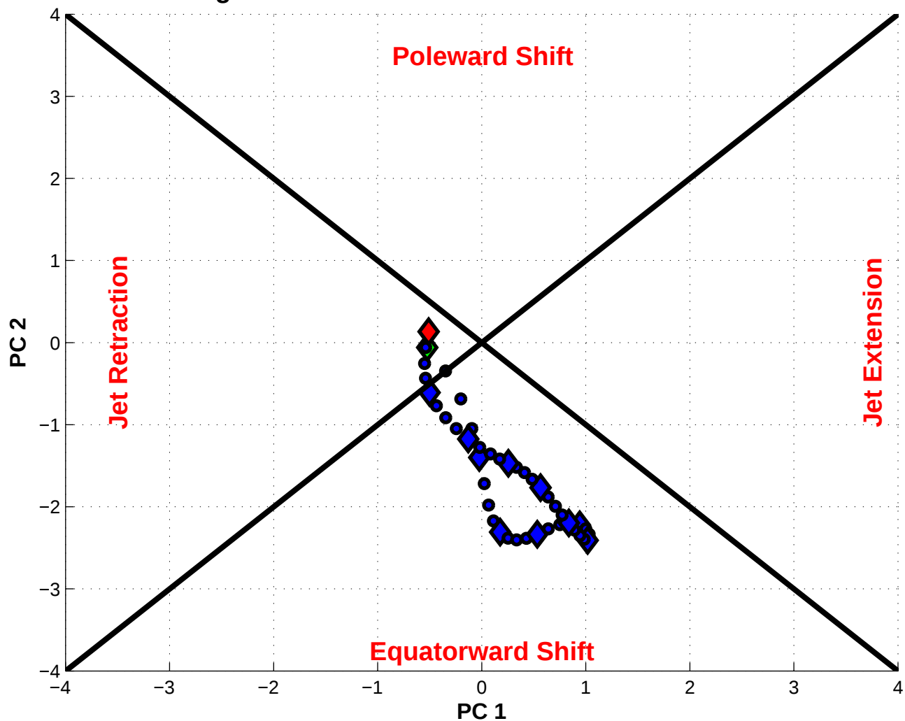
NPJ Phase Diagram valid 0000 UTC 16 Mar 2005 – 0000 UTC 27 Mar 2005
