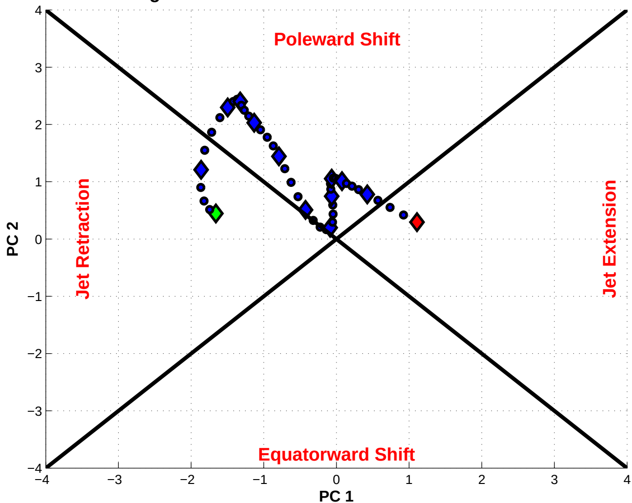
NPJ Phase Diagram valid 0000 UTC 18 Dec 2015 – 0000 UTC 30 Dec 2015
