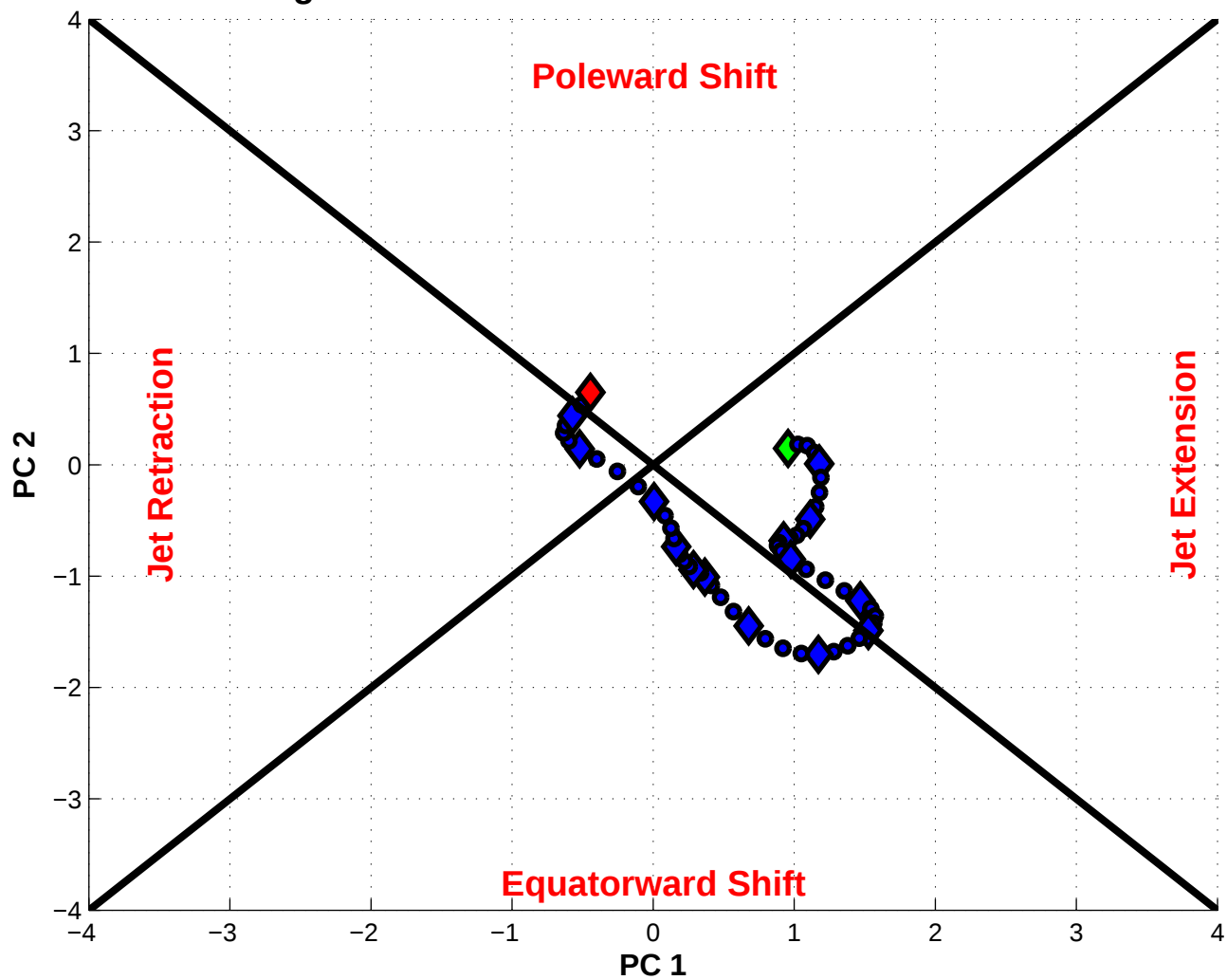
NPJ Phase Diagram valid 1800 UTC 18 Jan 2005 – 0600 UTC 02 Feb 2005
