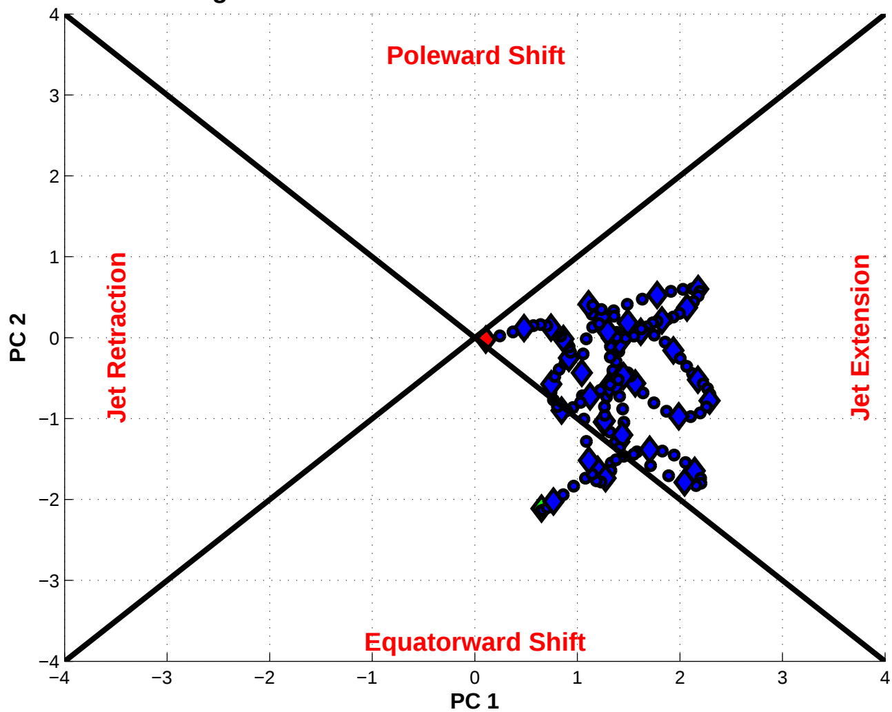
NPJ Phase Diagram valid 0000 UTC 19 Dec 1980 – 1800 UTC 26 Jan 1981
