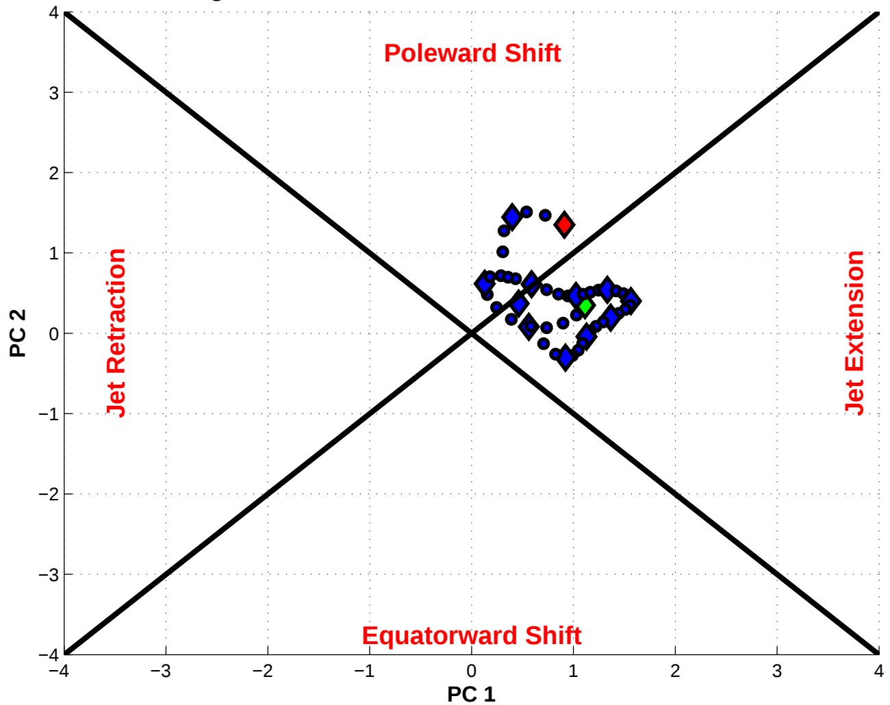
NPJ Phase Diagram valid 0000 UTC 19 Dec 1986 – 1800 UTC 30 Dec 1986
